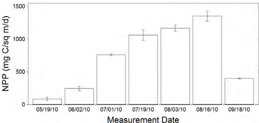
Figure 2. Net primary productivity of Oak Lake (Brookings County) in mg C•m -2 •d -1 during the summer of 2010 (mean +/- 1 standard error). Production measured to 16-cm depth.
