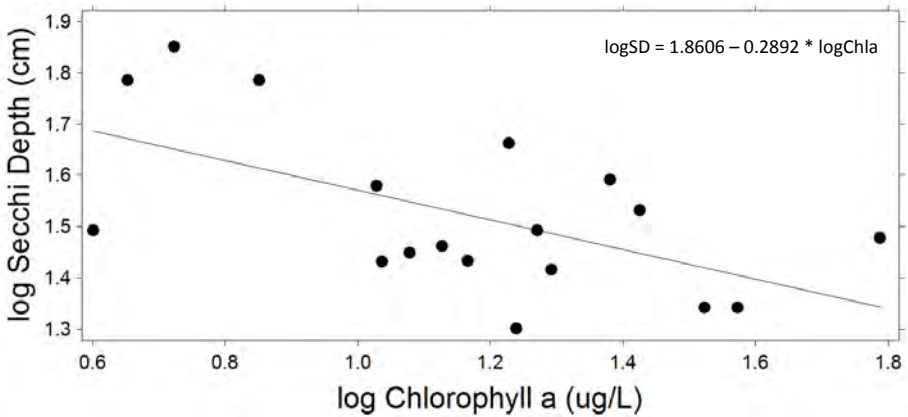
Figure 4. Relationship between Secchi depth (cm) and corrected chlorophyll a ( R^2 = 0.30 , P = 0.011 ) of Oak Lake during the 2010 growing season.
