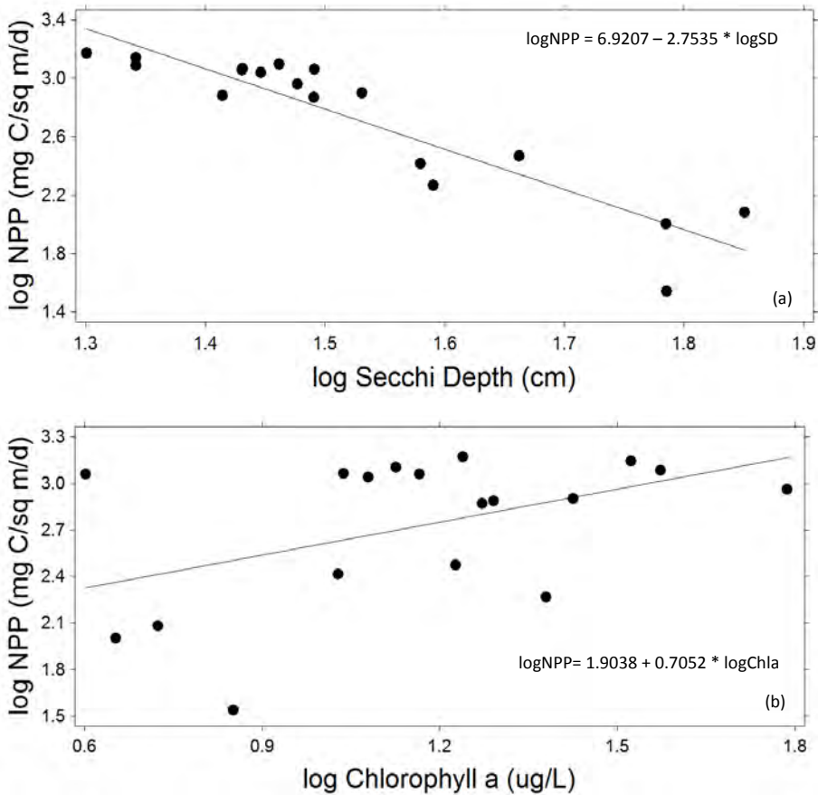
Figure 3. Relationships between net primary production of Oak Lake to 16-cm depth and (a) Secchi depth (cm) ( R^2 = 0.82 , P < 0.01 ) and (b) corrected chlorophyll a ( R^2 = 0.17 , P = 0.048 ) during the 2010 growing season.
