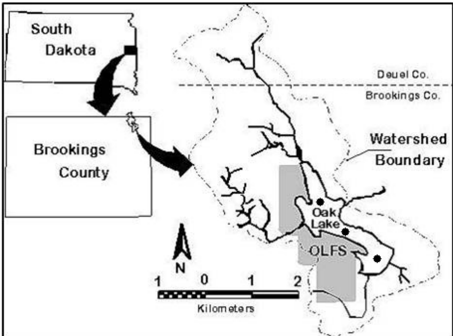
Figure 1. Basin monitoring sites within the Oak Lake basin (Brookings County) where light/dark productivity and monitoring measurements were taken.
