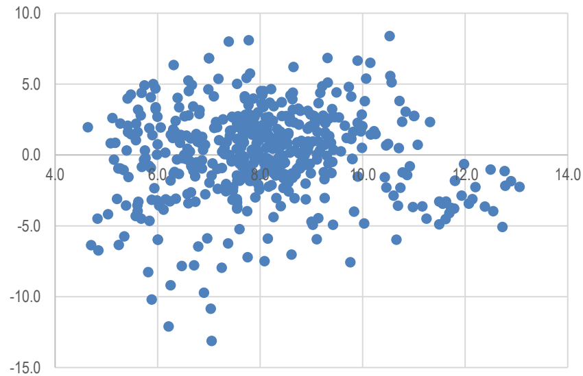
Figure 22: Residual plot for the linear regression model.
