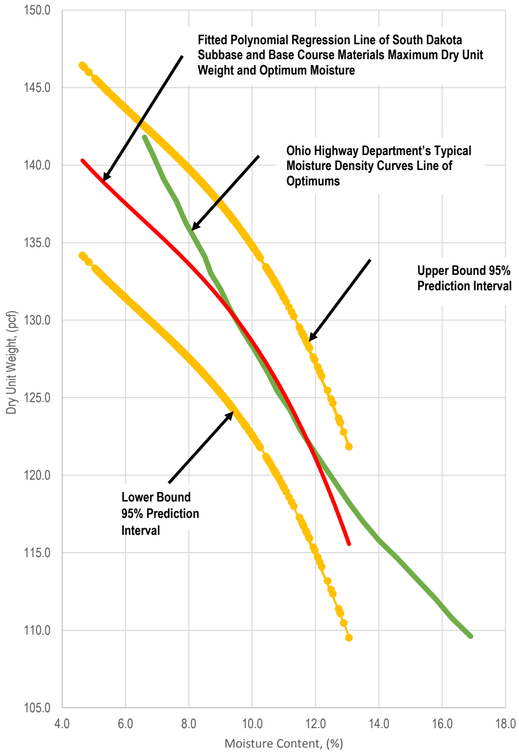
Figure 29: Line of optimums plotted within the 95 percent prediction interval.
