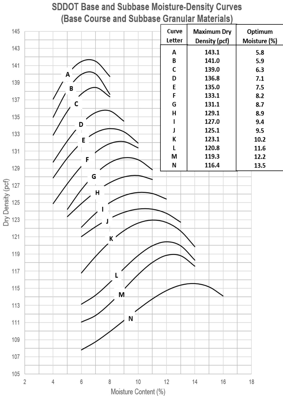
Figure 30. These curves were plotted with the regression model discussed in Chapter 3. The SDDOT Base and Subbase Moisture Density curves line of optimums shown in
