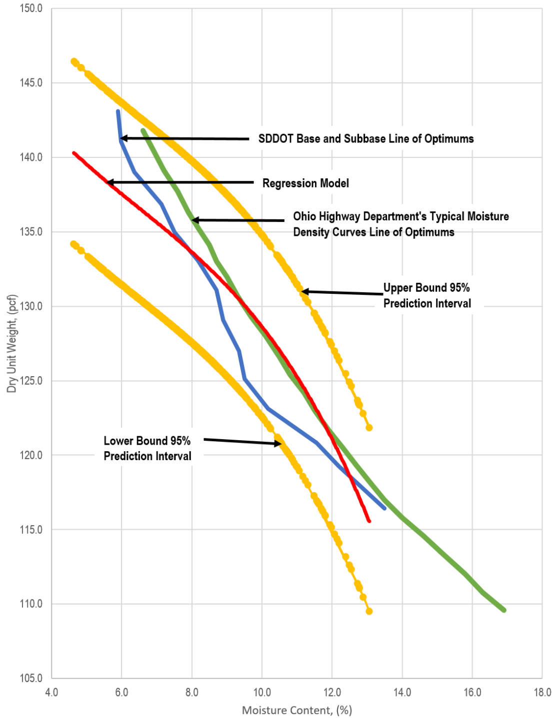
Figure 31: Lines of optimum comparison plotted within Prediction Interval.
