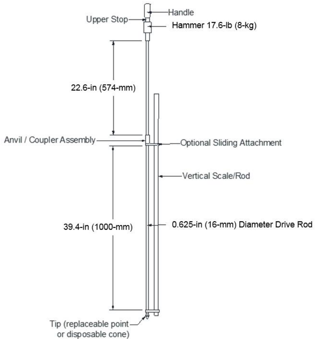
Figure 14: DCP schematic.
