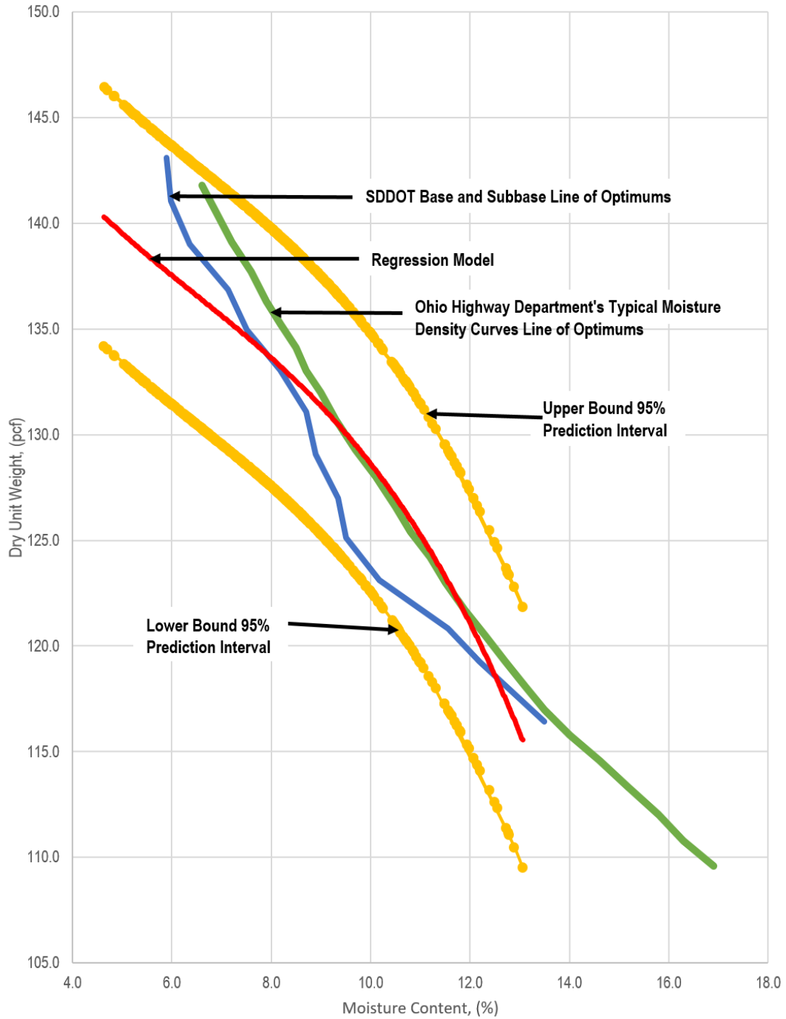
Figure 31 (combination of Figure 18 and Figure 28) in blue did slightly follow a more effective regression model than the previously plotted Ohio Highway Departments Typical Moisture Density Curves shown in green. Of particular note is that the new curves have been created from moisture density relations of granular materials encountered by the SDDOT thus making them a more desirable option. The new family
