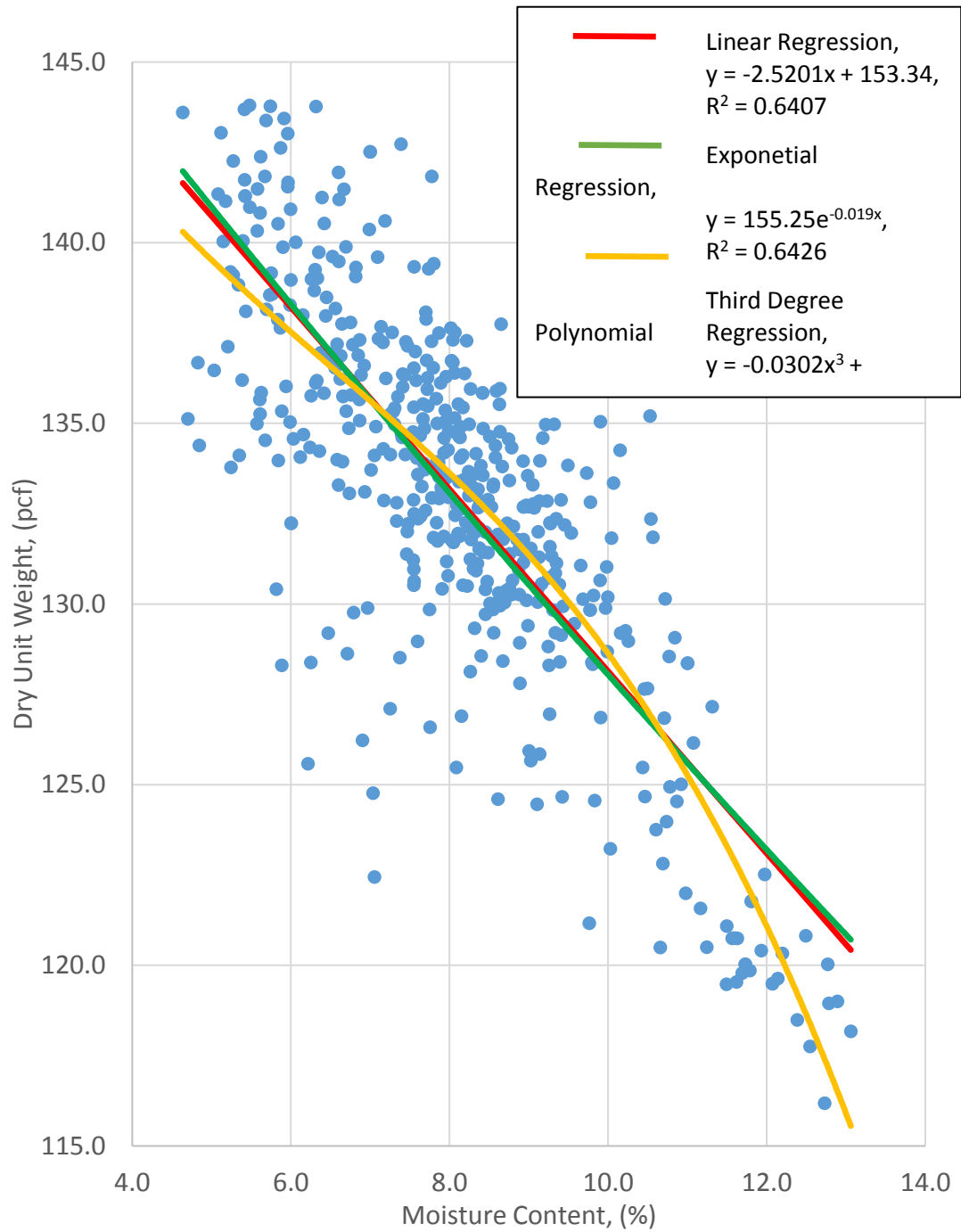
Figure 21: Fitted regression lines for granular moisture density relations.
