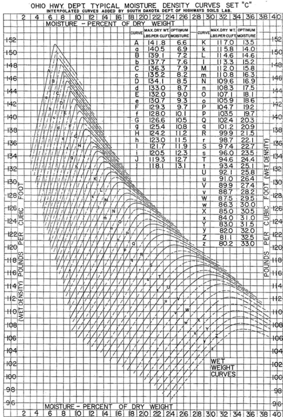
Figure 9: Ohio Highways Department's Typical Moisture Density Curves, Set C with interpolated curves (SDDOT, 2015a)
