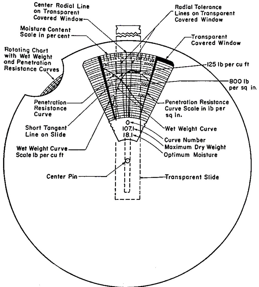
Figure 8: Typical Curve Circular Slide Rule (Joslin, 1958).
