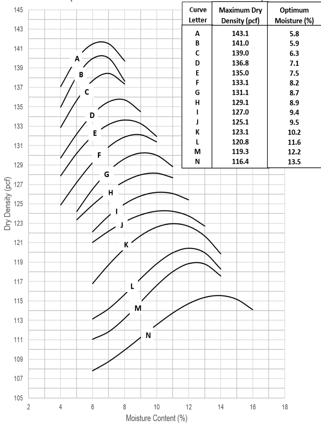
Figure 30: The SDDOT Base and Subbase Moisture Density Curves.
