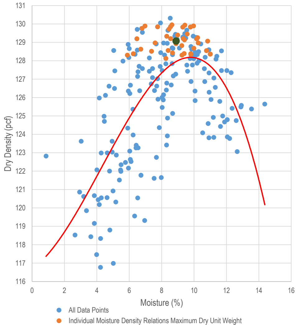
Figure 16: Observed skewed curve phenomenon.
