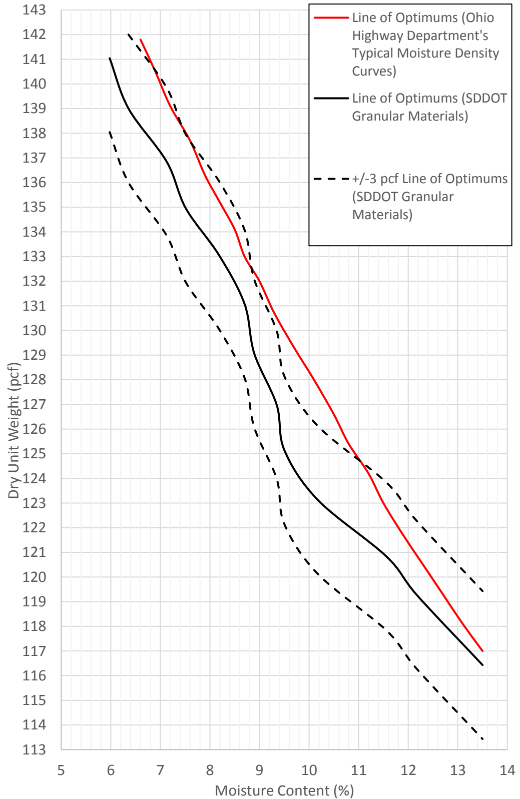
Figure 18: Lines of Optimums Used in Comparison Analysis.
