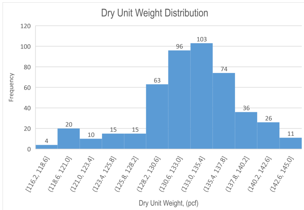
Figure 19: Dry Unit Weight Distribution
