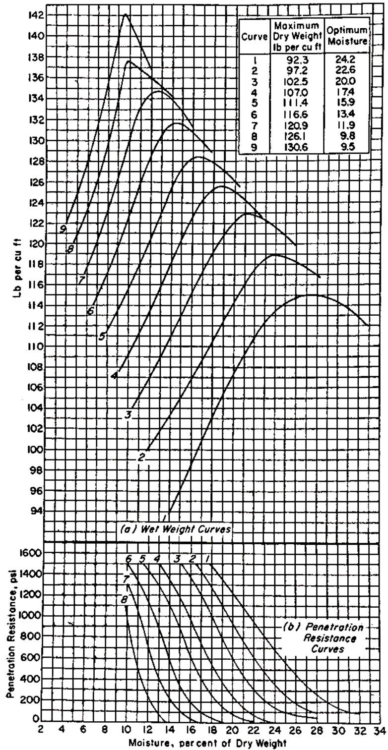
Figure 6: Typical embankment control curves, set A (Joslin, 1958).
