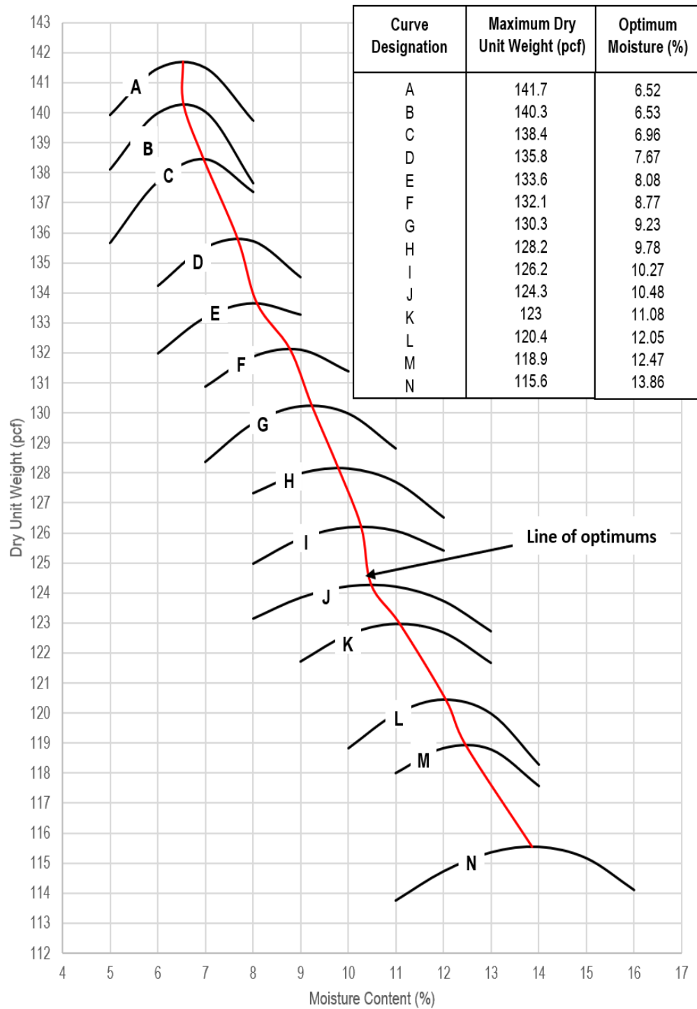
Figure 17: Line of optimums for new family of compaction curves (red line).
