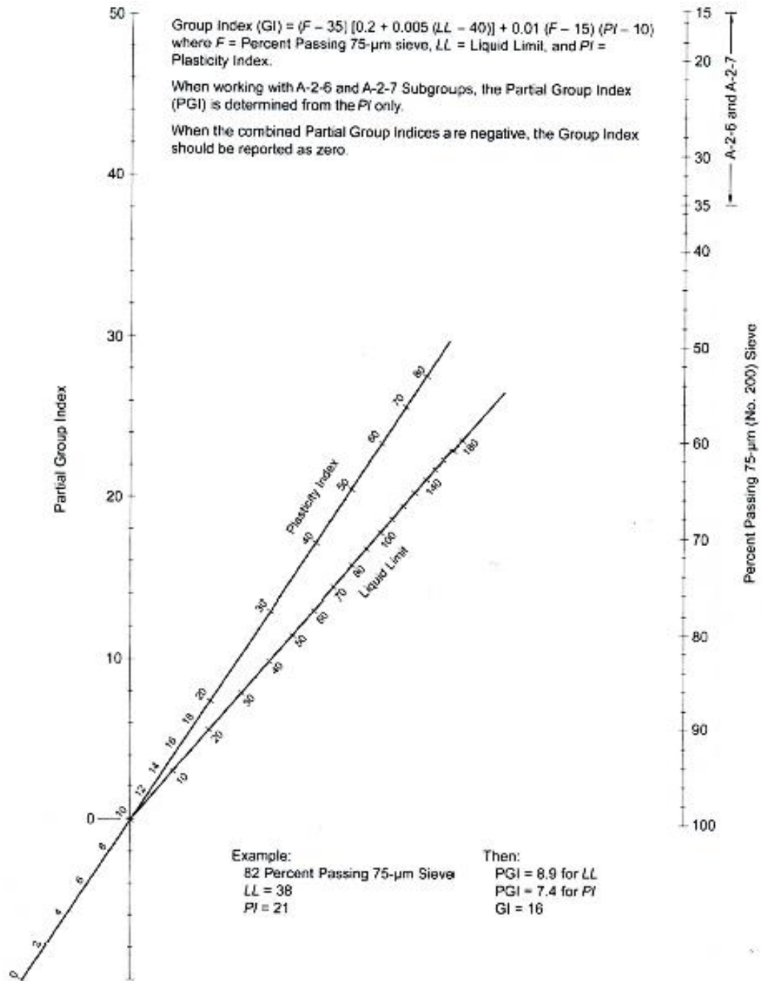
Figure 1: AASHTO M 145 Group Index Chart (AASHTO, 2015a).
