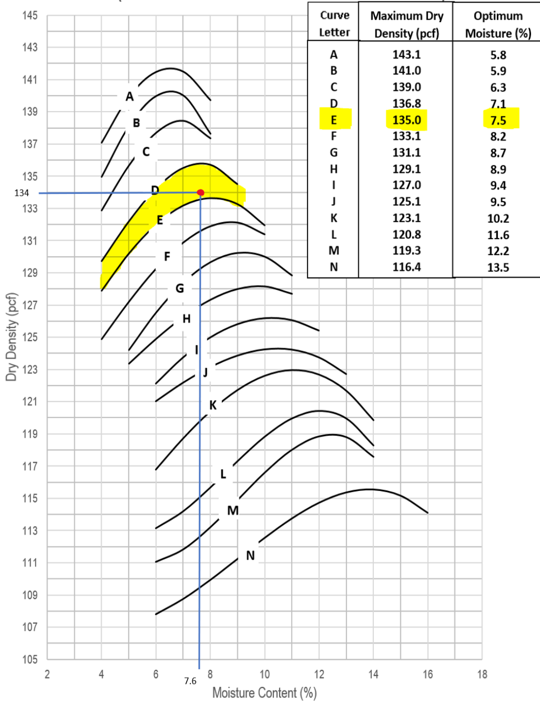
Figure 32: The plotted example using the SDDOT Moisture Density Curves.
