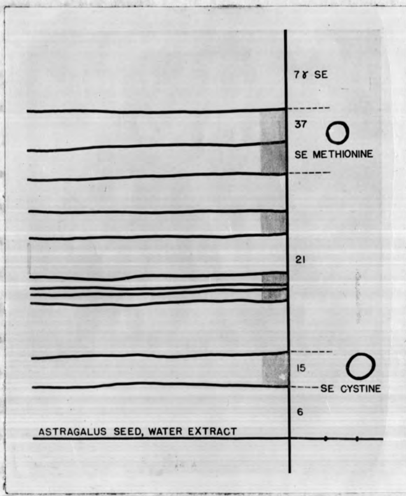
FIGURE V. A tracing of a portion of a phenol chromato- gram of a horizontal band of a water extract of Astragalus bisulcatus seed on the origin. The quantities of selenium found in the strips cut at the dotted lines are shown. The narrow shaded portions at the right show which horizontal strips are all colored.
