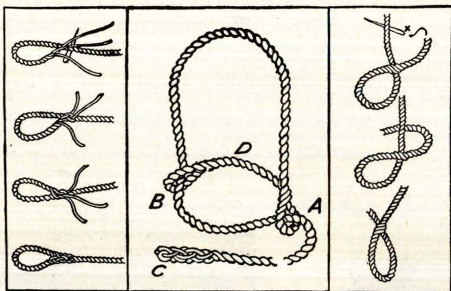
Steps in making eye splice B.
