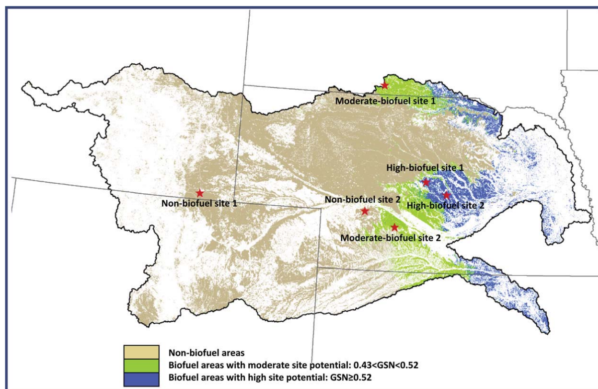
Fig. 2 – Grassland areas that are potentially suitable for cellulosic biofuel feedstock development (green and blue) within the GPRB identified by Gu et al. (2011). Pixels in green and blue represent areas that either overperformed or normally performed for seven of nine years from 2000 to 2008 and with moderate (the averaged GSN are 0.43–0.52) or high (the averaged GSN are greater than 0.52) ecosystem site potential. Grassland areas that are not suitable for biofuel feedstock development are in tan. Locations of the six representative sites are also shown in the figure (red stars).
