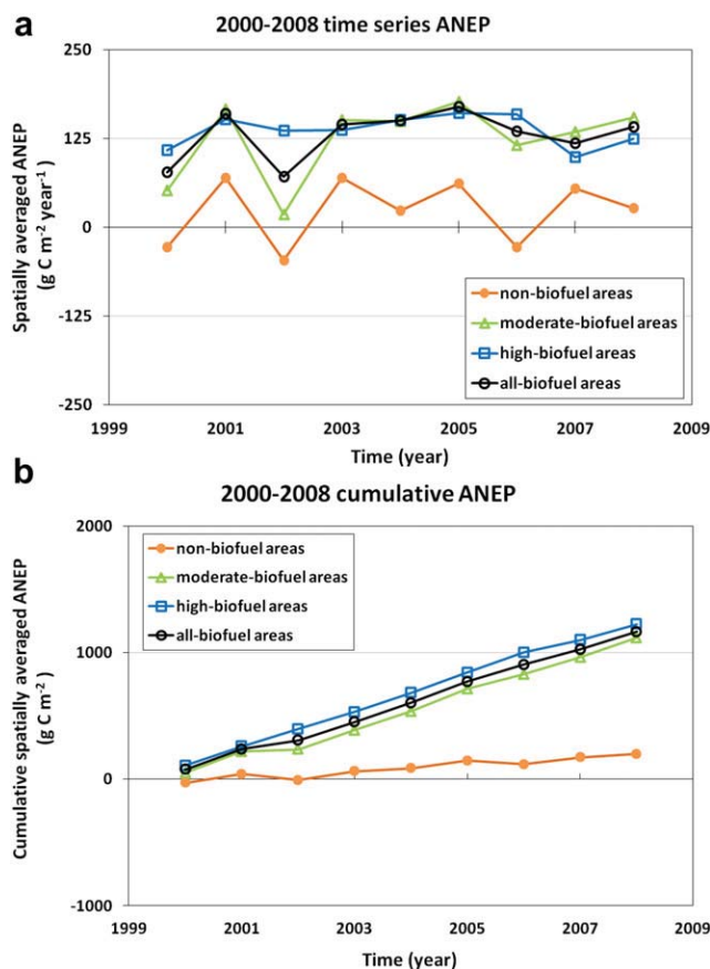
Fig. 4 – 2000–2008 Spatially averaged time series plots for the non-, the moderate-, the high-, and the all-biofuel grasslands. (a) Spatially averaged ANEP, (b) Cumulative spatially averaged ANEP.
