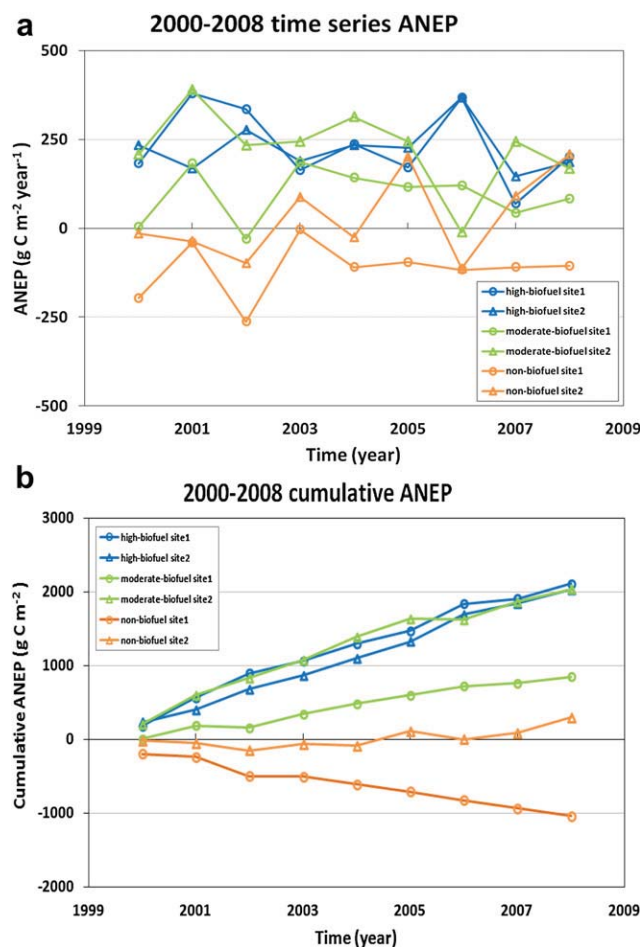
Fig. 3 – 2000–2008 Time series plots for the six representative sites. (a). ANEP, (b). Cumulative ANEP. Locations of the six sites are shown in Fig. 2 (red stars).
