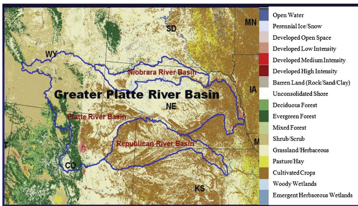
Fig. 1 – Location of the Greater Platte River Basin (inside the blue outline) and the land cover types as identified in the National Land Cover Database (NLCD). (For interpretation of the references to color in this figure legend, the reader is referred to the web version of this article.)
