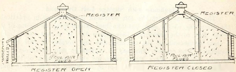
Fig. 10--Foul air flues may be used in the one-story hoghouse if registers are installed as shown. When there are enough hogs in the house, leave the register open so the foul air can go out at the ceiling as shown. With only a few hogs, it will be safe to close the register in very cold weather.
