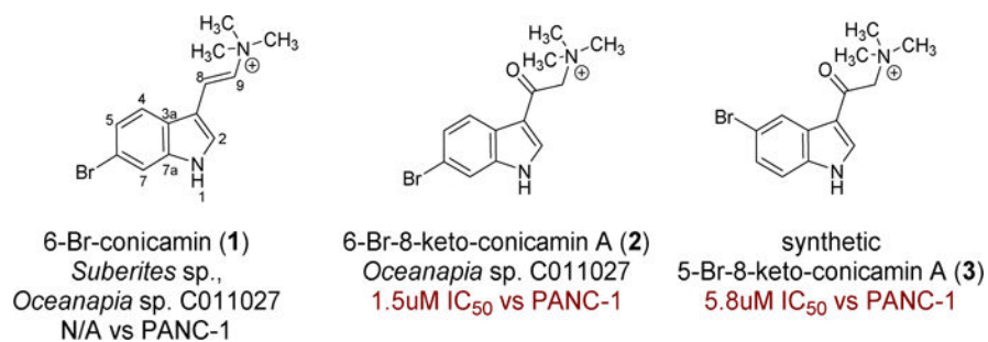
Fig. 1. The major products, 1 and 2 , isolated from Oceanapia sp. C011027 and the 5-Br synthetic analog 3 .
