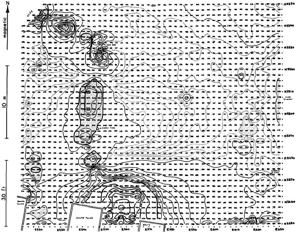
Figure 7. A magnetic map that covers the same area as Figure 6. While the predominant pattern is caused by the base of a former windmill and an iron pipe, there are also faint anomalies at the location of the cellar near the lower right corner of the map.
