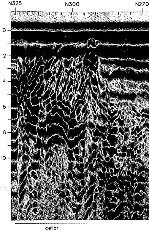
Figure 5. A ground-penetrating radar profile made at the Springfield Armory. My interpretation was that there might be a cellar shown on the right half of this profile; the cellar was actually on the left side. The length of the profile is 55 ft (17 m) and the bottom of the depth scale is 10 ft (3 m).
