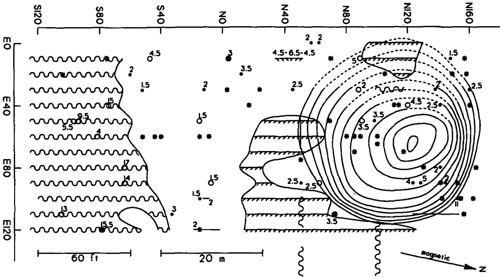
Figure 9. A basin-like soil feature at Valley Forge. This was found during a search for an earthen fort. The circular contours are at depth intervals of 0.5 ft (0.15 m) and range from 3 to 8 ft (1 to 2.4 m) deep.
