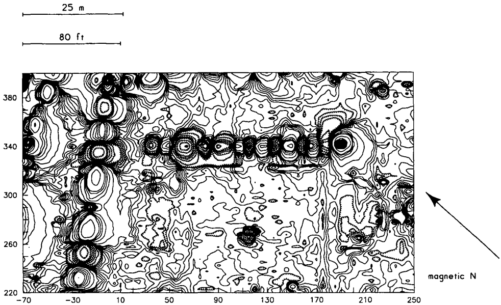
Figure 4. The magnetic effect of underground pipes at Fort Necessity. The bead-like patterns shown on this map are caused by four iron pipes. Magnetic lows are indicated with hachured contours.
