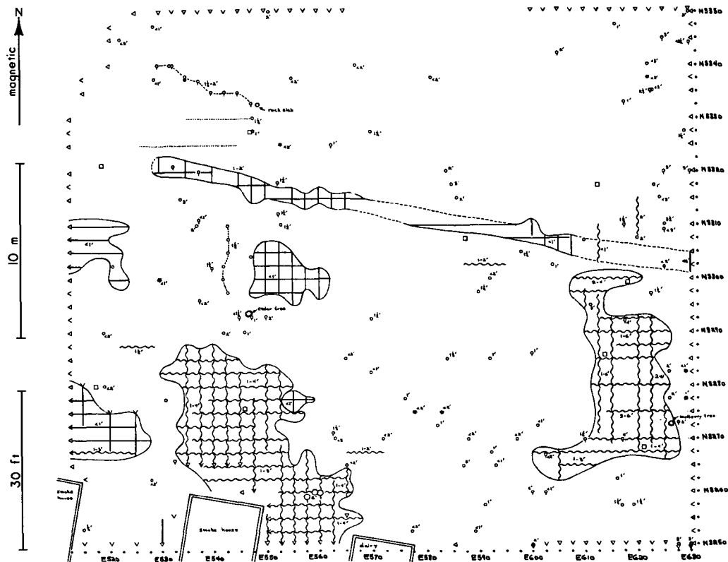
Figure 6. A radar echo map made at Appomattox Manor, Virginia. The cellar of an early building was found near the lower right corner of this area, where the radar detected distinctive echoes. Numbers in the map show the depth of the echoes, in feet; multiply these numbers by 0.3 to convert them to meters.
