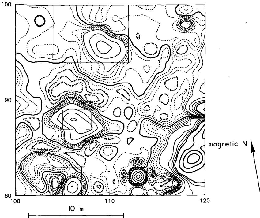
Figure 10. Jamestown Island. On the basis of this magnetic map, excavations were placed at the three rectangular areas shown here; kilns or concentrations of brick were found at each excavation.
