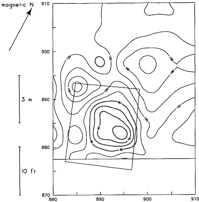
Figure 8. A map of electrical resistivity at Harpers Ferry. The low values coincide with the location of a shed which is seen on Sanborn maps from the years 1902 through 1933; it is marked with a rectangle.
