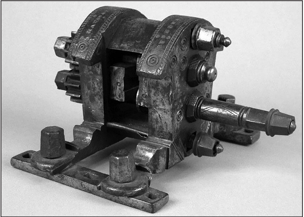
Figure 1. Glazier's vise, probably made by Edward White, in the collection of the Connecticut Historical Society. (Photo courtesy of Connecticut Historical Society, 2013.)
