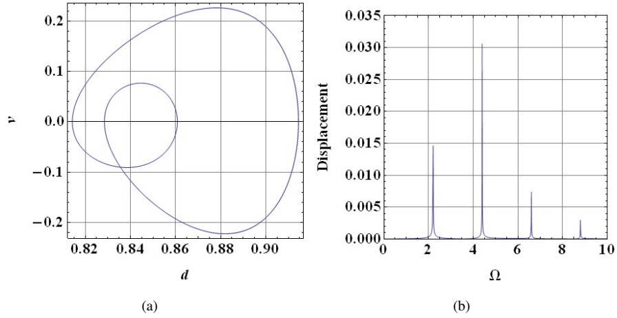
Fig. 7 The phase portrait (a) and the FFT (b) of an orbit at V_{AC} = 2 V and \Omega = 2.2 .
