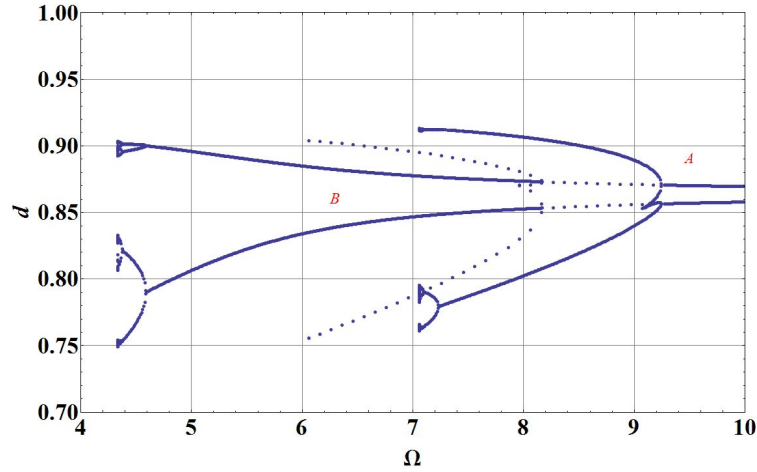
Fig. 4 The bifurcation diagram for the upper-well orbits at V_{AC} = 2 V.
