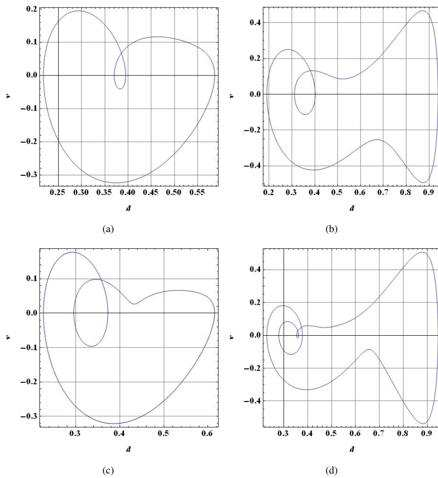
Fig. 27 The phase portraits of the superharmonic orbits of order (a) two \Omega = 0.87 , (b) three \Omega = 0.68 , (c) four \Omega = 0.58 , and (d) five \Omega = 0.44 at V_{AC} = 3.5 V.
