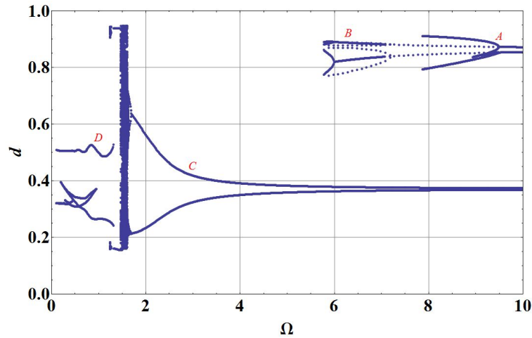
Fig. 12 The bifurcation diagram for V_{AC} = 3 V.
