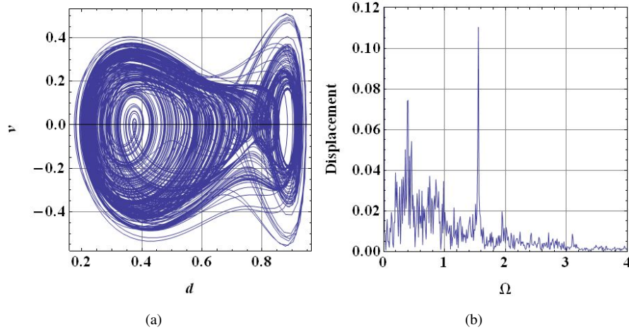
Fig. 16 The phase portrait (a) and the FFT (b) of a fully developed chaotic attractor at \Omega = 1.55 and V_{AC} = 3 V.
