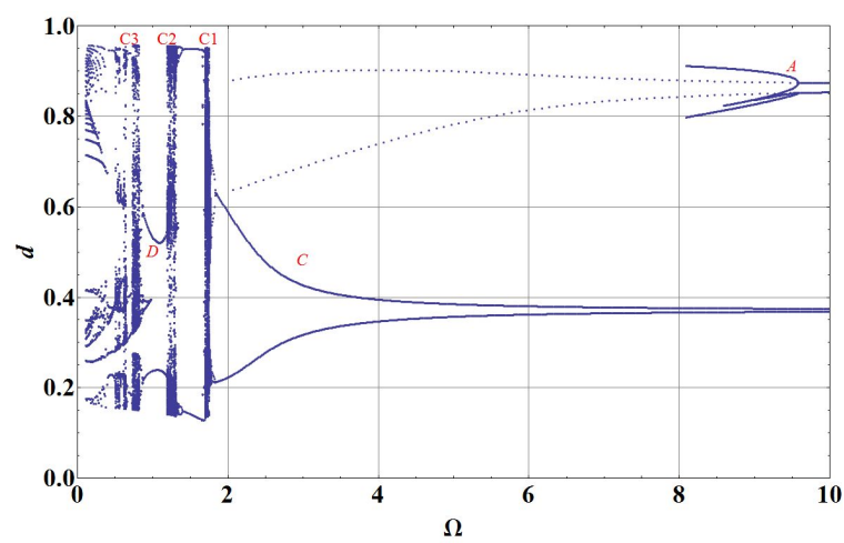
Fig. 21 The bifurcation diagram for V_{AC} = 3.5 V.
