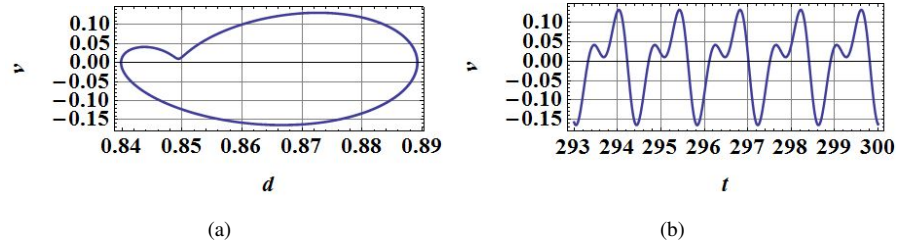
Fig. 5 The phase portrait (a) and the time-history of the beam tip velocity (b) for a period-two orbit at V_{AC} = 2 V and \Omega = 9 .
