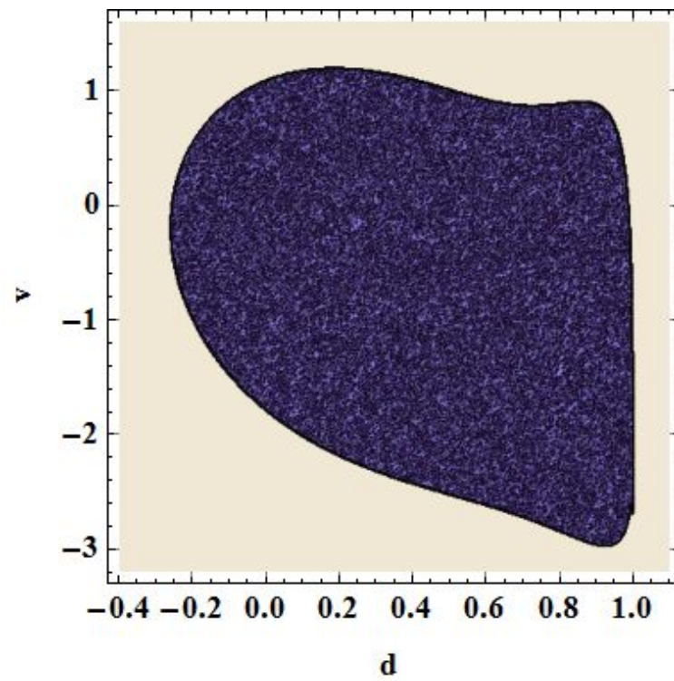
Fig. 30 The basin of attraction of a chaotic attractor at V_{AC} = 3 V and \Omega = 1.62 .
