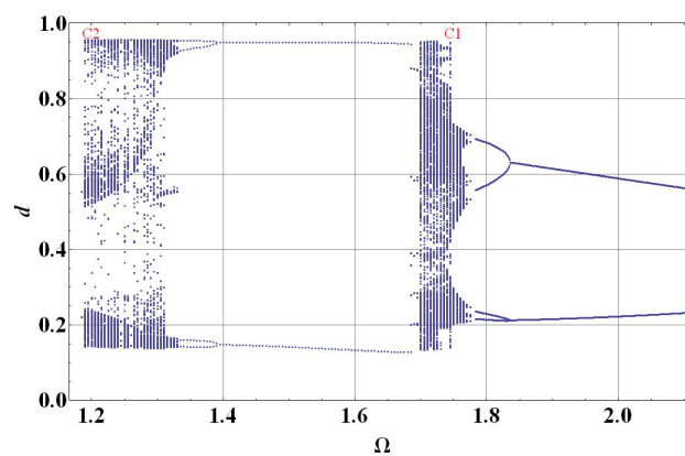
Fig. 22 Bifurcation diagram for the chaotic regions at V_{AC} = 3.5 V.
