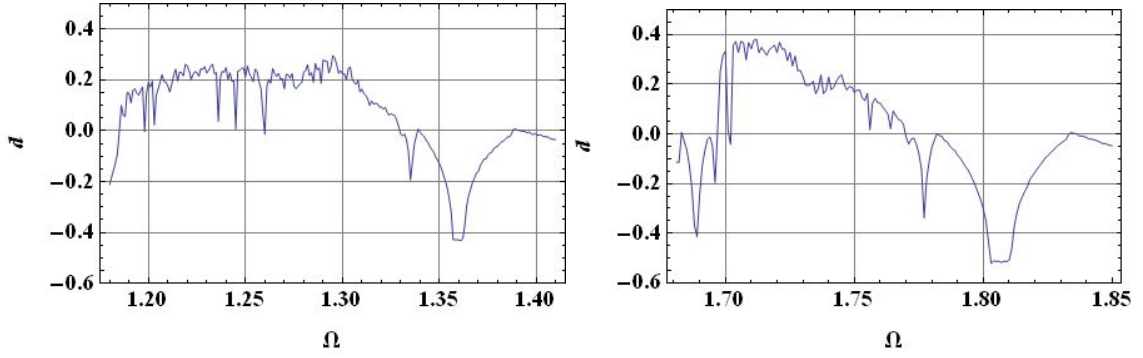
Fig. 23 The maximum Lyapunov exponent of the chaotic attractors at V_{AC} = 3.5 V.
