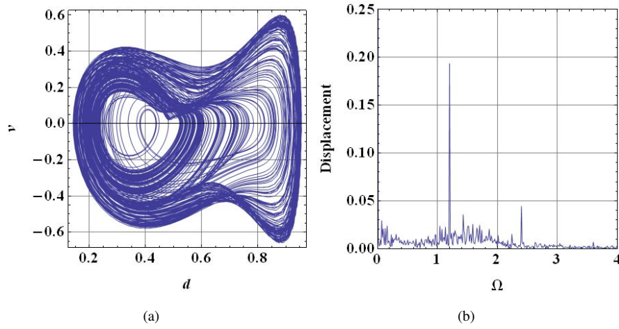
Fig. 24 The phase portrait (a) and the FFT (b) of a two-well chaotic attractor at V_{AC} = 3.5 V and \Omega = 1.2 .
