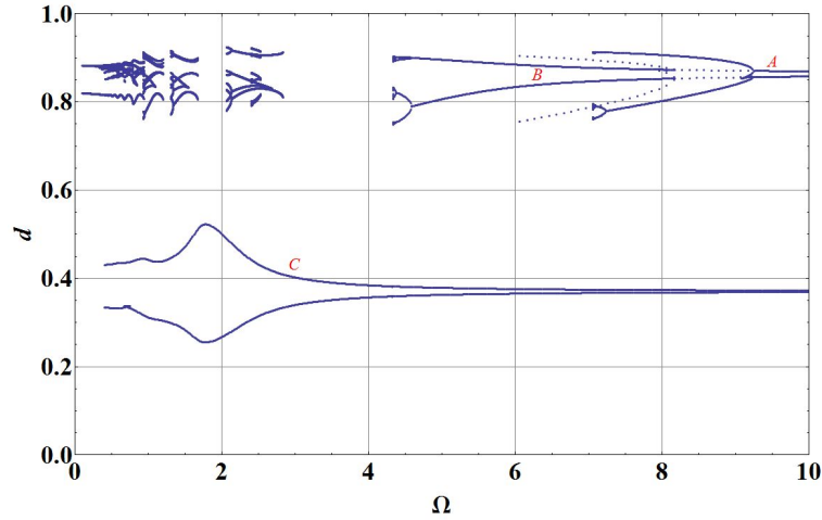
Fig. 3 The bifurcation diagram for V_{AC} = 2 V.
