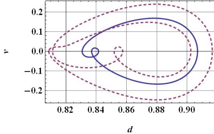
Fig. 8 The phase portraits of the coexisting orbits at V_{AC} = 2 V and \Omega = 2.5 .
