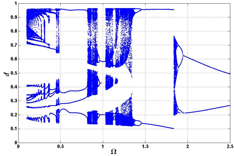
Fig. 28 The bifurcation diagram for the chaotic regions at V_{AC} = 4 V.
