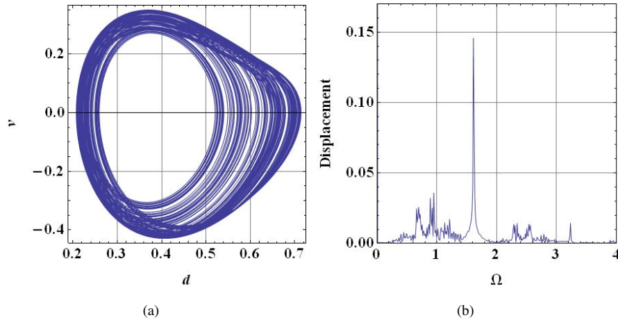
Fig. 15 The phase portrait (a) and the FFT (b) of a banded chaotic attractor at V_{AC} = 3 V and \Omega = 1.615 .
