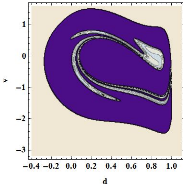
Fig. 29 The basin of attraction of the orbits at V_{AC} = 2 V and \Omega = 7.5 .
