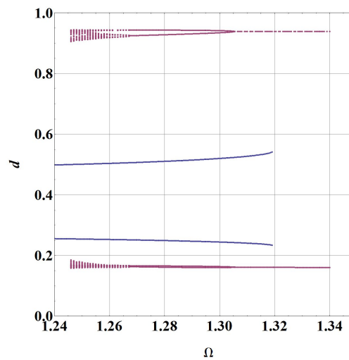
Fig. 19 The coexistence of two-well branch of orbits and chaos with a stable one-well periodic orbit.
