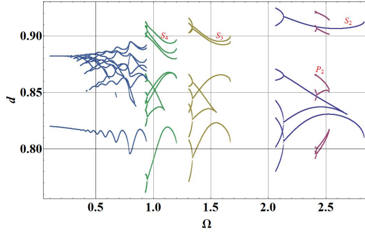
Fig. 6 Bifurcation diagram of the superharmonic orbits in the upper-well at V_{AC} = 2 V.
