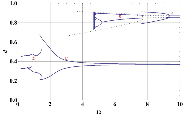
Fig. 9 The bifurcation diagram for V_{AC} = 2.5 V.
