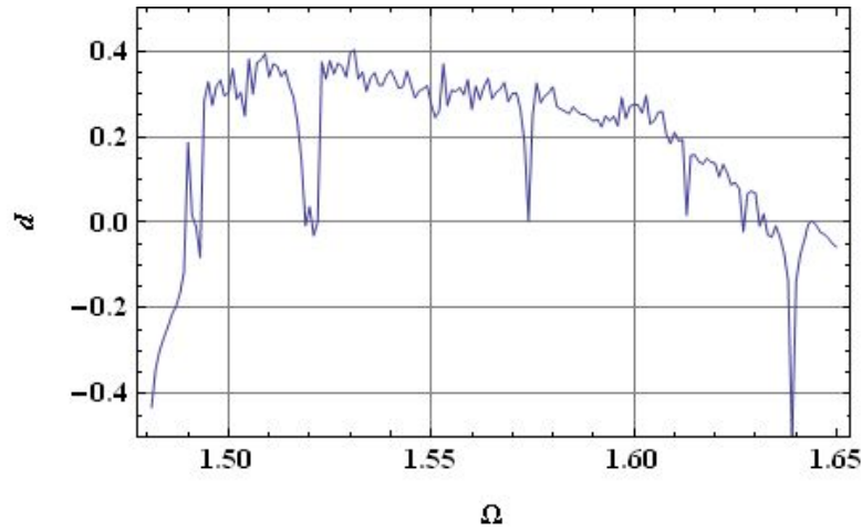
Fig. 14 The maximum Lyapunov exponent of the chaotic attractors at V_{AC} = 3 V.
