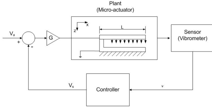
Fig. 2 Block diagram of the close-loop system.
