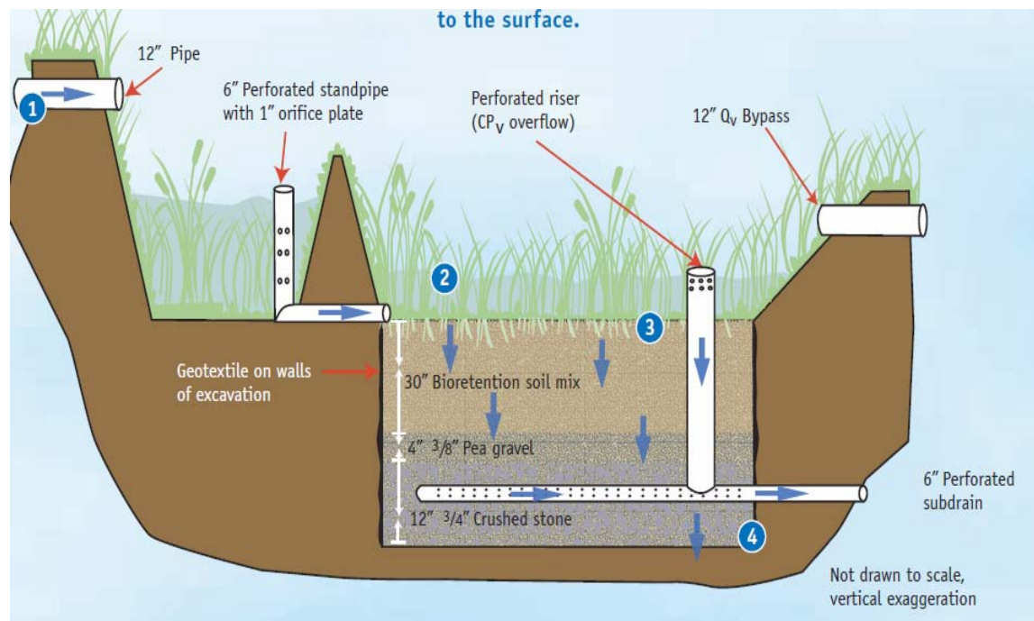
Figure 1. Bioretention Schematic
