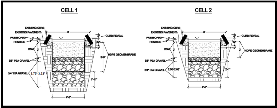
Figure 13. Cross-Section of Durham Bio-5 Bioretention Cells.
