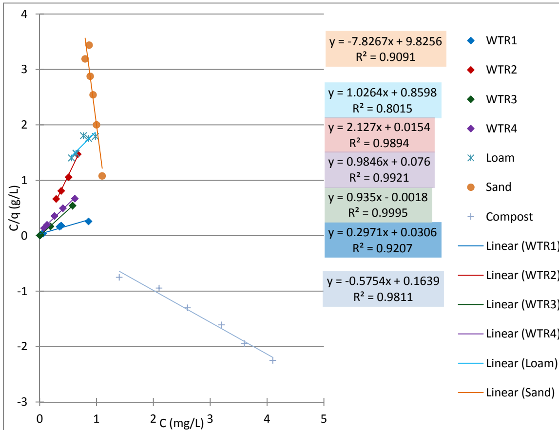
Figure 19. Langmuir Isotherm Model for Constituents
