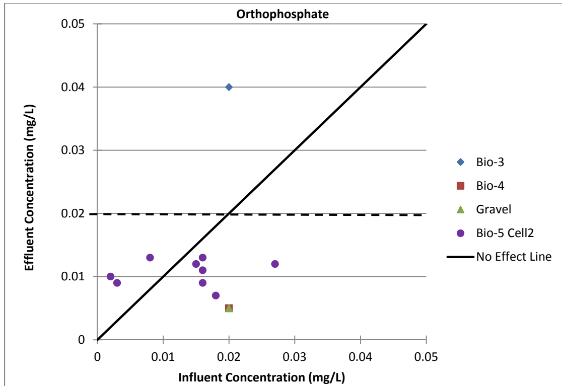
Figure 36. Treatment Effect Plot on OP for 4 UNH systems.
