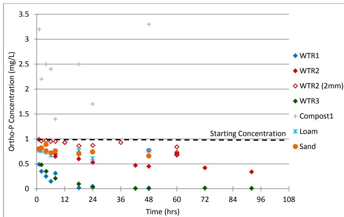
Figure 16. Kinetics Study Results.
