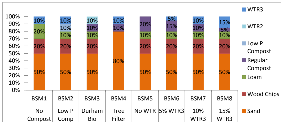
Figure 14. BSM Composition on a volume basis
