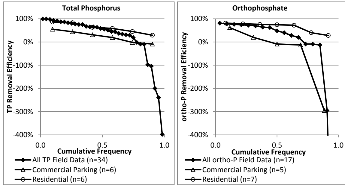
(a) (b) Figure 6. Cumulative Frequency Functions of Total Phosphorus and Orthophosphate Removal Efficiencies in the SPU Bioretention Database.
