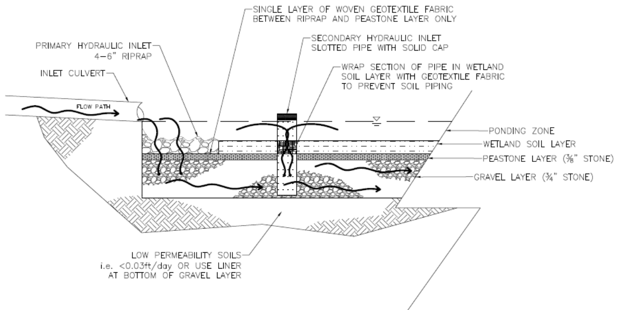
Figure 2: Modification of hydraulic inlet to subsurface gravel layer. Hydraulic Outlet Configuration
