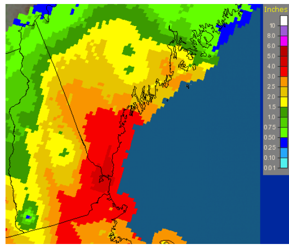
FIGURE 3.2: 24-hour rainfall totals for April 16, 2007. (Image source: NOAA-NWS Advanced Hydrologic Prediction Service).
