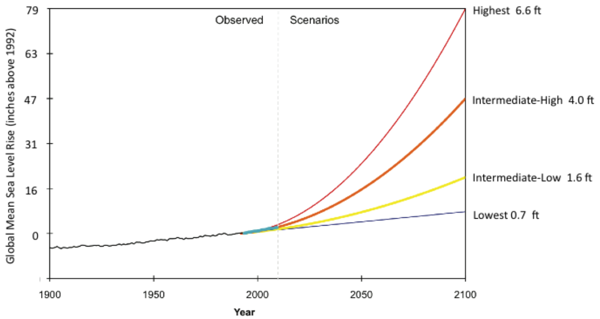
FIGURE 2.7. Global mean sea-level-rise scenarios from 1992 from the U.S. National Climate Assessment. Figure from Parris et al., 2012
