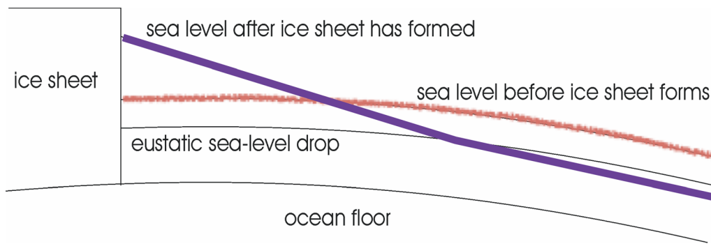
FIGURE 2.2. Schematic of the self-gravitation effect. The ocean is pulled toward the mass of an ice sheet, which raises sea level locally. A reduction in the ice-sheet mass causes a local lowering of sea level although sea level is raised significantly away from the ice sheet.
