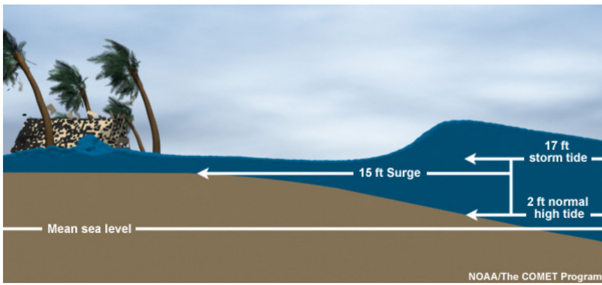
FIGURE 3.1. Storm Tide Components. Figure from endnote reference 49.
