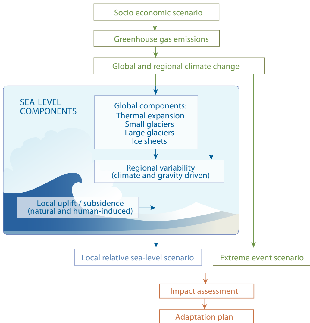
FIGURE 4.1. Conceptual model used to provide guidance regarding future sea-level rise for New Hampshire. Modified from Nicholls et al. (2014).
