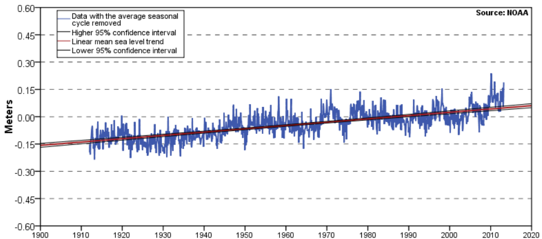
FIGURE 2.5. Mean sea-level trends from Portland, Maine; Seavey Island (Portsmouth Naval Shipyard), Maine; and Boston, Massachusetts, based on observed monthly mean sea-level data from NOAA tide gauges (NOAA, 2014).
