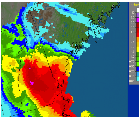
FIGURE 3.1: 24-hour rainfall totals for May 14, 2006. (Image source: NOAA-NWS Advanced Hydrologic Prediction Service).
