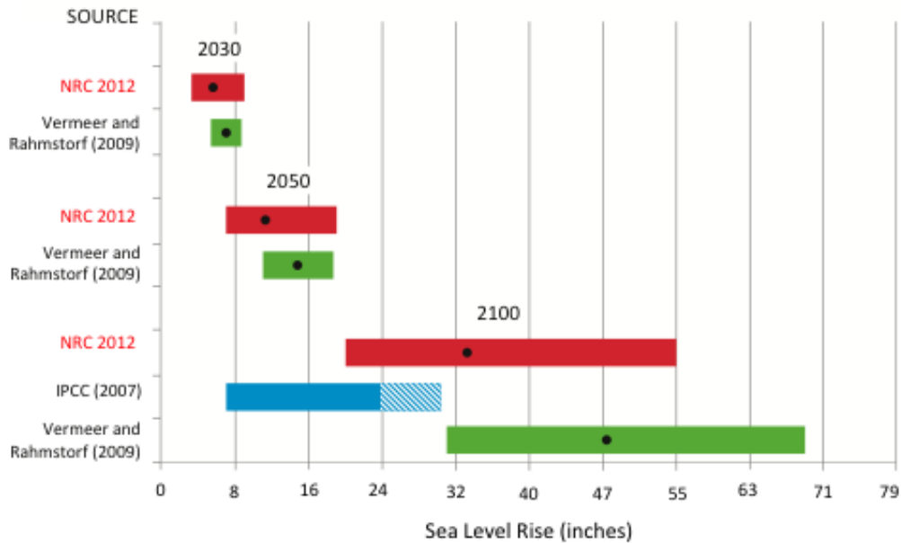
FIGURE 2.6. Global sea-level rise for 2030, 2050, and 2100 projected by the National Research Council (2012), in red; by Vermeer and Rahmstorf (2009), in green; and by the Intergovernmental Panel on Climate Change (2007), in blue. The dots are the projected mean values and the colored bars represent the range. The Intergovernmental Panel on Climate Change value includes the sea-level projection (blue) plus a scaled-up ice sheet discharge component (blue diagonal lines). Figure modified from National Research Council, 2012.
