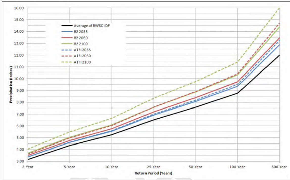
Observed and Forecasted 24-hour Rainfall for Medium (B2) and Precautionary (A1FI) Scenarios for 2035, 2060 and 2100 with Return Periods of 2 to 500 Years
