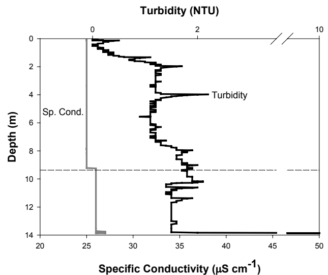
Fig. 4: Vertical profiles of turbidity and specific conductivity for Christine Lake on September 26, 2003. Thermocline is represented by the dashed line.
