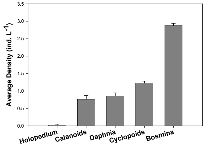
Fig. 10: Average density ( \pm 1 SE) of zooplankton in Christine Lake on September 26, 2003
