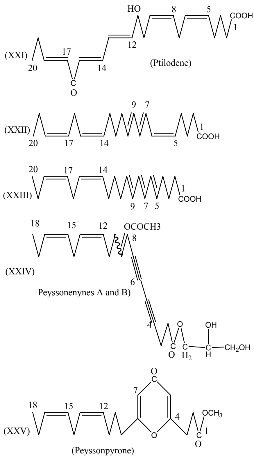
Figure 7: PUFA-related compounds from Rhodophyceae.
