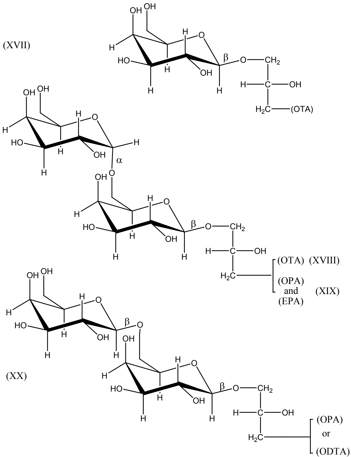
Figure 6: Mono- and di-D-galactosyl lysoglycerides from Dinophyceae and Haplophyceae.
