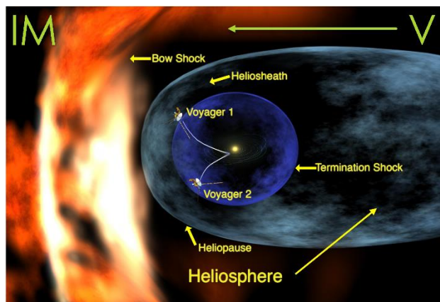
Figure 1: Sun moving through the interstellar medium [Zell, Holly. 2015]
