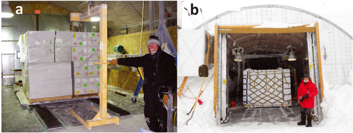
Fig. 7. (a) View of the inside of the core-handling arch showing an AFP with four wood skids (32 ISC boxes) of ice core. Also shown is the roller track system on the floor to facilitate the movement of the AFPs. (b) A finished AFP of ice cores sits inside the core-handling arch as it waits for its cold-deck LC-130 flight to McMurdo Station.
