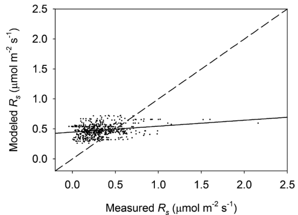
Fig. 6. Relationship between all R_s measurements made from January to March and corresponding modeled R_s . The linear relationship is represented by the solid line while the dashed line has a 1:1 slope.
