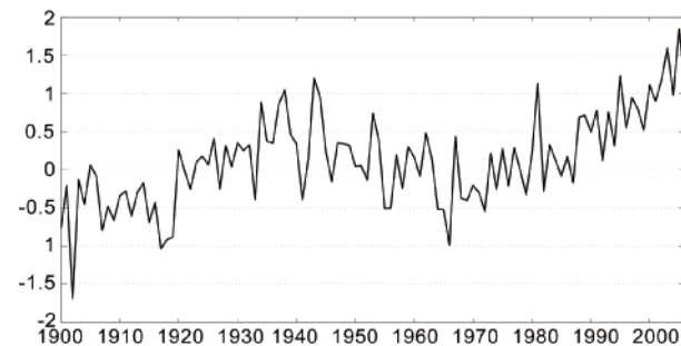
Fig. 5.2. Arctic-wide and annually averaged surface air temperature anomalies (°C; 60°N–90°) over land for 1900–2006 based on the CRU TEM2V monthly data set. Anomalies are relative to the twentieth-century average.
