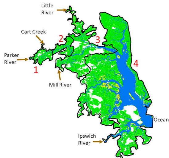
Figure 1. Plum Island Sound estuary highlighting the four zones along the 24-km axis where a sediment balance was constructed. The most significant river inputs to the system are identified. The colors correspond to elevation and land cover: white, uplands or barrier island >2-m NAVD88; green, intertidal marshes dominated by Spartina patens between 0.8 and 2-m NAVD88; yellow, intertidal wetlands dominated by Spartina alterniflora between 0 and 0.8-m NAVD88; blue, open water and intertidal flats <0 NAVD88. The ocean adjacent to the estuary is the Gulf of Maine. The coordinates at the mouth of the estuary are 42°41.489'N 70°45.555'W. North is straight up the image.
