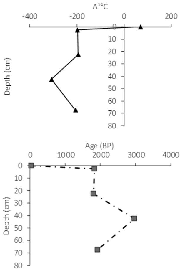
Figure 7. \Delta^{14}\text{C} and ^{14}\text{C} age of clay-bound fine particulate organic carbon distribution in a core of Spartina patens marsh sediment from the Plum Island Sound estuary.
