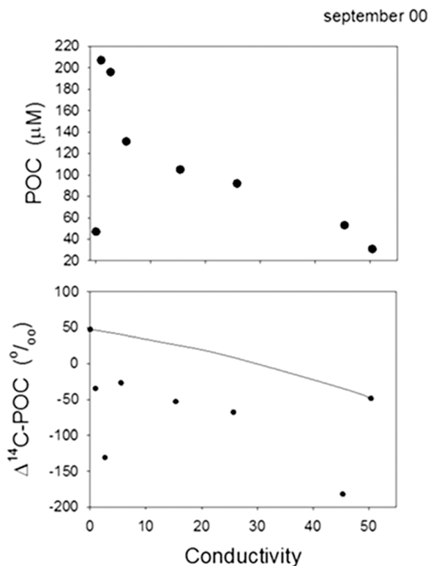
Figure 6. (top) Particulate organic carbon concentration and \Delta^{14}\text{C} -POC versus conductivity (dots) and the conservative mixing curve (curved line in bottom figure) along the entire length of the Plum Island Sound estuary in September 2000. Plotting against a conservative tracer is essential for using a two end-member mixing model to calculate the mass of ancient marsh carbon required to match the ^{14}\text{C} values as observed.
