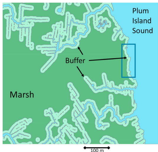
Figure 3. An example from along the northwestern edge of Plum Island Sound showing the delineation of the 10-m buffer. Note that the buffer is readily apparent along mosquito ditches, first, second, third, and fourth-order tidal creeks, Plum Island Sound, and marsh ponds. The blue rectangular box delineates the zone where we show selective results of marsh edge erosion during the 2005–2011 interval.
