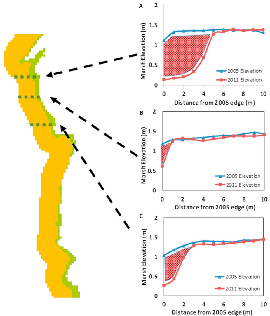
Figure 4. Example of edge erosion for three transects (dark green dotted lines on map) adjacent to the NW shoreline of Plum Island Sound (see Figures 2 and 3). The map to the left shows the 10-m buffer delineated from the 2005 digital elevation model. The green band along the right side of the buffer represents area that had eroded by 2011. Cross sections of marsh elevation along each of the transects are shown in graphs A–C.
