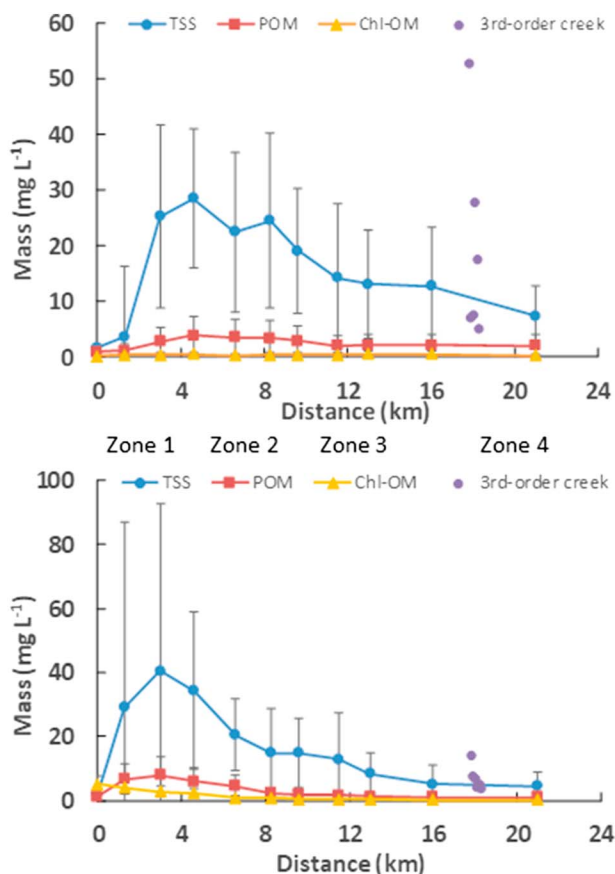
Figure 5. Thirteen-year median (CV, error bars) distribution of total suspended solids, particulate organic matter, and chlorophyll a converted to organic matter along the main axis of the Plum Island Sound estuary in (top) spring (during high river flow) and (bottom) fall (during low river flow). Also shown is the distribution of suspended solids along the length of a third-order tidal creek off Plum Island Sound during 2016.
