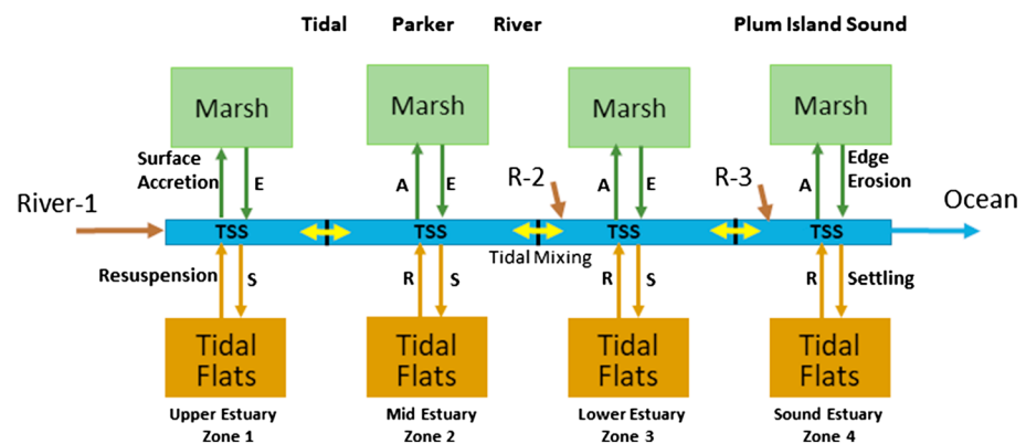
Figure 2. Box model used to examine sediment budget of the Plum Island Sound, marsh-dominated estuary. The estuary is divided into four sections, each with open water (estuarine tidal creeks and bays), intertidal flats, creek bottoms, and adjacent intertidal marsh. Sediment enters the system via rivers (River-1 refers to the Parker River and other ungauged stream inputs to the upper 5 km of the estuary. R-2 refers to the Mill and Little Rivers that are also ungauged and that enter in the lower estuary. R-3 refers to the Ipswich River and other ungauged stream inputs including the Rowley River). Edge erosion (E) refers to the sediment entering each section of the river via erosion of marsh creek banks. (a) Surface accretion is the mass of sediment coming from flood tide waters that sustains marsh elevation gain. Resuspension (R) and settling (S) refer to solids that exchange between the water column and creek bottoms in association with variations in tidal current velocities. Ocean refers to the sediment that enters or exits from the ocean. All terms including the standing stock of total suspended solids in the water column of each estuarine section were measured explicitly in this study except for exchanges with tidal flats and the ocean, which were calculated by mass balance.
