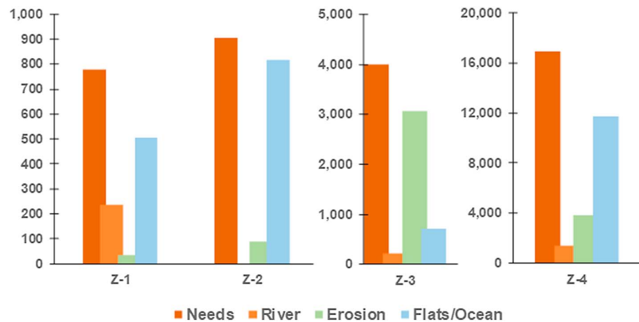
Figure 8. Summary of river, shoreline erosion, and ocean or tidal flats and creek bottom mineral sediment inputs to marshes in four zones along the Plum Island Sound estuary that enable marshes to maintain elevation relative to current rates of sea level rise ( 2.8 \text{ mm yr}^{-1} ). Unit: \text{MT d}^{-1} .
