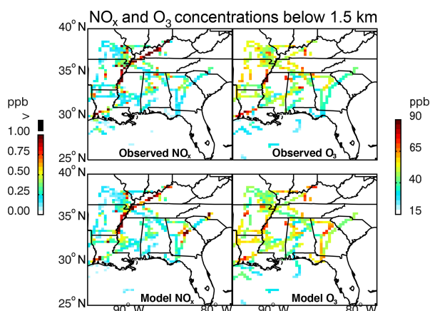
Figure 4. Ozone and \text{NO}_x concentrations in the boundary layer (0–1.5 km) during SEAC 4 RS (6 August to 23 September 2013). Observations from the aircraft and simulated values are averaged over the 0.25^\circ \times 0.3125^\circ GEOS-Chem grid. \text{NO}_x above 1 ppb is shown in black. The spatial correlation coefficient is 0.71 for both \text{NO}_x and \text{O}_3 . The normalized mean bias is -11.5\% for \text{NO}_x and 4.5\% for \text{O}_3 .
