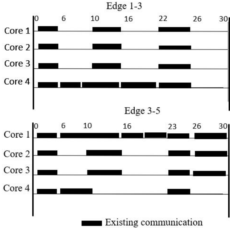
Figure 3.8: Before allocation of the new request
