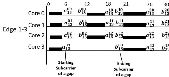
Figure 3.5: Concept of Gaps
