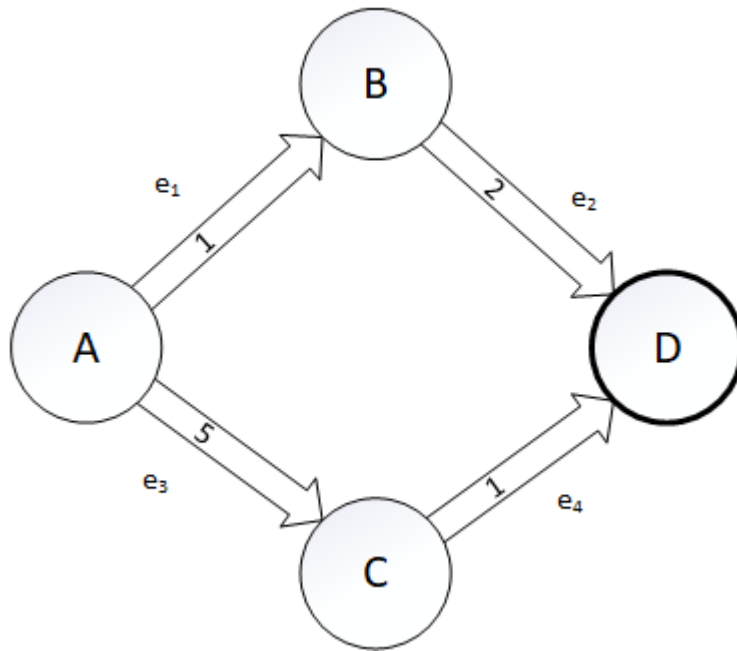
Figure 7: Problem Graph featuring a static single resource per edge.
