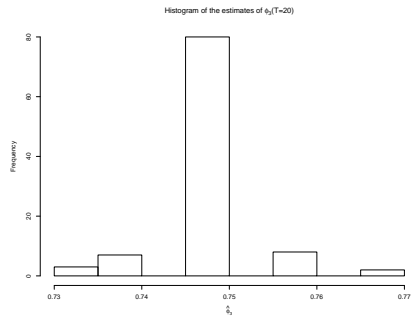
(c) Histogram of \hat{\phi}_3 (T = 20)
