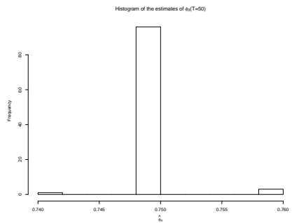
(i) Histogram of \hat{\phi}_3 (T = 50)
