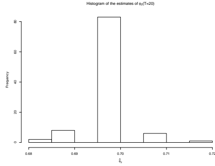
(b) Histogram of \hat{\phi}_2 ( T = 20 )
