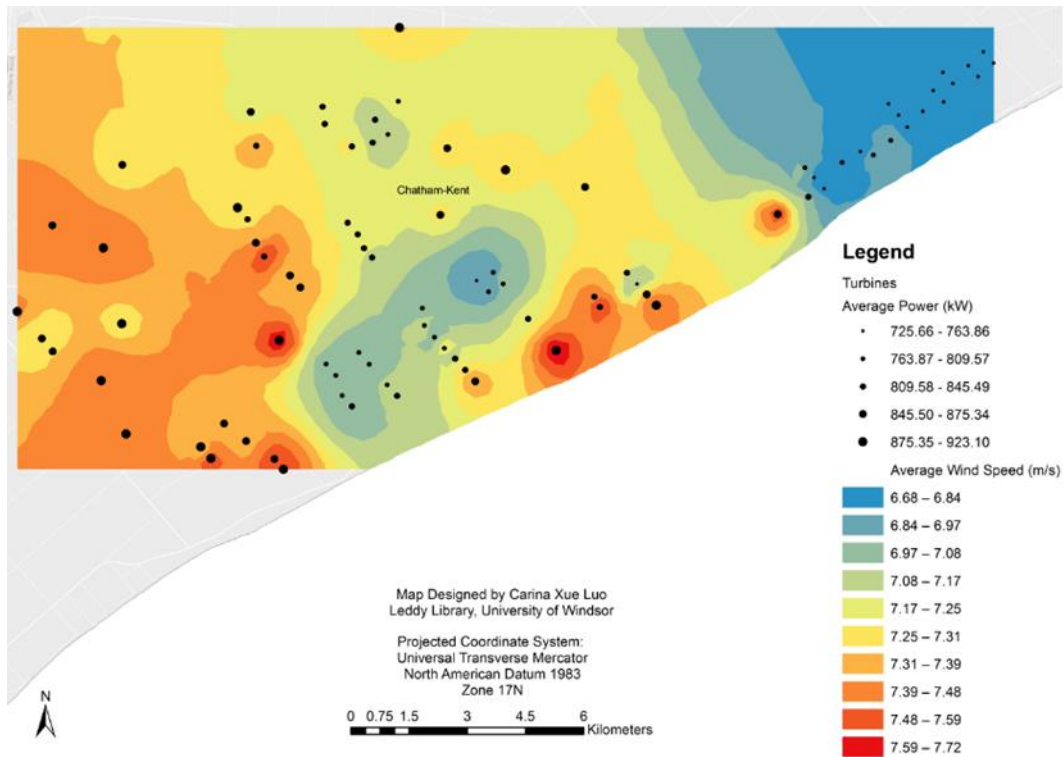
Figure 2. 4: Average wind speed and average power produced for wind farm 1.
