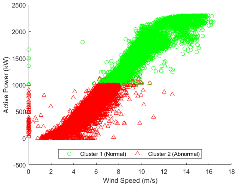
Figure 4. 2: Clustering results from monitoring blade SCADA parameters with wind speed and power shown.
