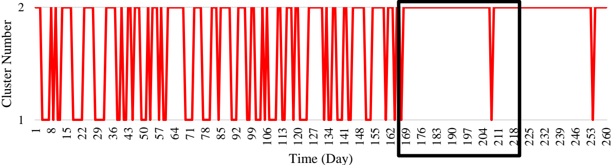
Figure 4. 5: Assigned clusters for each day for the first 260 days of the dataset for wind turbine 42 with a 50-day moving window.
