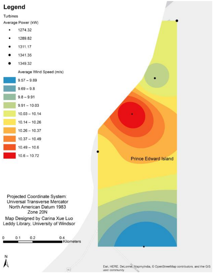
Figure 2. 6: Average wind speed and average power produced for wind farm 3.
