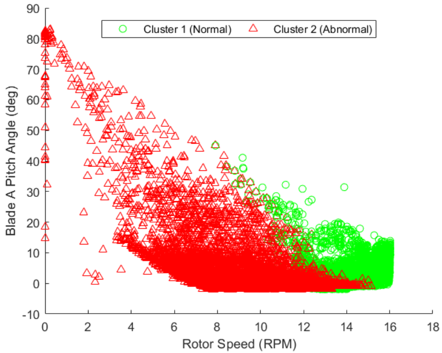
Figure 4. 1: Clustering results from monitoring blade SCADA parameters with rotor speed and blade pitch shown.
