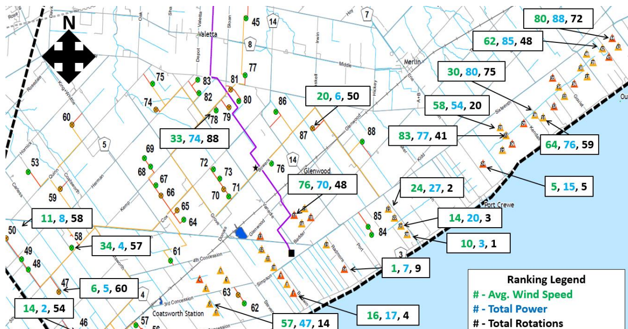
Figure 2. 3: Ranking of wind speed and select SCADA variables (from highest to lowest) for select turbines at farm 1.
