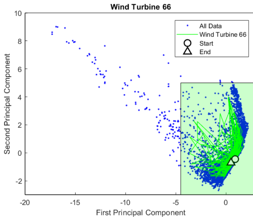
Figure 3. 6: The path taken by wind turbine 66 that appears to be operating normally, but repairs were still performed.
