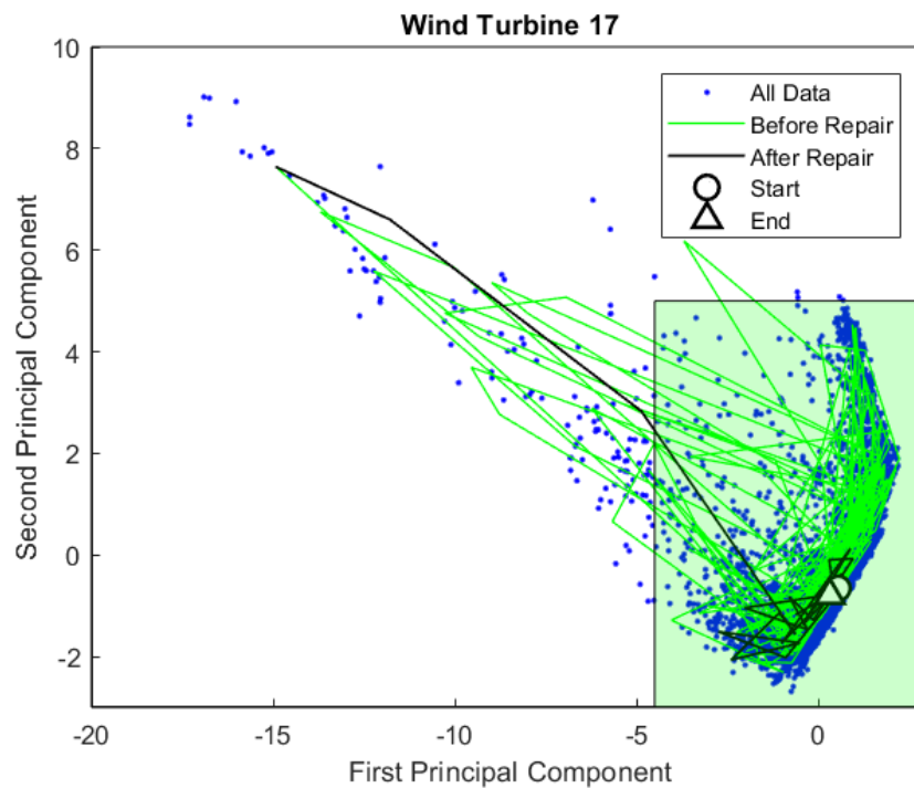
Figure 3. 7: The path taken by wind turbine 17 blades before and after repairs were performed.
