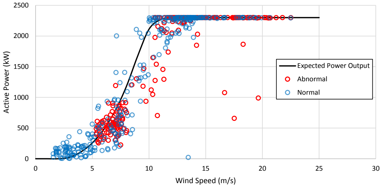
Figure 3. 5: Power curve comparison for wind turbine 1.
