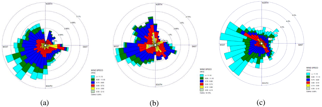
Figure 2. 2: Wind rose for (a) wind farm 1, (b) wind farm 2, and (c) wind farm 3 measured by on-site meteorological mast.
