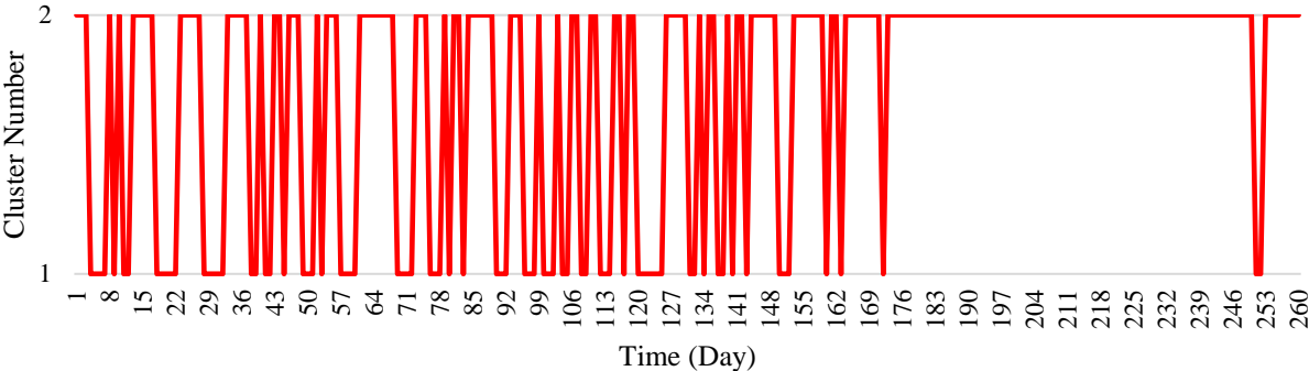
Figure 4. 4: Assigned clusters for each day for the first 260 days of the dataset for wind turbine 47.
