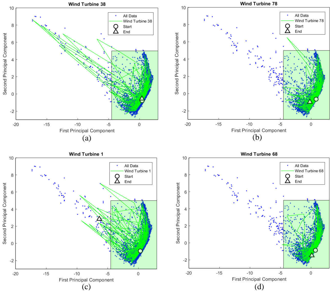
Figure 3. 4: The path that the blades of wind turbines (a) 38, (b) 78, (c) 1, and (d) 68 take respectively from the start of the dataset to the end.
