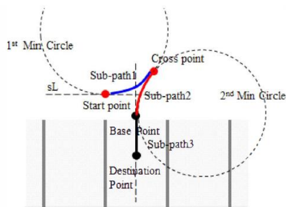
Figure 2.7: Three step parking maneuver for backward perpendicular parking [19]
