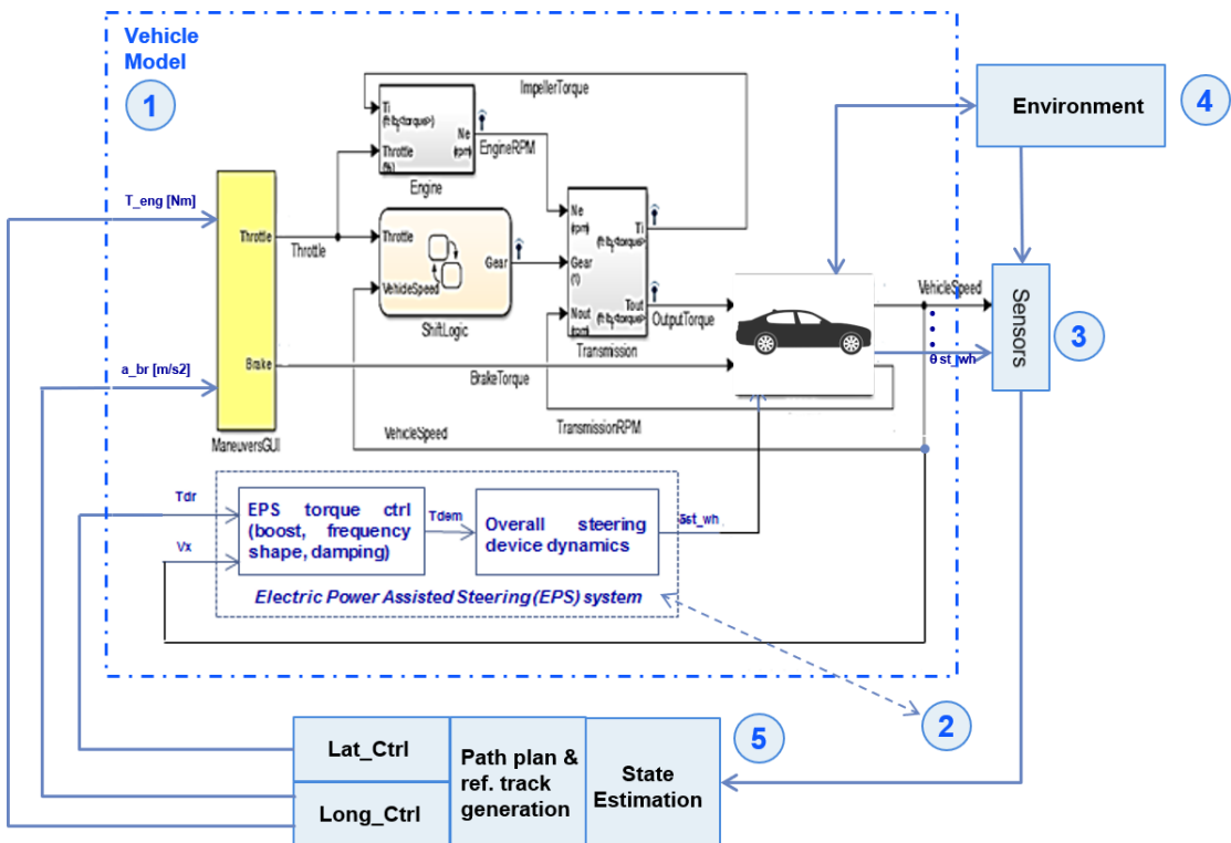
Figure 1.4: Functional System Architecture
