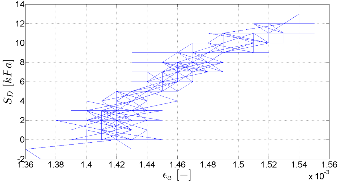
Figure 33 Triaxial test results for 0.01% axial strain amplitude
