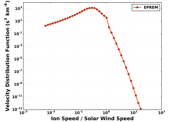
FIG. 11. This figure is the same as Figure (9) except that the field line is traced to 5 AU.
