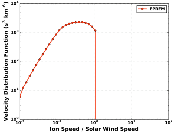
FIG. 13. This plot shows the distribution function at 1 AU with no CIR included in the simulation.
