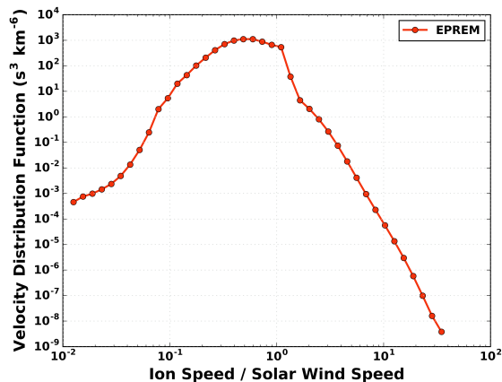
FIG. 16. This figure is the same as Figure (15) except with \alpha = 4 ( D \propto v^2 ). The only difference in the distributions is in the thermal part of the distribution.
