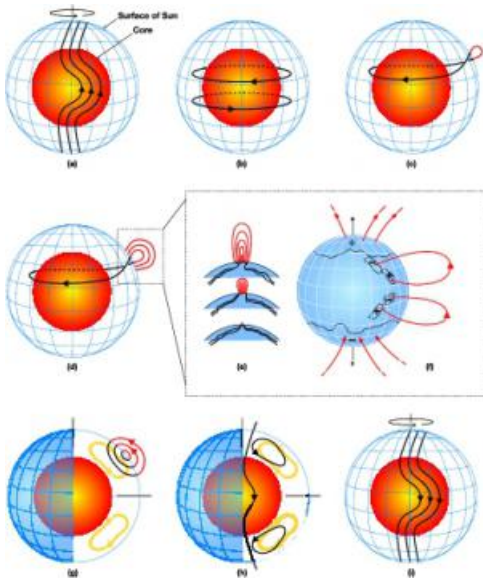
FIG. 2. The diagram shows the Sun's full solar cycle as the field starts predominantly poloidal, becomes more toroidal and then becomes dominantly poloidal again, with the opposite polarity as when the solar cycle started. This figure was taken from [3].
