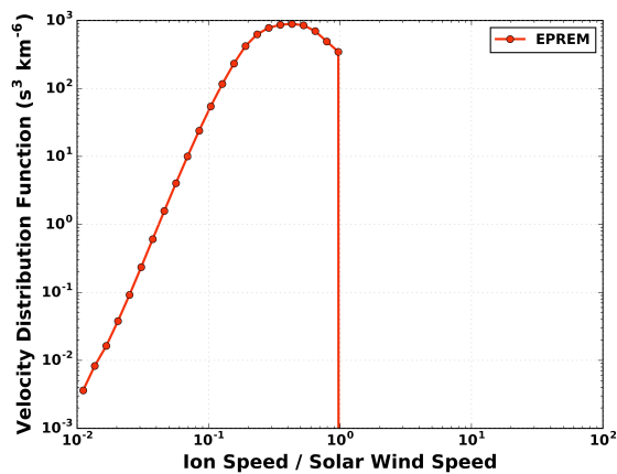
FIG. 5. This image shows the log-log plot of the PUI distribution (number of particles) at 1 AU versus the magnitude of the particle velocity (normalized to the solar-wind velocity). This simulation was run without a CIR or momentum-diffusion.
