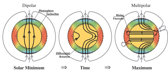
FIG. 1. The effect on the magnetic fields from the differential rotation of the Sun through time. This figure was taken from [2].
