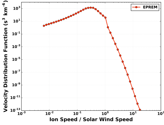
FIG. 12. This figure is the same as Figure (11) except that the diffusion coefficient parameter \alpha = 3.5 ( D \propto v^{1.5} ).
