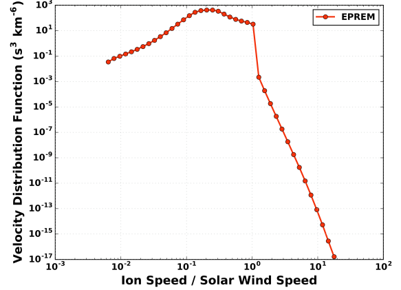
FIG. 10. This figure is the same as Figure (8) except that the field line is traced to 5 AU.
