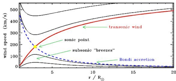
FIG. 3. The figure shows 4 of the 6 possible solution types. The other two are not explicit functions of r and are therefore ignored. The Parker solar wind solution is the transonic wind solution. This figure was taken from [5].
