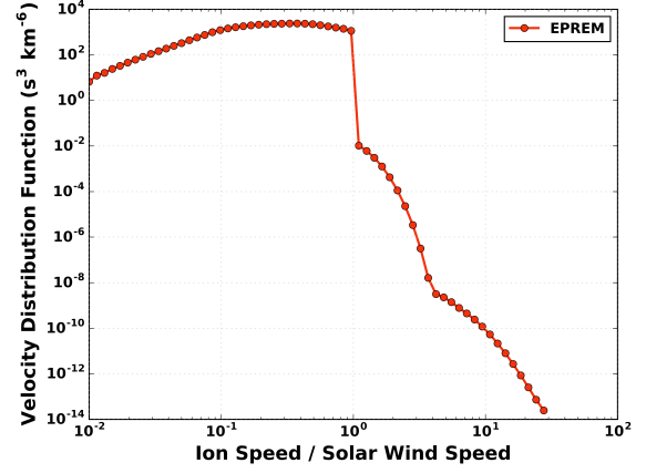
FIG. 14. This plot is the same as Figure (13) except with momentum-diffusion included. The momentum-diffusion parameters are the same as Figure (9).
