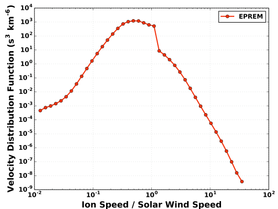
FIG. 7. The plotted PUI distribution inside the compression region at 1 AU. The slope of the tail is softer than v^{-5} , but does demonstrate acceleration of the PUIs when compared to Figure (5).
