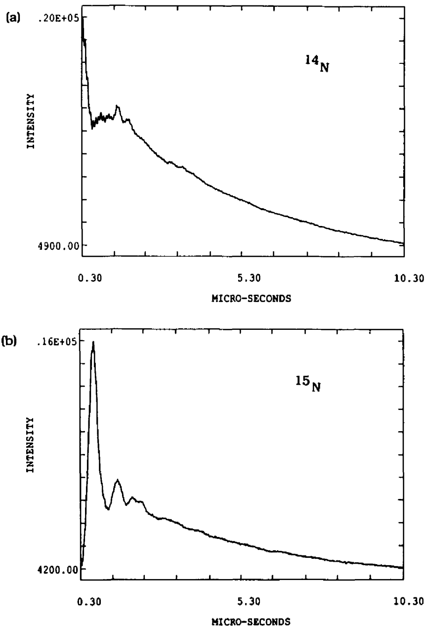
Figure 4.8 (a) Three pulse ESEEM spectrum of C^{14}N adduct along g_{yy} . Data file SE2875.NIP. Frequency-8.78 GHz, Field-2906 G., tau-242 nsec. (b) C^{15}N spectrum. Data file SE2886.NIP. Frequency-8.76 GHz, Field-2906 G., tau-323 nsec.
