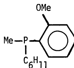
(+)-(R)-ACMP (Ref. 12, 13)
