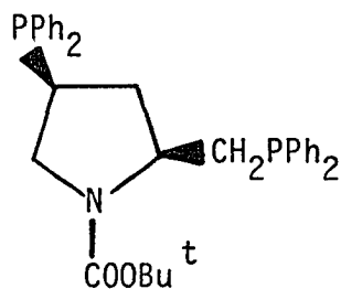
(-)-(2S,4S)-BPPM (Ref. 29)
