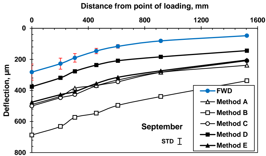
Figure 5.7. Measured and Predicted Deflection Basins for Texas Section
