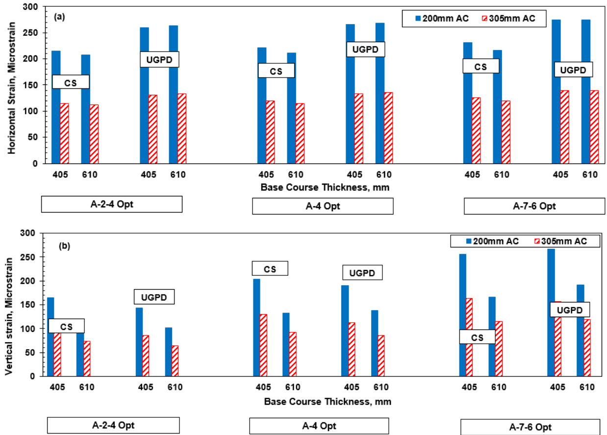
Figure 2.6. (a) Horizontal strain (b) Vertical strain at optimum moisture content under different base course and subgrade material types under single loading type on Interstate cross sections
