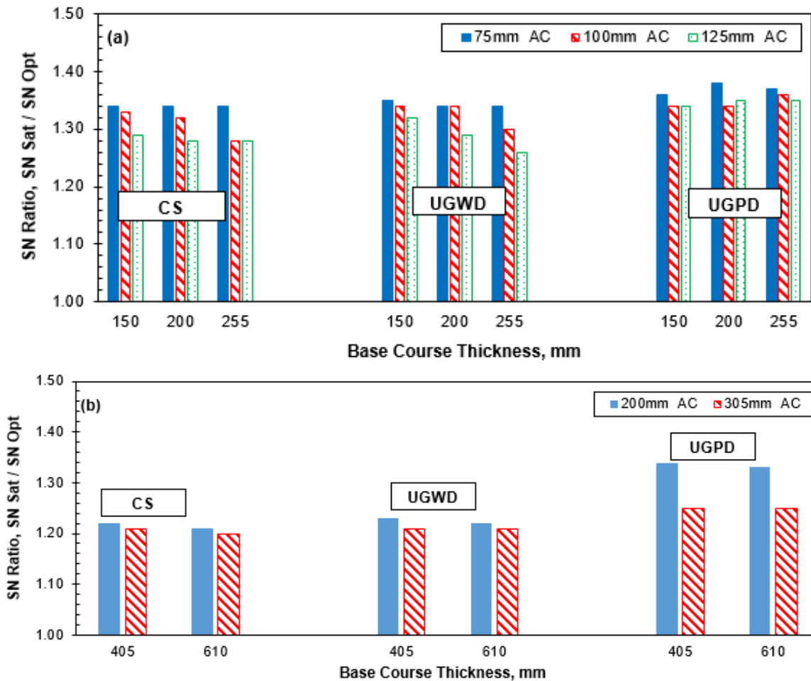
Figure 2.11. Ratio of saturated to optimum moisture condition for the structural Number (SN) for (a) Low volume sections (b) interstate sections under different base course types
