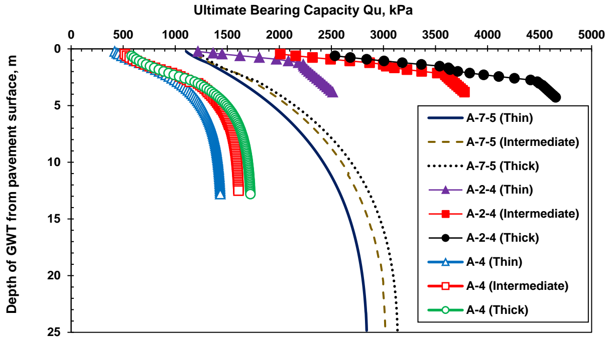
Figure 6.3. Variation of bearing capacity with groundwater table levels for the proposed soils
