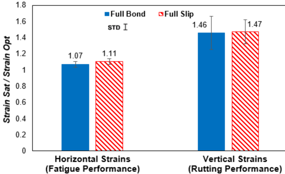
Figure 2.2. Ratio of saturated to optimum moisture condition for horizontal tensile strain and vertical compressive strain under full bond and full slip interlayer conditions for low volume roads.
