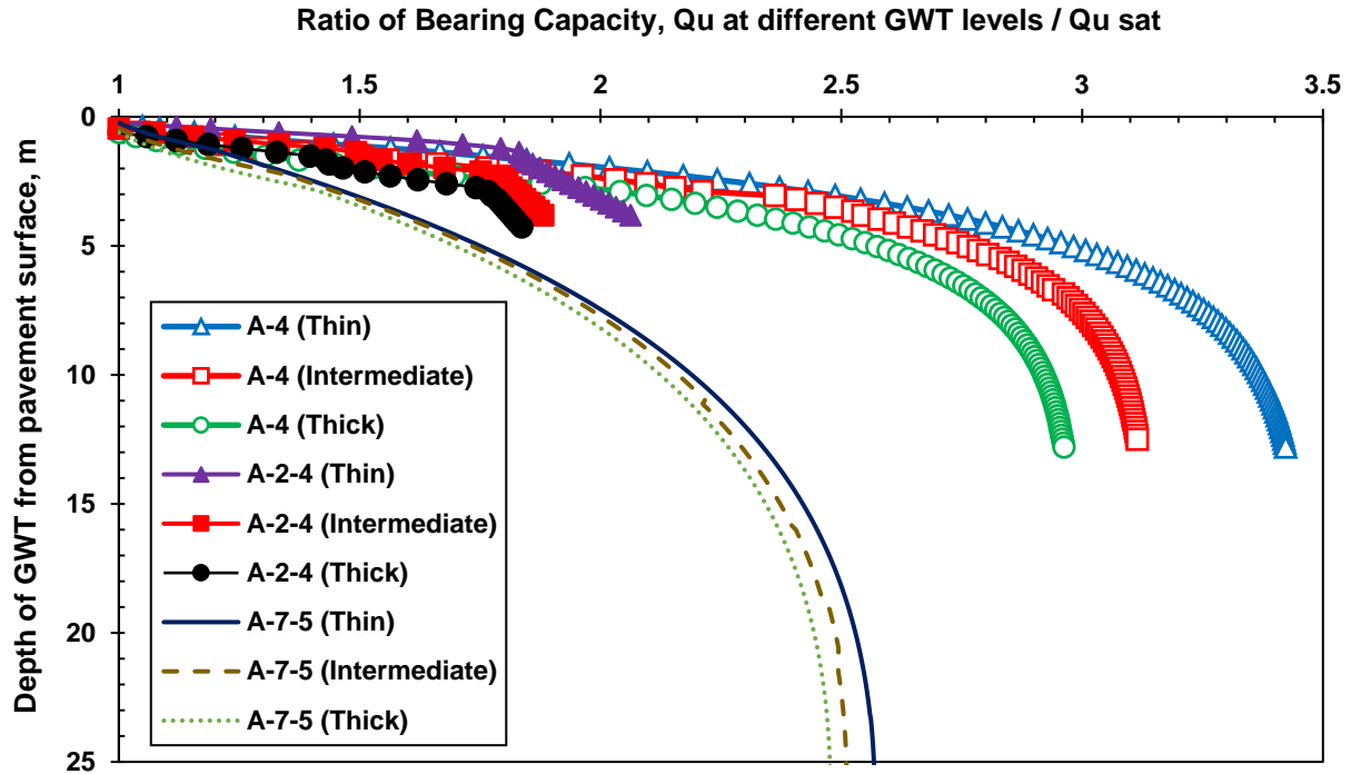
Figure 6.4. Ratio of bearing capacity with groundwater table levels for the proposed soils
