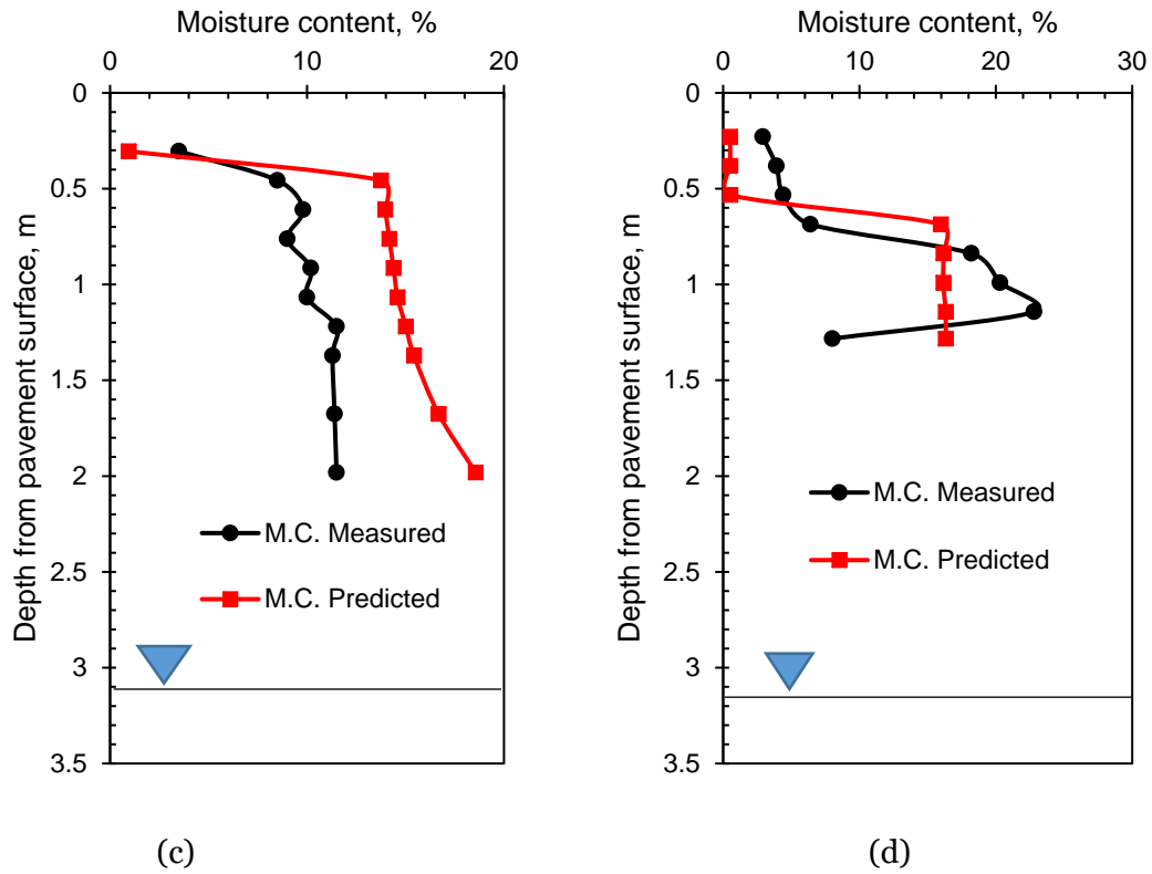
Figure 5.4. TDR Measured and Suction - SWCC predicted moisture content profiles for (a) Maine section; (b) Minnesota section; (c) Texas section; (d) Montana section
