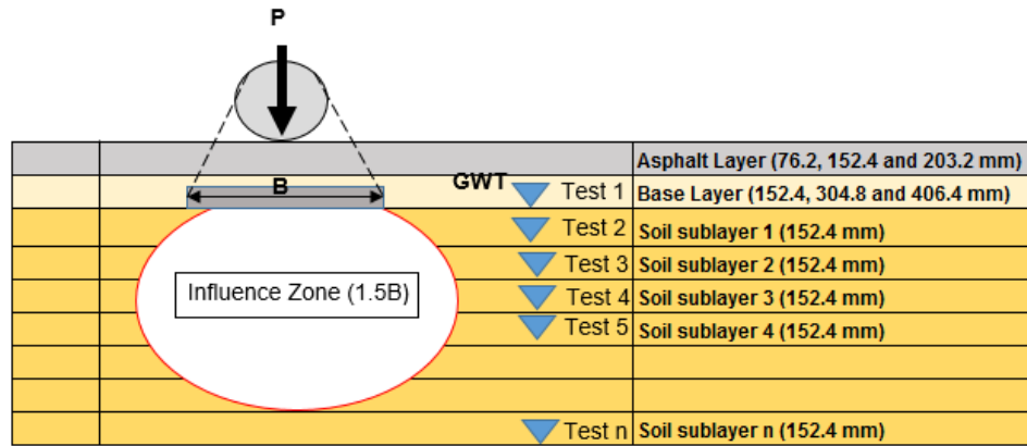
Figure 6.2. Schematic to demonstrate the pavement cross section and the analysis approach
