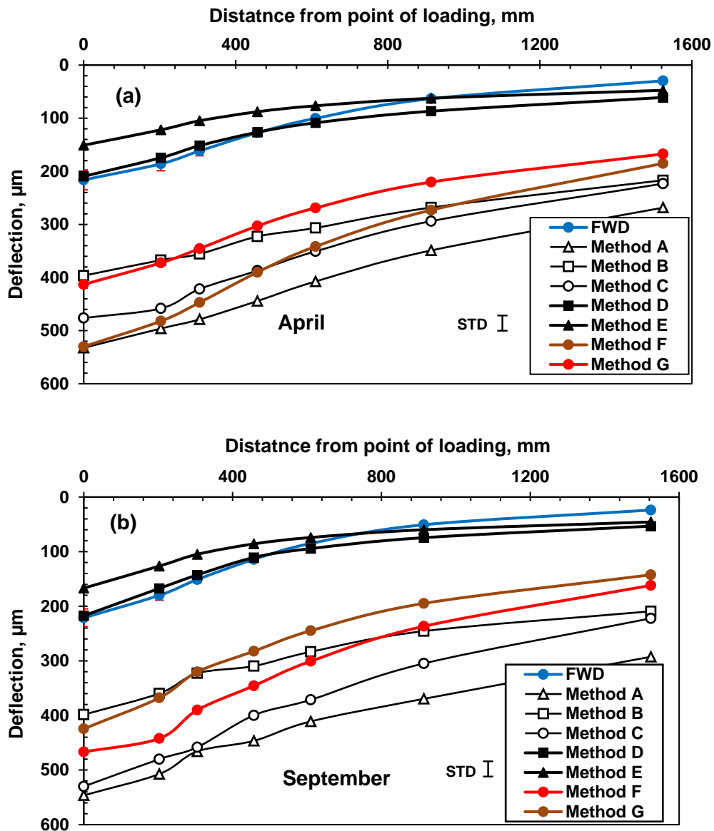
Figure 5.5. Measured and Predicted Deflection Basins for Maine Section (a) April (b) September
