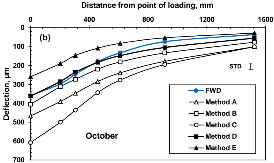
Figure 5.6. Measured and Predicted Deflection Basins for Minnesota Section (a) April (b) October
