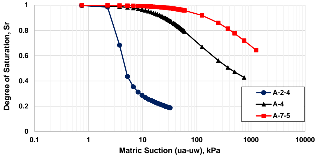
Figure 4.3. Predicted SWRC for the proposed soils
