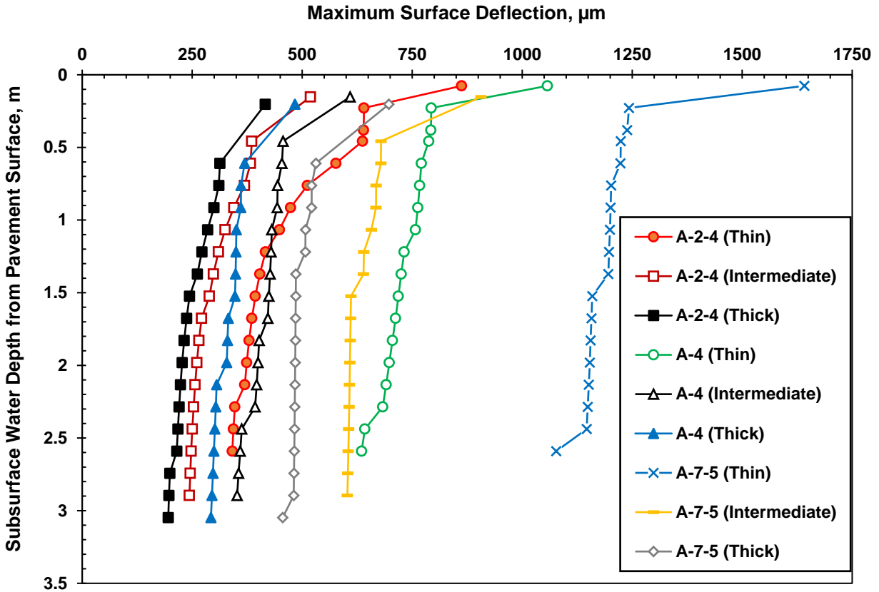
Figure 4.4. Variation of the maximum surface deflection with depth of subsurface water levels
