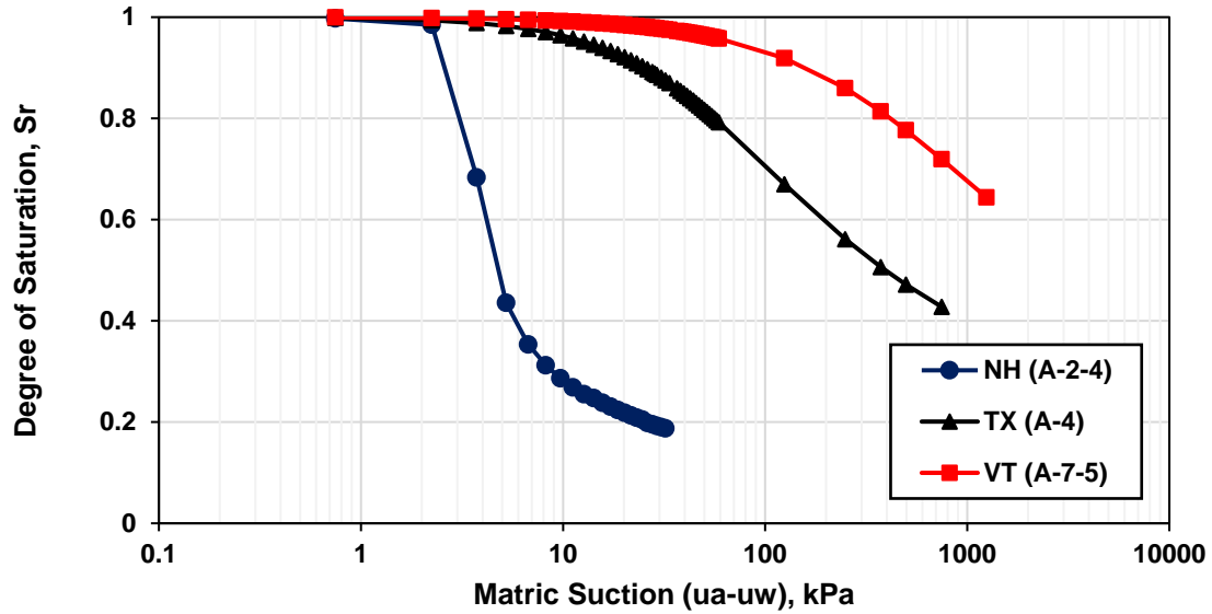
Figure 6.1. Predicted SWRC for the proposed soils
