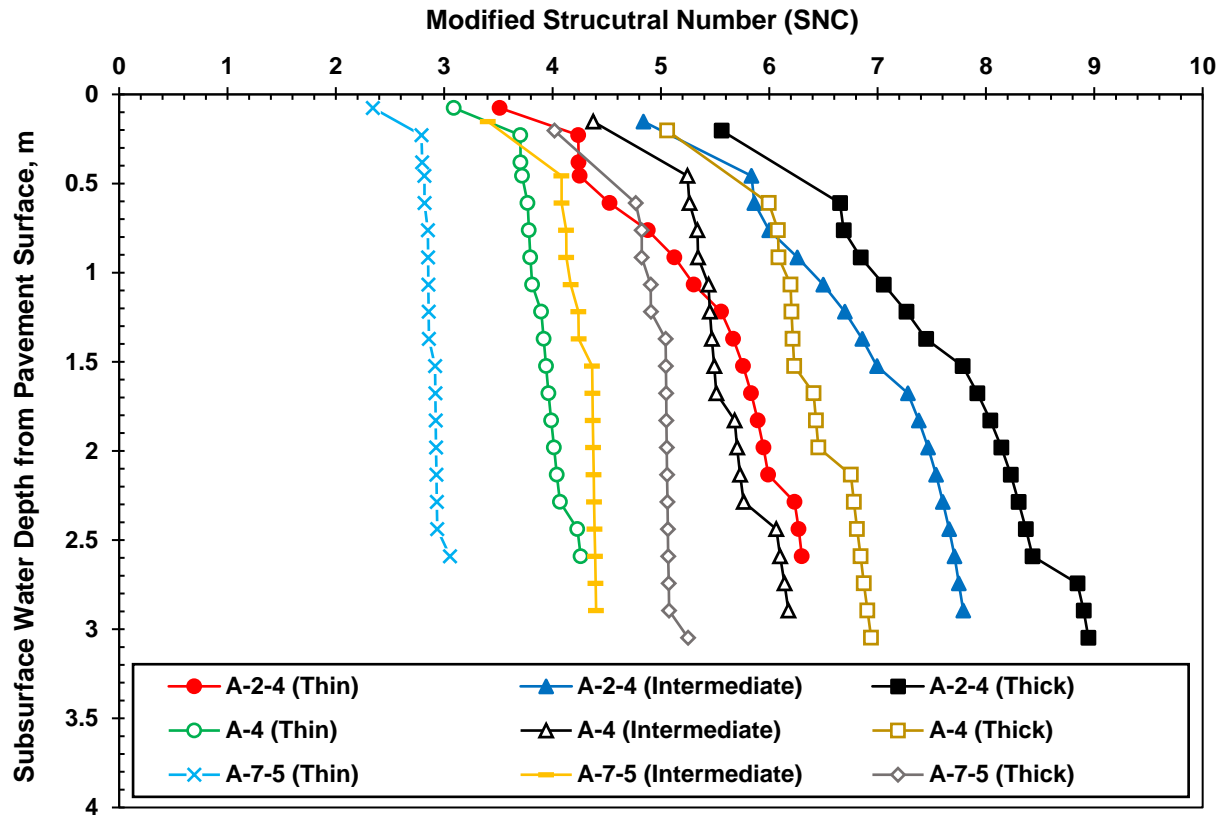
Figure 4.7. Variation of the modified structural number with subsurface water levels
