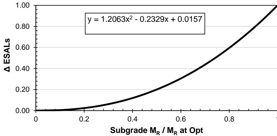
Figure 2.12. Change in ESALs versus change in subgrade resilient modulus
