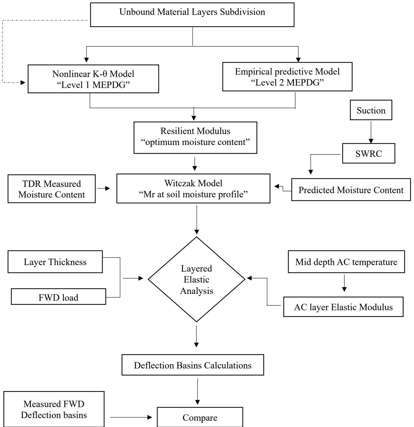
Figure 5.3. Flow Diagram of the procedure
