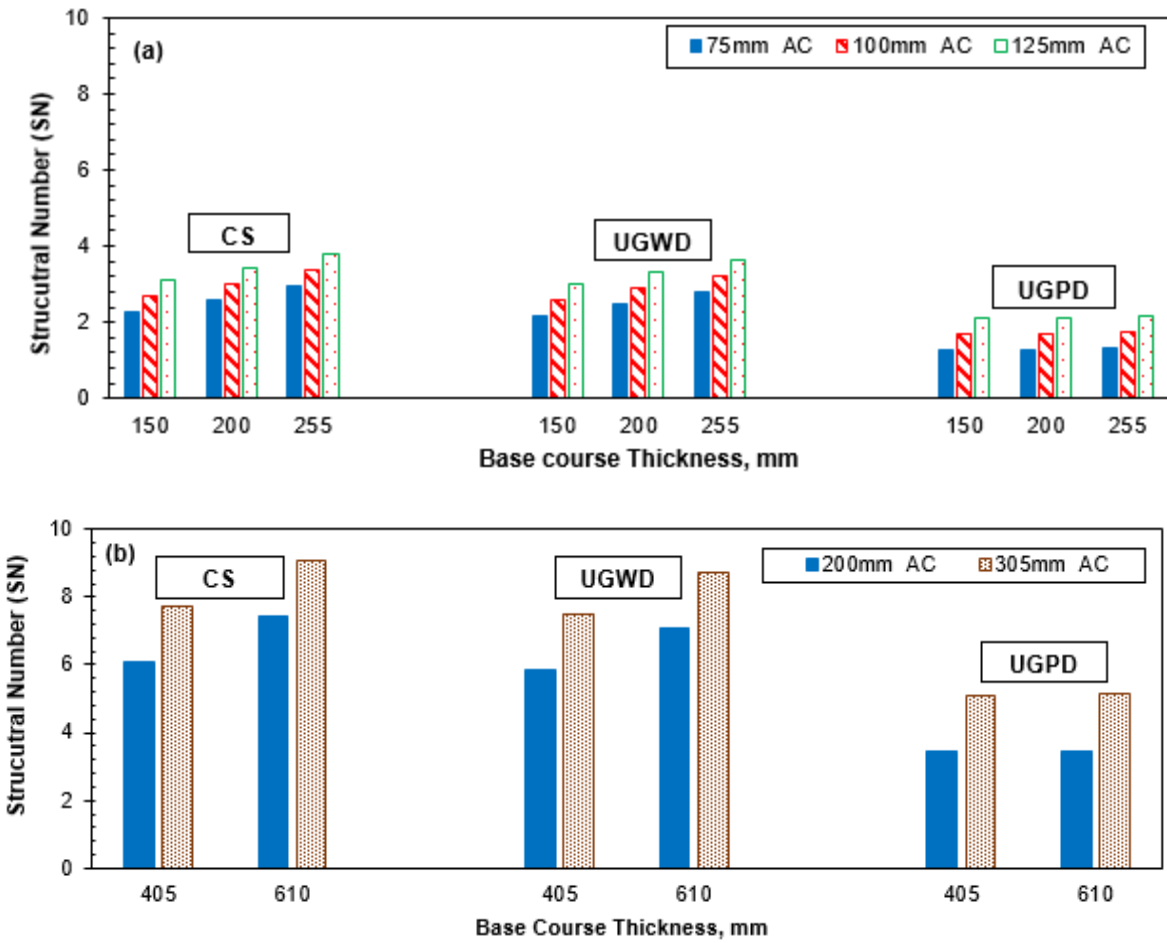
Figure 2.9. Structural number (SN) for (a) Low-volume sections (b) Interstate sections under different base course types
