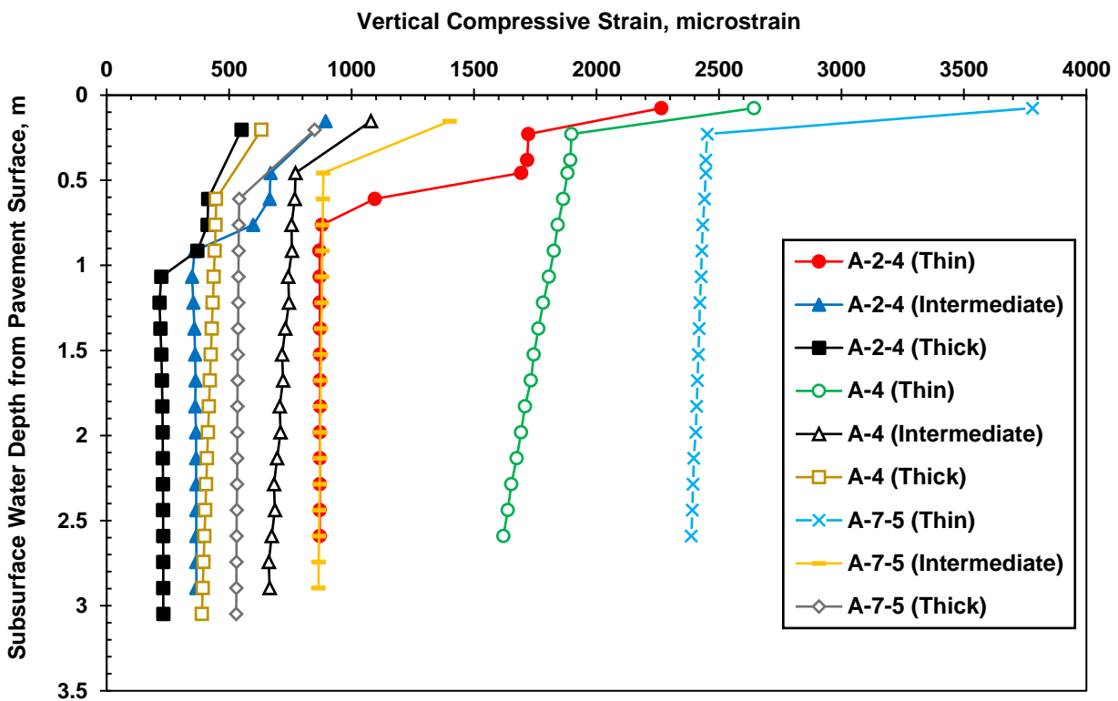
Figure 4.6. Variation of the vertical compressive strain at the top of the subgrade layer with depth to subsurface water
