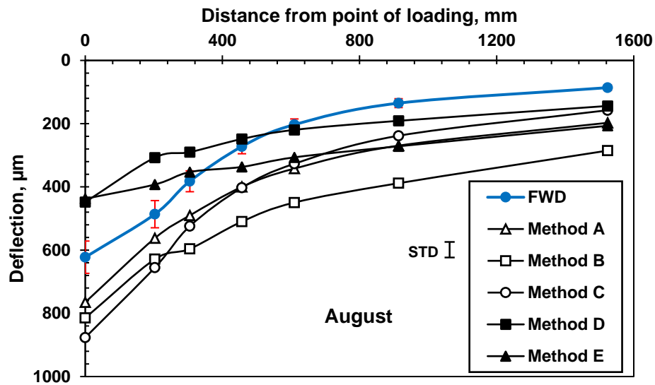
Figure 5.8. Measured and Predicted Deflection Basins for Montana Section
