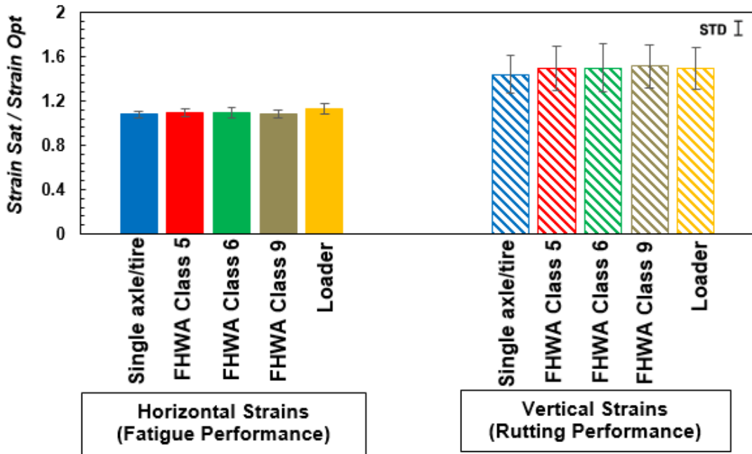
Figure 2.3. Ratio of saturated to optimum moisture condition for horizontal tensile strain and vertical compressive strain under different truck loading types for all low volume cross sections
