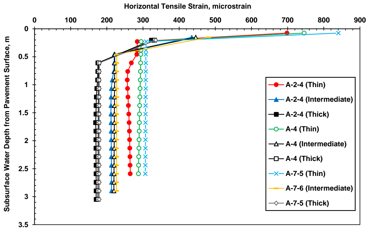
Figure 4.5. Variation of the horizontal tensile strain at the bottom of the asphalt layer with depth to subsurface water levels
