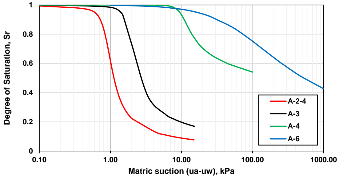
Figure 5.1. Predicted SWRC for the proposed soils
