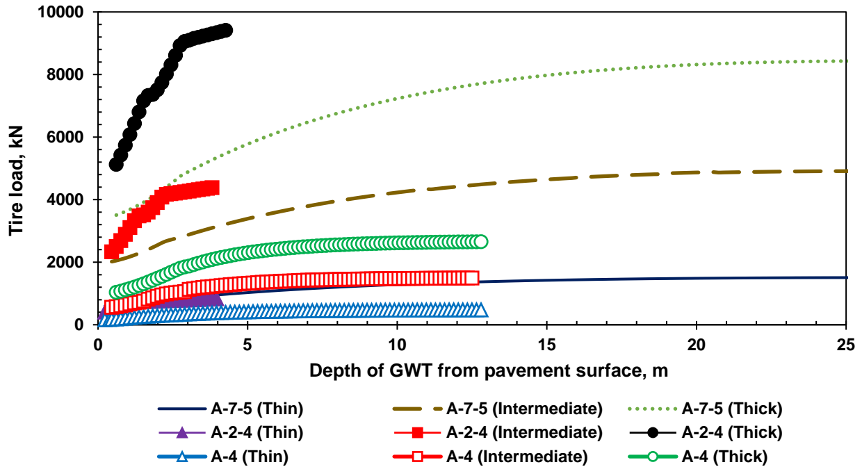
Figure 6.5. Tire loads at ultimate bearing capacity at groundwater table levels for the proposed soils
