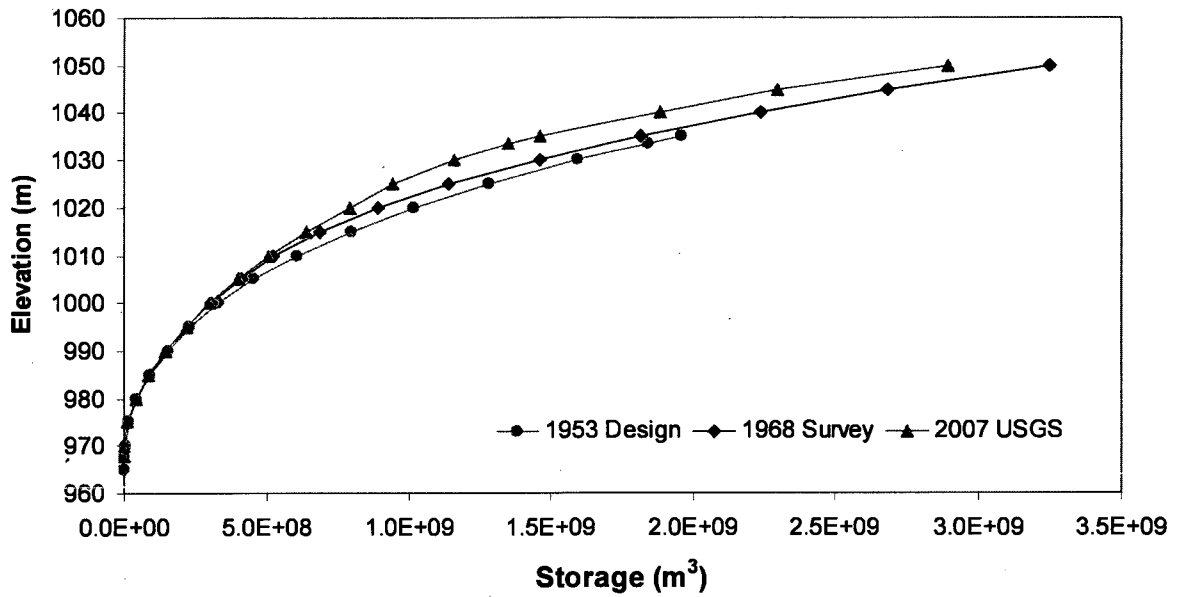
Figure 2-5 Storage-elevation relationships for the Kajakai Reservoir
