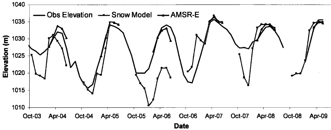
Figure 3-12 Comparison of monthly reservoir water surface elevations for water years 2004-2009; observed data (black), HMS snow model results (green), and model results using initial AMSR-E SWE (red)
