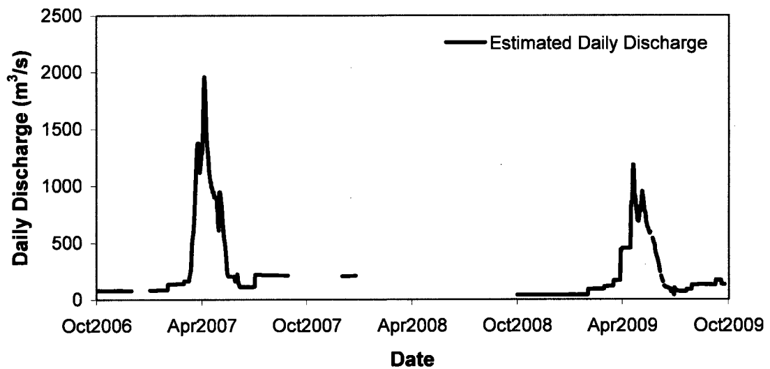
Figure 2-6 Estimated daily discharge from Kajakai Reservoir
