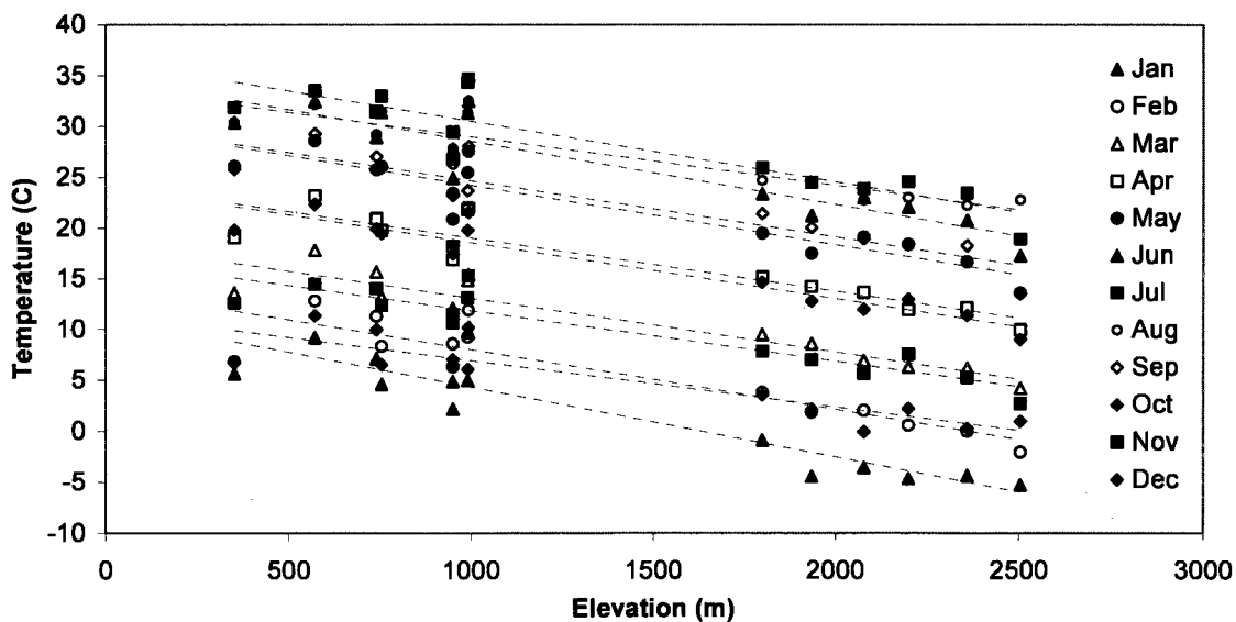
Figure 2-8 Average monthly observed temperatures, 2003 – 2009, by elevation
