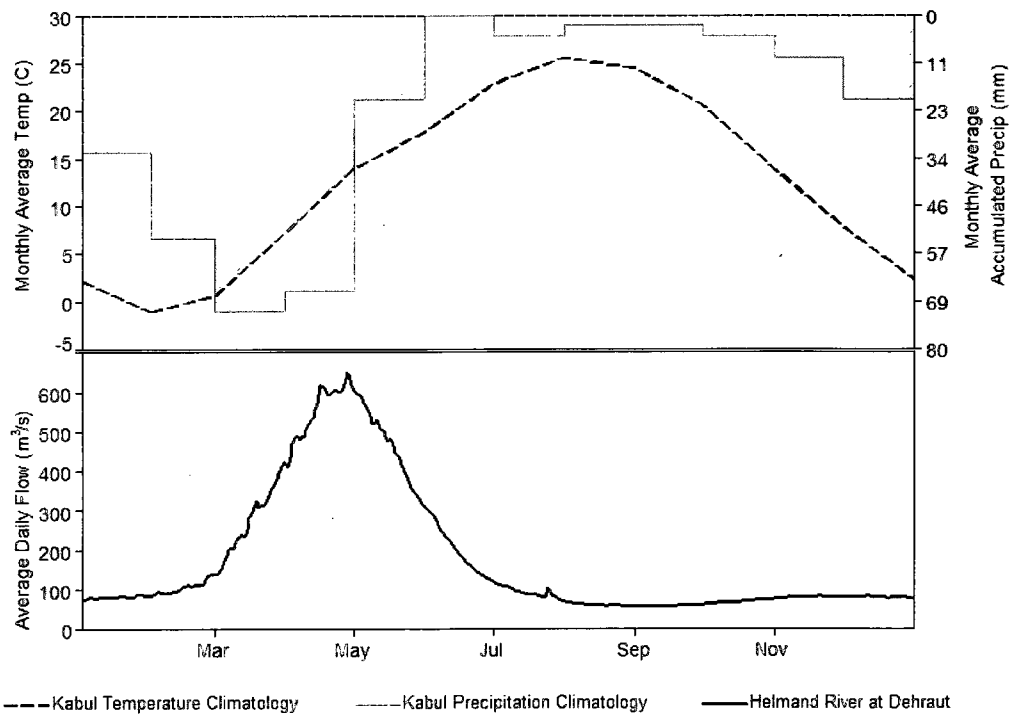
Figure 2-2 Historical stream flow and climatology data
