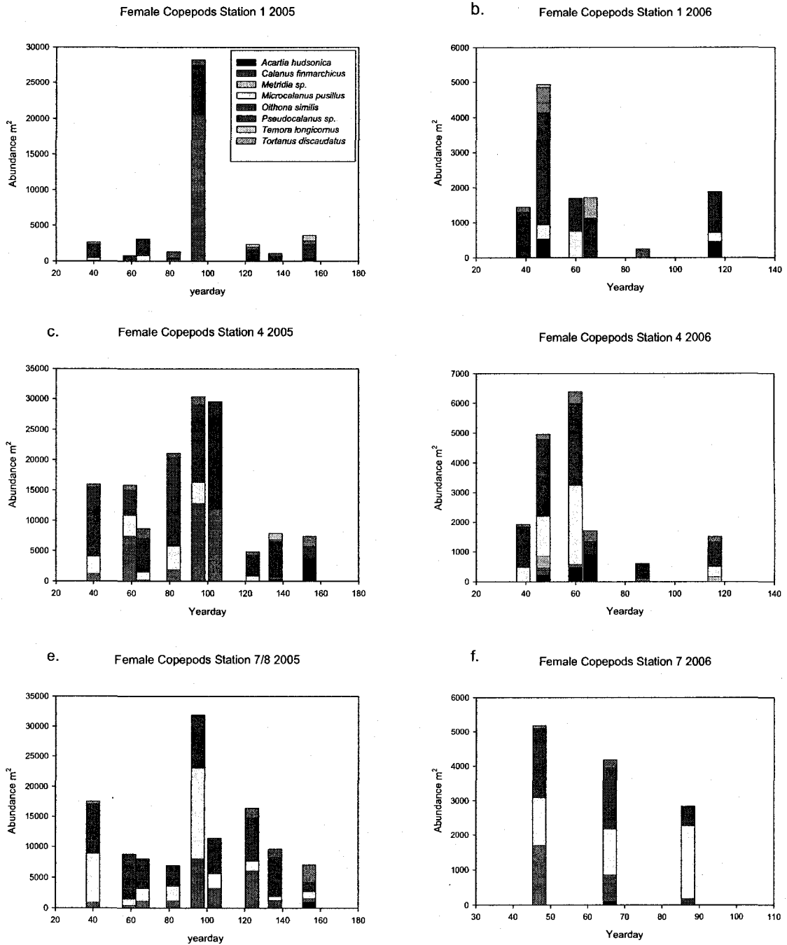
Figure 13. Female copepod abundance ( m^2 ) collected during 2005 at Stations 1 (a), 4 (c), 7 and 8 (e) and during 2006 at Stations 1 (b), 4 (d) and 7 (f). A 65 cm ring net with a 200 \mu m mesh was used to collect the vertical profile of zooplankton. Note: abundance scaling differs among panels.
