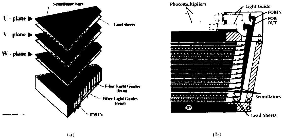
Figure 3-7: Forward electromagnetic calorimeters : (a) exploded view of one of the modules and (b) scheme of the EC light readout system where we denoted FOBIN -fiber optic bundle inner, FOBOU -fiber optic bundle outer, IP -composite inner plate.
