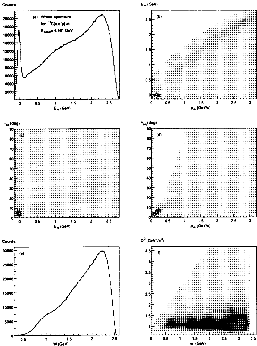
Figure 4-24: Accessible spectra for ^{12}\text{C}(e,e'p) at 4.461 GeV beam energy: (a) missing energy E_m , (b) missing energy vs. missing momentum p_m , (c) polar angle \theta_{pq} versus missing energy E_m , (d) polar angle \theta_{pq} versus missing momentum p_m , (e) invariant mass W for the (e,e'p) reaction and (f) Q^2 versus \omega distribution.
