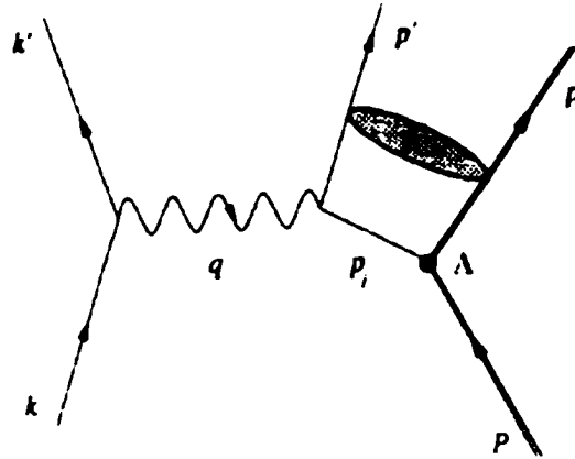
Figure 2-3: Diagram for the semi-exclusive (e,e'p) reaction. The DWIA adds to the PWIA diagram the FSI, symbolized here by the shaded area.
