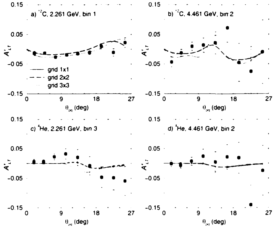
Figure 5-3: Convergence test: other cases. The theory calculation is done with OMEA (a,b) and with RMSGA (c,d) 3 . The calculated points are interpolated with Splines.
