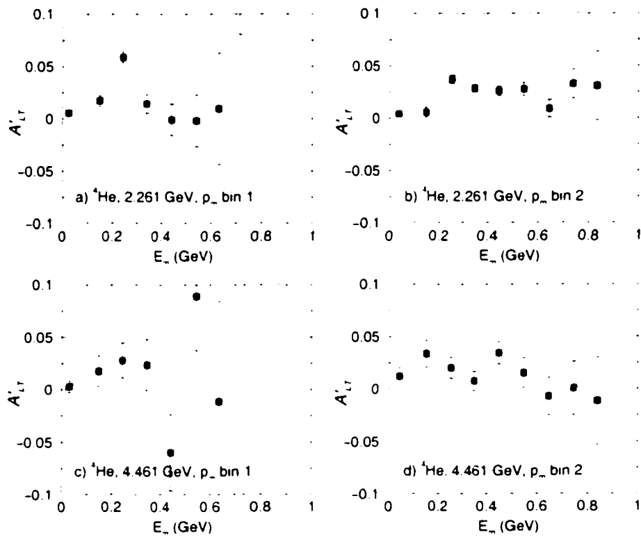
Figure 5-14: A'_{LT} versus E_m for helium. The two missing momentum bins are defined as follows: 1) 0.0 < p_m < 0.2 and 2) 0.2 < p_m < 0.45 with p_m in GeV/c. No radiative corrections were applied. Errors shown are purely statistical.
