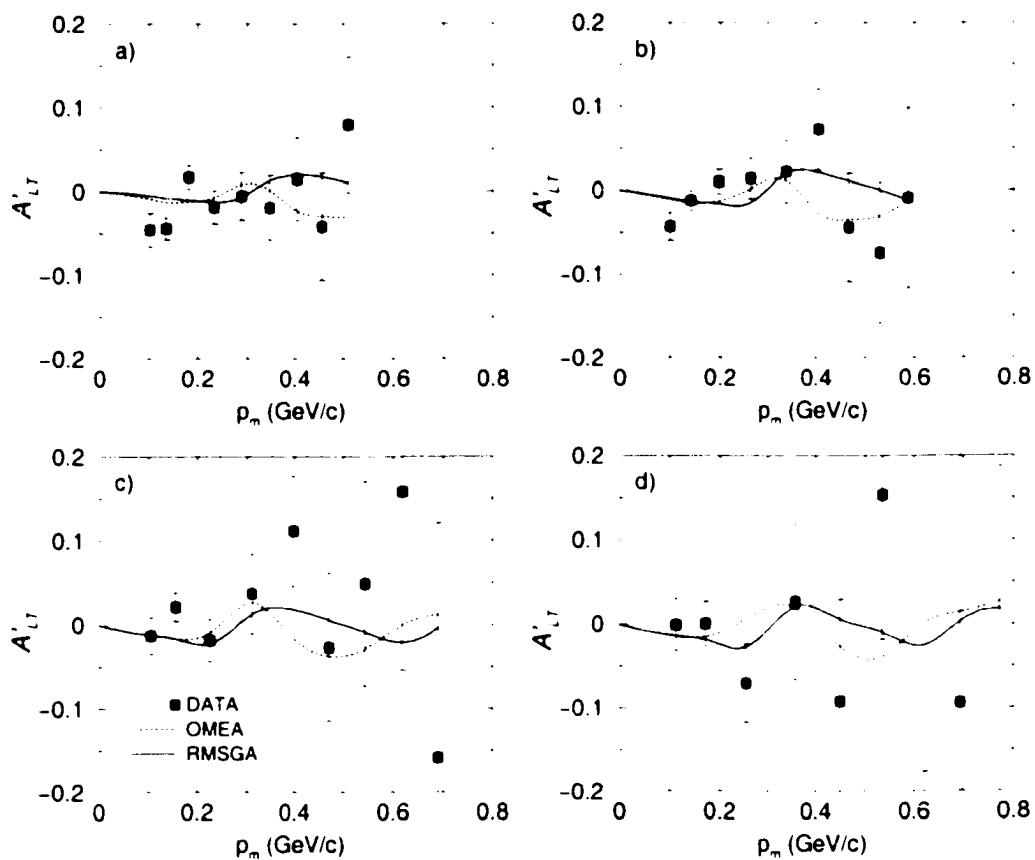
Figure 5-13: Dependence of A'_{LT} versus missing momentum p_m for ^{12}\text{C}(e, e'p) at 4.462 GeV, in four Q^2 bins along the quasielastic ridge. The Q^2 bins are set as follows: a) 0.800 < Q^2 \text{ (GeV}^2/c^2) < 1.200 , b) 1.200 < Q^2 \text{ (GeV}^2/c^2) < 1.600 , c) 1.600 < Q^2 \text{ (GeV}^2/c^2) < 2.000 and d) 2.000 < Q^2 \text{ (GeV}^2/c^2) < 2.400 . The solid (dotted) curves correspond to RMSGA (OMEA) calculations used as described in section 5.2. The data used are listed in table 5.6. Errors shown are statistical.
