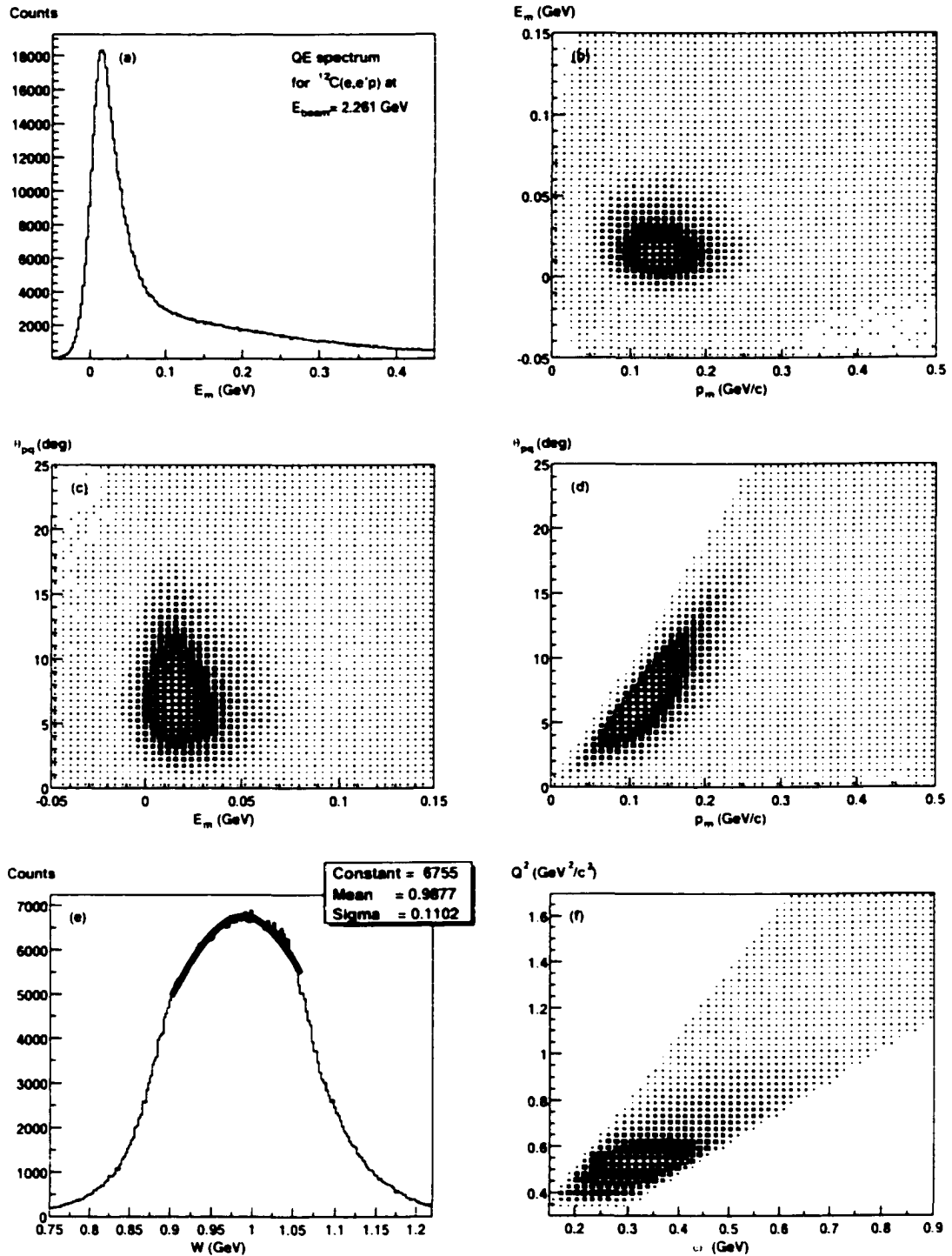
Figure 4-27: Quasielastic spectra for ^{12}\text{C}(e,e'p) at 2.261 GeV, obtained with eq.(4.18): (a) missing energy E_m . (b) missing energy vs. missing momentum p_m . (c) polar angle \theta_{pq} versus missing energy E_m . (d) polar angle \theta_{pq} versus missing momentum p_m . (e) invariant mass W for the (e,e'p) reaction and (f) Q^2 versus \omega cut. The E_m cut (4.19) is not shown. Compare to figure 4-23.
