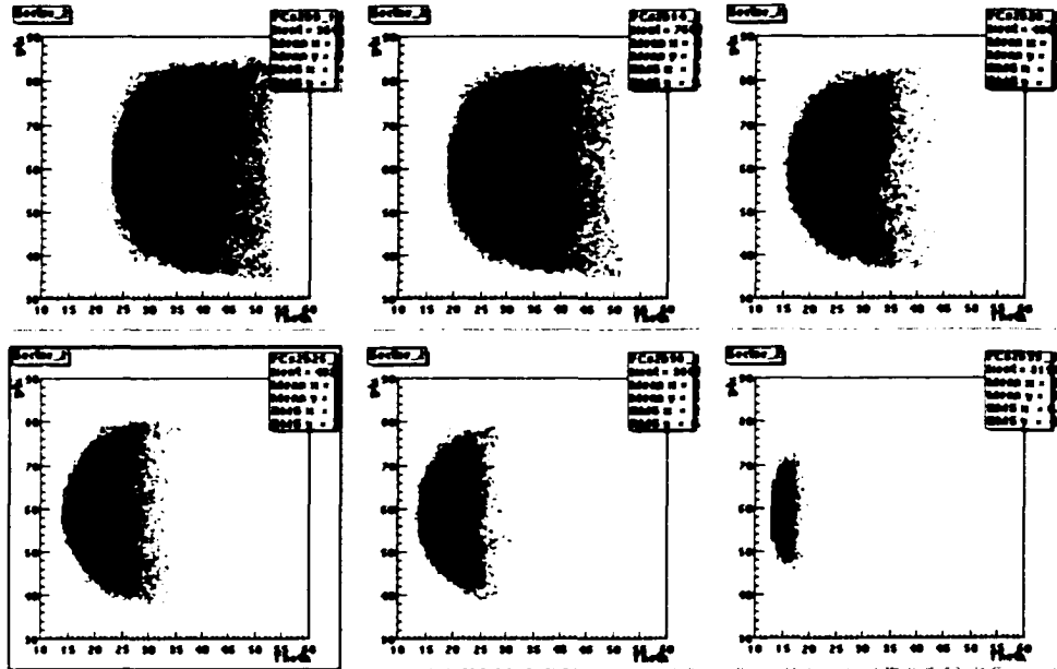
Figure B-6: Some typical plots of \phi(\theta) dependency. For the rest, please consult reference [102]
