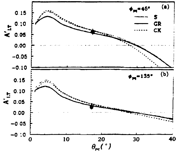
Figure 2-8: The A'_{LT} asymmetry for q = 0.35 GeV/c, \omega = 0.072 GeV ( Q^2 = 0.128 GeV ^2/c^2 ), for p-shell knockout on ^{12}\text{C} , measured at BATES by X.Jiang et al. [25]. The three curves correspond to different choices of optical potential (explained in the text).
