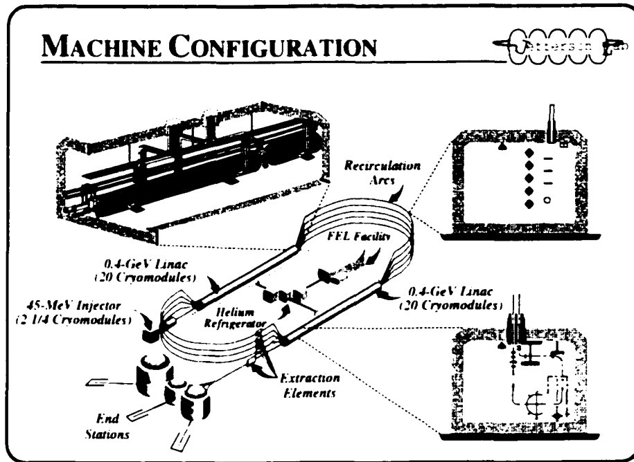
Figure 3-1: The CEBAF Accelerator. The three blowup boxes show (clockwise from upper l.h.s.): one of the linac cryomodules, a cross section of the tunnel with the five recirculating arcs, and a cross section of a cryomodule.
