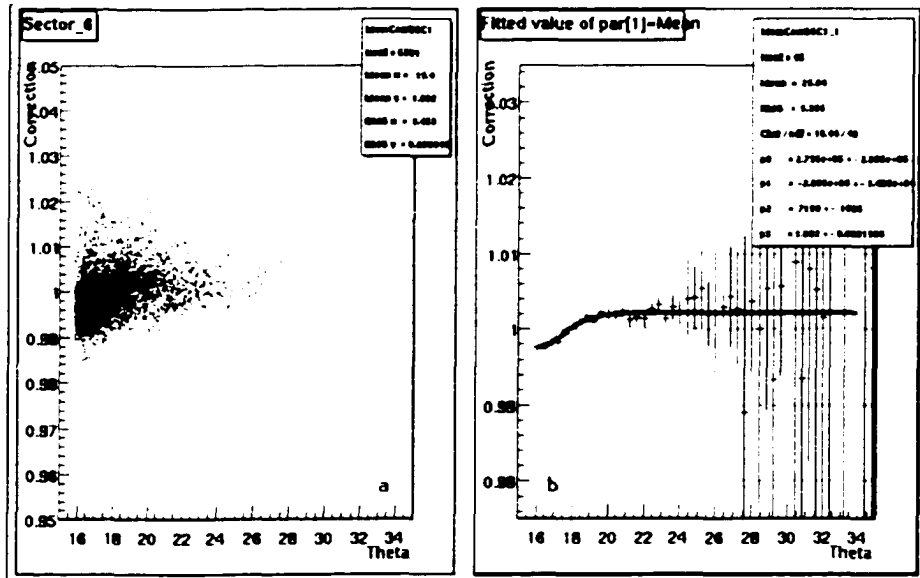
Figure A-6: Plot of the correction f_2 versus the angle \theta (left) and the fit with the function from eq.(A.7) (right). Only sector 6 is shown. For the others, please consult [104].
