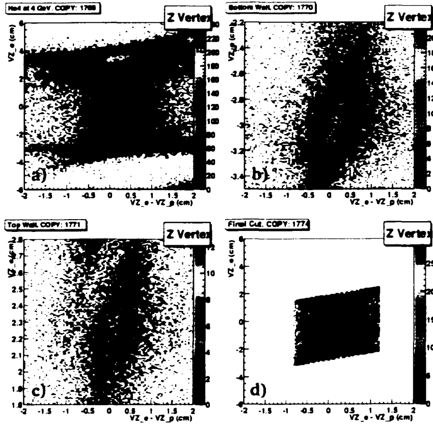
Figure 4-19: Liquid Target: the three visible bands in (a) are the thermal insulation and the target walls (in this order, from top to bottom). The position of the ridges in (b) and (c) is determined by a slice fit of the 2-d distributions. The cuts are positioned 3 mm inside the walls (d).
