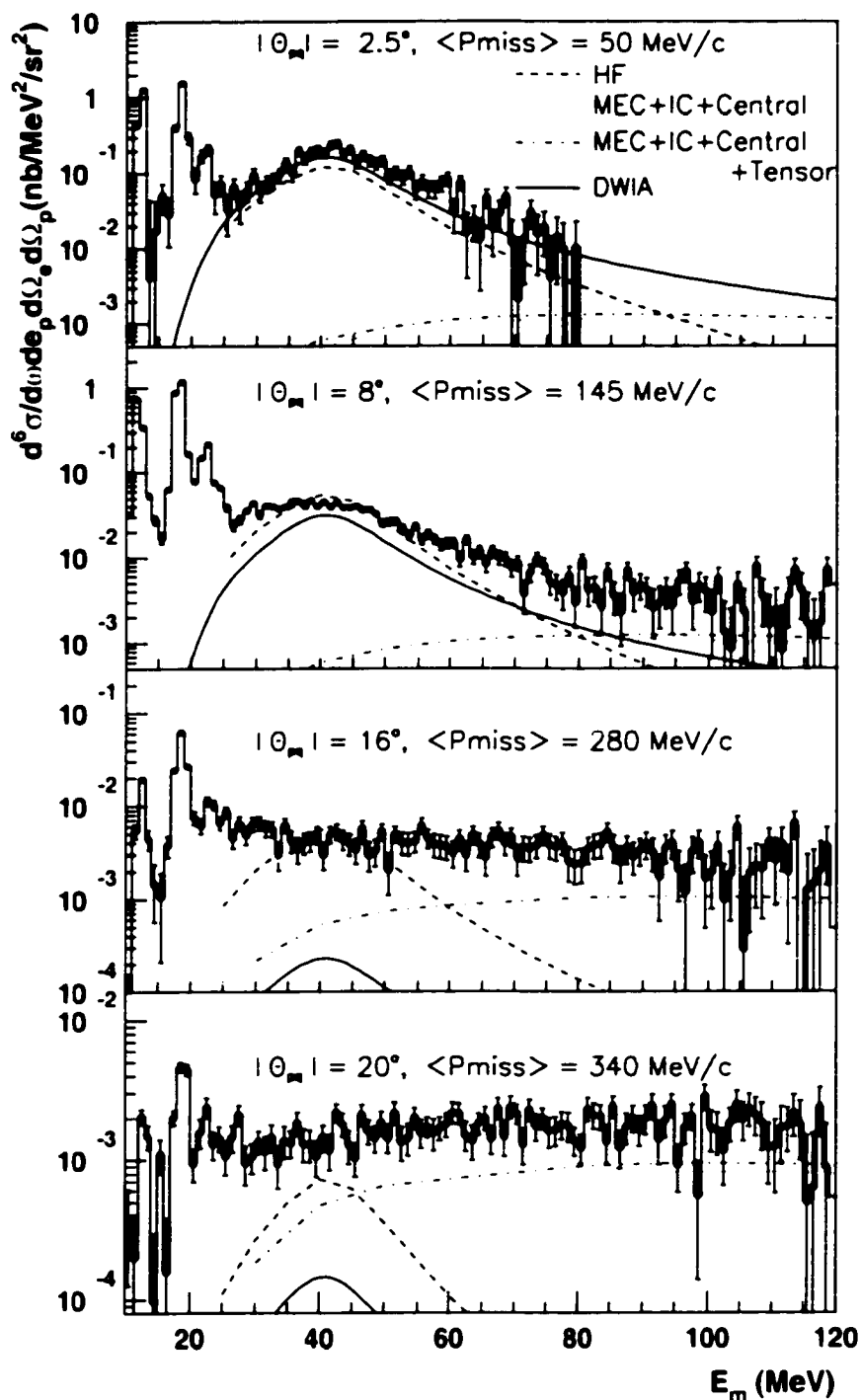
Figure 2-6: ^{16}\text{O}(e, e'p) cross-section measured at different outgoing proton angles as a function of missing energy from N. Liyanage et al. [51]. The curves show the single-particle strength calculated by J. Kelly ( s -shell only, solid curve) and by J. Ryckebusch (dashed curve), folded with the Lorentzian parameterization of Mahaux. The dotted line shows the Ryckebusch et al. calculations of the (e, e'pn) and (e, e'pp) contributions to (e, e'p) including MEC, IC and central correlations, while the dot-dashed line also includes tensor correlations. (from N. Liyanage et al. [51]).
