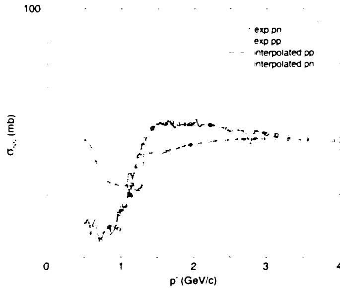
Figure D-1: Nucleon-nucleon scattering data: \sigma_{pN}^{tot} cross sections. Abscissa p' is the proton momentum. From [23].
