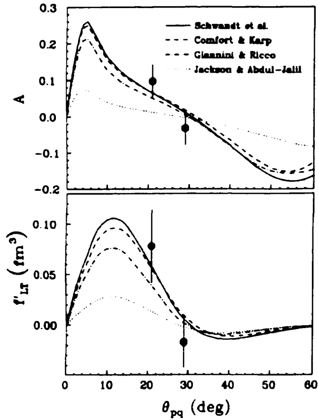
(b) The A'_{LT} and fifth response function f'_{LT} reported in [12].
