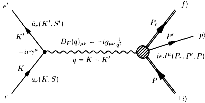
Figure 2-1: Lowest order graph for the exclusive ( e, e'p ) electron scattering process.
