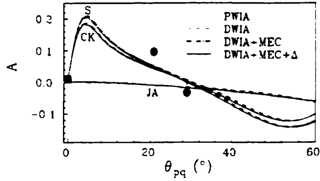
(a) The A'_{LT} asymmetry measurement reported in [24].
