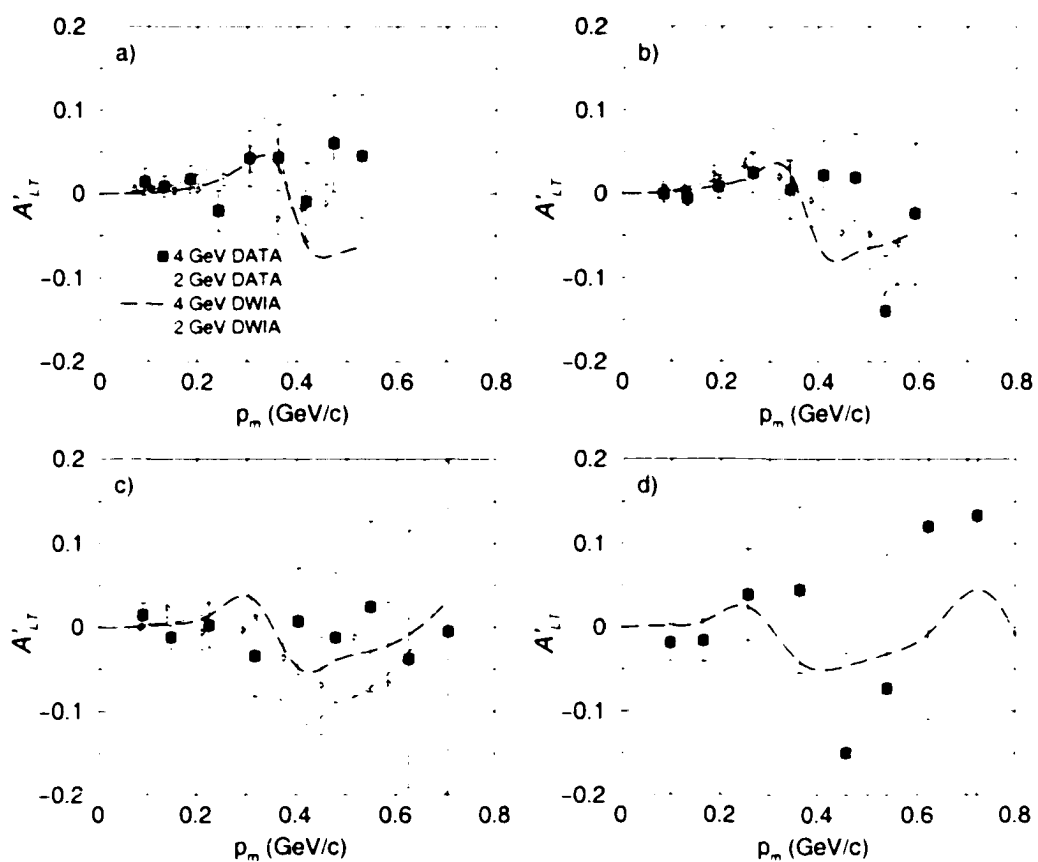
Figure 5-11: Consistency test between 2.262 and 4.462 GeV ^4\text{He} data: Q^2 bin n from 4.462 GeV (figure 5-10) is overlapped with bin n - 1 from 2.262 GeV ^4\text{He} (figure 5-9), where n = 2, 3, 4 , corresponding (in this order) to graphs (a), (b) and (c).
