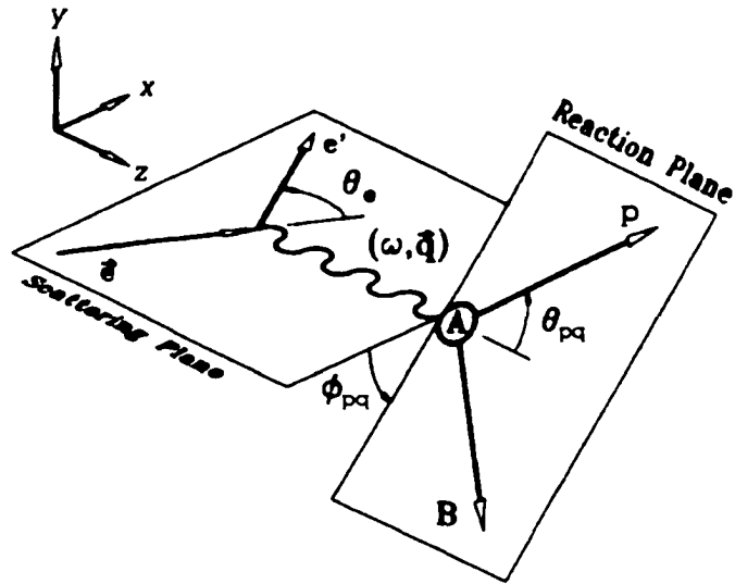
Figure 2-2: Kinematics for the semi-exclusive (\vec{e}, e'p) process. (figure from [12]).
