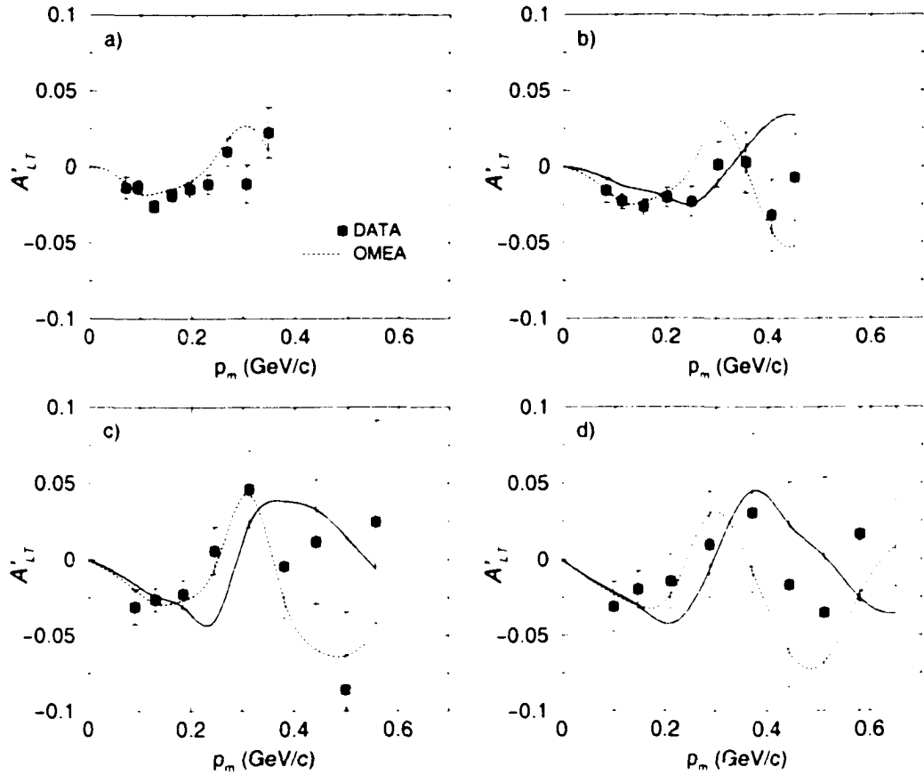
Figure 5-12: Dependence of A'_{LT} versus missing momentum p_m for ^{12}\text{C}(e, e'p) at 2.262 GeV, in four Q^2 bins along the quasielastic ridge. The Q^2 bins are set as follows: a) 0.350 < Q^2 \text{ (GeV}^2/c^2) < 0.712 , b) 0.712 < Q^2 \text{ (GeV}^2/c^2) < 1.075 , c) 1.075 < Q^2 \text{ (GeV}^2/c^2) < 1.438 and d) 1.438 < Q^2 \text{ (GeV}^2/c^2) < 1.800 . The solid (dotted) curves correspond to RMSGA (OMEA) calculations used as described in section 5.2. The data used are listed in table 5.5. Errors shown are statistical.
