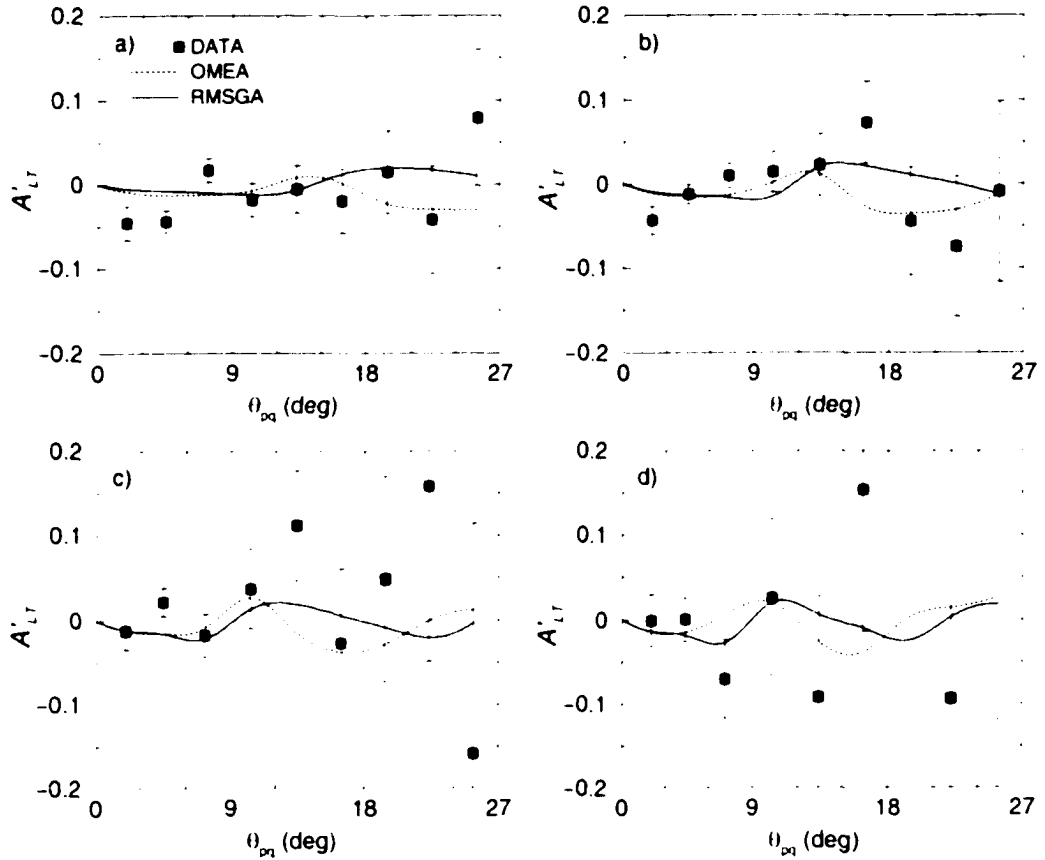
Figure 5-8: Dependence of A'_{LT} versus \theta_{pq} for ^{12}\text{C}(e, e'p) at 4.462 GeV. Measurements were done with an angle bin width of \Delta\theta_{pq} = 3' , for four Q^2 bins along the quasielastic ridge. The Q^2 bins are set as follows: a) 0.800 < Q^2 \text{ (GeV}^2/c^2) < 1.200 , b) 1.200 < Q^2 \text{ (GeV}^2/c^2) < 1.600 , c) 1.600 < Q^2 \text{ (GeV}^2/c^2) < 2.000 and d) 2.000 < Q^2 \text{ (GeV}^2/c^2) < 2.400 . There were no constraints on p_m or p' . The solid (dotted) curves correspond to RMSGA (OMEA) calculations used as described in section 5.2. The data are listed in table 5.6. Errors shown are statistical.
