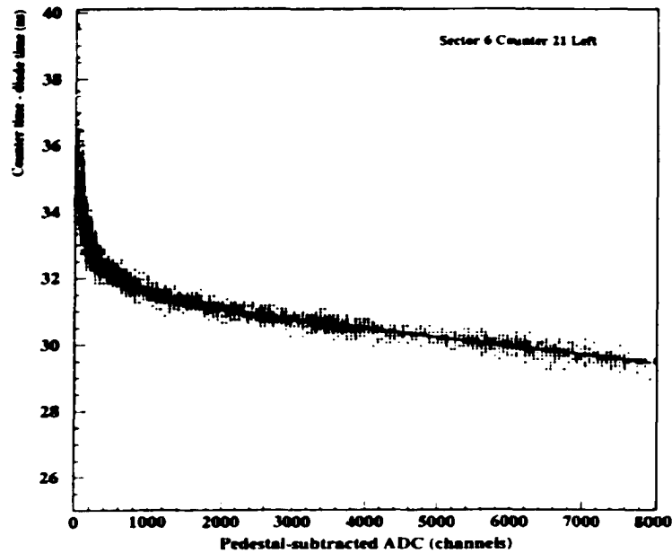
Figure 4-2: Typical dependence of the TDC times (ns) versus pulse height (ADC counts). The fit is done with with the function in eq.4.2. (from [63])
