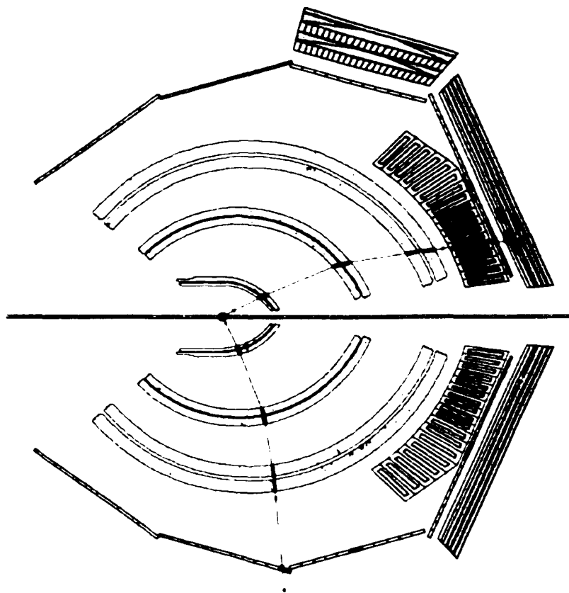
Figure 4-1: Snapshot of a CLAS Event Display (CED) screen to illustrate RECSIS track reconstruction. The display shows a cross-section through two diametrically opposite sectors of CLAS. The inbending track is the electron that gives the trigger. The outbending track corresponds to a positive particle.
