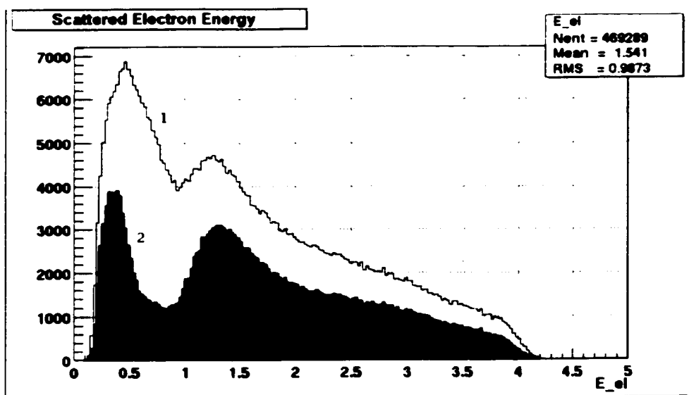
Figure B-5: Energy spectra of the electron before (1) and after (2) the forward calorimeter cut as given by equation (B.1). E_{e1} is in GeV.
