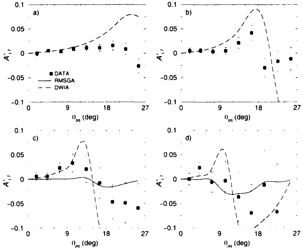
Figure 5-5: Dependence of A'_{LT} versus \theta_{pq} for {}^4\text{He}(e, e'p) at 2.262 GeV. Measurements were done with an angle bin width of \Delta\theta_{pq} = 3^\circ , for four Q^2 bins along the quasielastic ridge. The Q^2 bins are set as follows: a) 0.350 < Q^2 \text{ (GeV}^2/c^2) < 0.712 , b) 0.712 < Q^2 \text{ (GeV}^2/c^2) < 1.075 , c) 1.075 < Q^2 \text{ (GeV}^2/c^2) < 1.438 and d) 1.438 < Q^2 \text{ (GeV}^2/c^2) < 1.800 . There were no constraints on p_m or p' . The solid (dashed) curves correspond to RMSGA (DWIA) calculations used as described in section 5.2. The data are listed in table 5.3. Errors shown are statistical.
