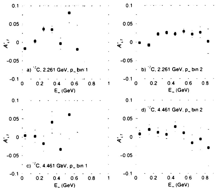
Figure 5-15: A'_{LT} versus E_m for carbon. The two missing momentum bins are defined as follows: 1) 0.0 < p_m < 0.2 and 2) 0.2 < p_m < 0.45 with p_m in \text{GeV}/c . No radiative corrections were applied. Errors shown are purely statistical.
