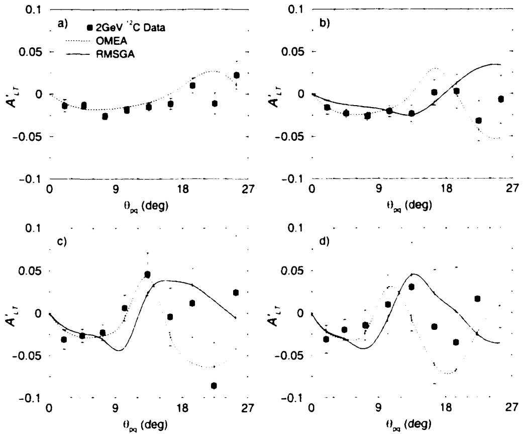
Figure 5-7: Dependence of A'_{LT} versus \theta_{pq} for ^{12}\text{C}(e, e'p) at 2.262 GeV. Measurements were done with an angle bin width of \Delta\theta_{pq} = 3^\circ , for four Q^2 bins along the quasielastic ridge. The Q^2 bins are set as follows: a) 0.350 < Q^2 \text{ (GeV}^2/c^2) < 0.712 , b) 0.712 < Q^2 \text{ (GeV}^2/c^2) < 1.075 , c) 1.075 < Q^2 \text{ (GeV}^2/c^2) < 1.438 and d) 1.438 < Q^2 \text{ (GeV}^2/c^2) < 1.800 . There were no constraints on p_m or p' . The solid (dotted) curves correspond to RMSGA (OMEA) calculations used as described in section 5.2. The data are listed in table 5.5. Errors shown are statistical.
