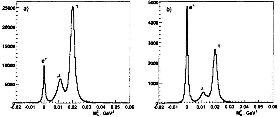
Figure 4-9: Mass squared for backward flying particles (paddles 20 and above) with momentum below 0.25 \text{ GeV}/c (a) without any sector cut (b) the electron and the other particle are required to be in the same sector (from [73] ).
