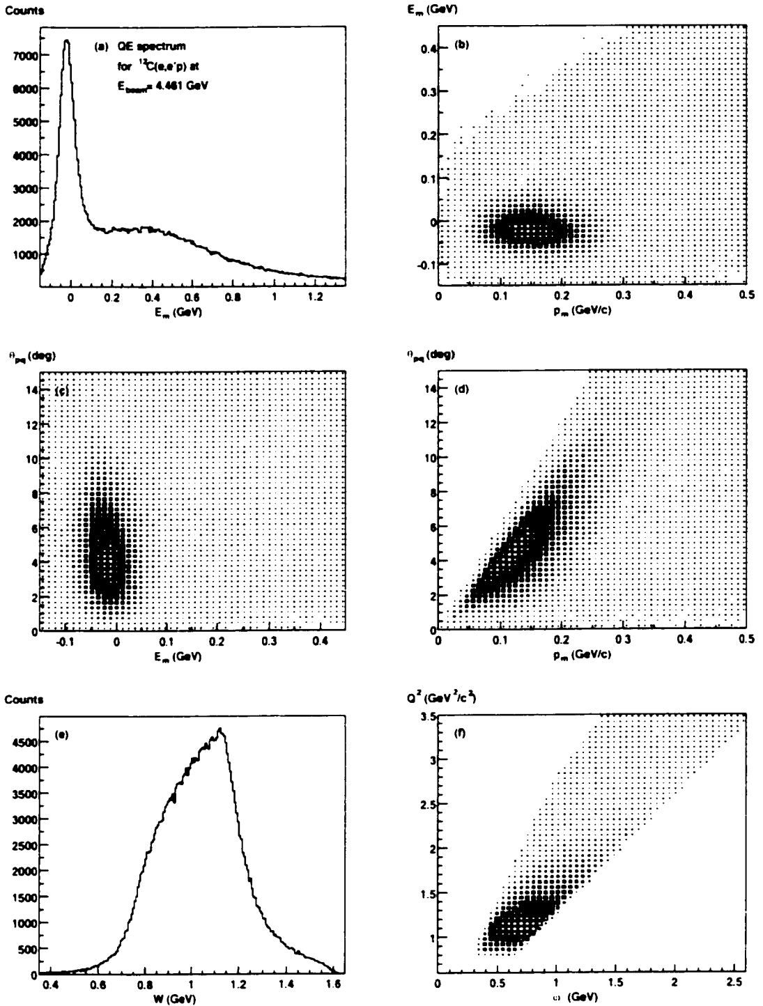
Figure 4-28: Quasielastic spectra for ^{12}\text{C}(e, e'p) at 4.461 GeV, obtained with eq.(4.18): (a) missing energy E_m , (b) missing energy vs. missing momentum p_m , (c) polar angle \theta_{pq} versus missing energy E_m , (d) polar angle \theta_{pq} versus missing momentum p_m , (e) invariant mass W for the (e, e'p) reaction and (f) Q^2 versus \omega cut. The E_m cut (4.19) is not shown. Compare to figure 4-24.
