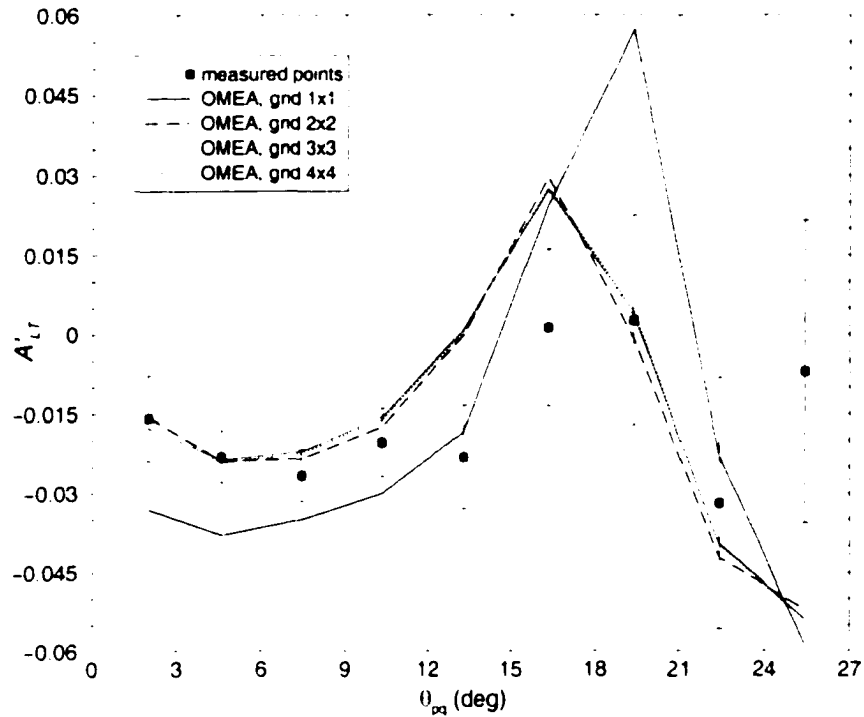
Figure 5-2: Convergence test on ^{12}\text{C} at 2.261 GeV, Q^2 bin A^2 . The theory calculation is done with OMEA, and the calculated points are linked by straight lines. Please refer to table 5.2.
