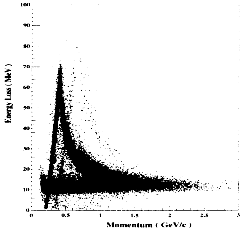
Figure 4-5: Energy loss in the scintillator material versus particle momenta. One can clearly distinguish the protons and pions and also a weak deuteron band.
