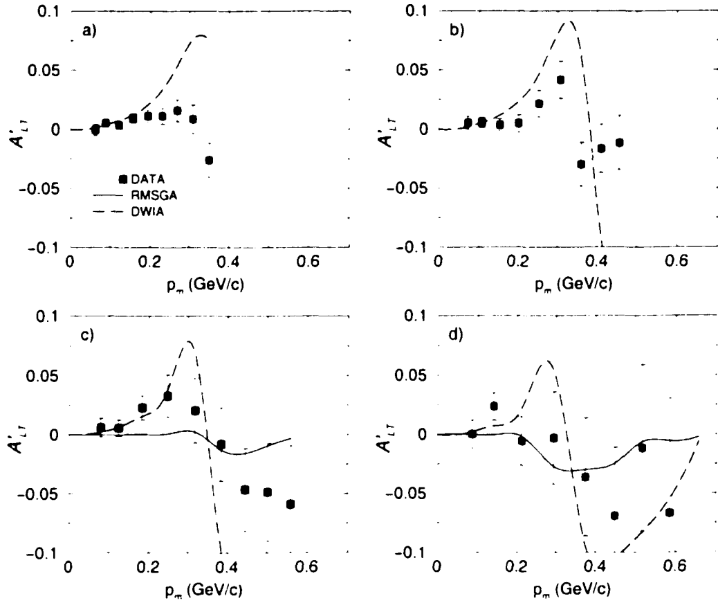
Figure 5-9: Dependence of A'_{LT} versus missing momentum p_m for {}^1\text{He}(e, e'p) at 2.262 GeV, in four Q^2 bins along the quasielastic ridge. The Q^2 bins are set as follows: a) 0.350 < Q^2 \text{ (GeV}^2/c^2) < 0.712 , b) 0.712 < Q^2 \text{ (GeV}^2/c^2) < 1.075 , c) 1.075 < Q^2 \text{ (GeV}^2/c^2) < 1.438 and d) 1.438 < Q^2 \text{ (GeV}^2/c^2) < 1.800 . The solid (dashed) curves correspond to RMSGA (DWIA) calculations used as described in section 5.2. The data used are listed in table 5.3. Errors shown are statistical.
