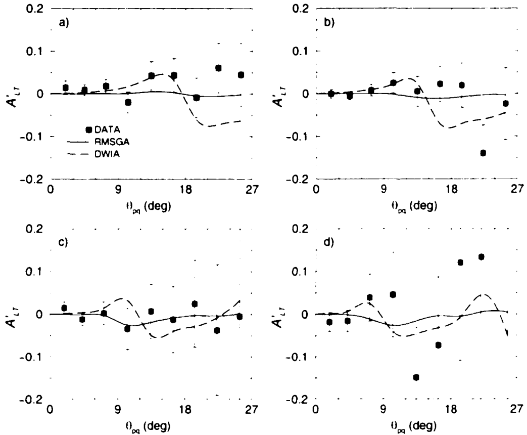
Figure 5-6: Dependence of A'_{LT} versus \theta_{pq} for {}^4\text{He}(e, e'p) at 4.462 GeV. Measurements were done with an angle bin width of \Delta\theta_{pq} = 3^\circ , for four Q^2 bins along the quasielastic ridge. The Q^2 bins are set as follows: a) 0.800 < Q^2 \text{ (GeV}^2/c^2) < 1.200 , b) 1.200 < Q^2 \text{ (GeV}^2/c^2) < 1.600 , c) 1.600 < Q^2 \text{ (GeV}^2/c^2) < 2.000 and d) 2.000 < Q^2 \text{ (GeV}^2/c^2) < 2.400 . There were no constraints on p_m or p' . The solid (dashed) curves correspond to RMSGA (DWIA) calculations used as described in section 5.2. The data are listed in table 5.4. Errors shown are statistical.
