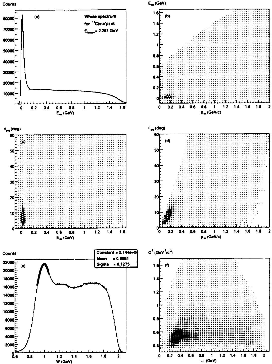
Figure 4-23: Accessible spectra for ^{12}\text{C}(e,e'p) at 2.261 GeV beam energy: (a) missing energy E_m , (b) missing energy vs. missing momentum p_m , (c) polar angle \theta_{pq} versus missing energy E_m , (d) polar angle \theta_{pq} versus missing momentum p_m , (e) invariant mass W for the (e,e'p) reaction and (f) Q^2 versus \omega distribution.
