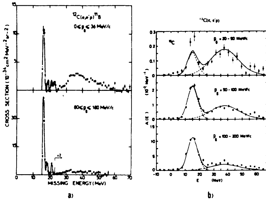
Figure 2-4: Missing energy spectra for the ^{12}\text{C}(e, e'p)^{11}\text{B} reaction, within different missing momentum ( p_B ) bins: (a) from J. Mougey et al. [4] (1976). (b) from K. Nakamura et al. [3] (1976). The data is well reproduced by DWIA.
