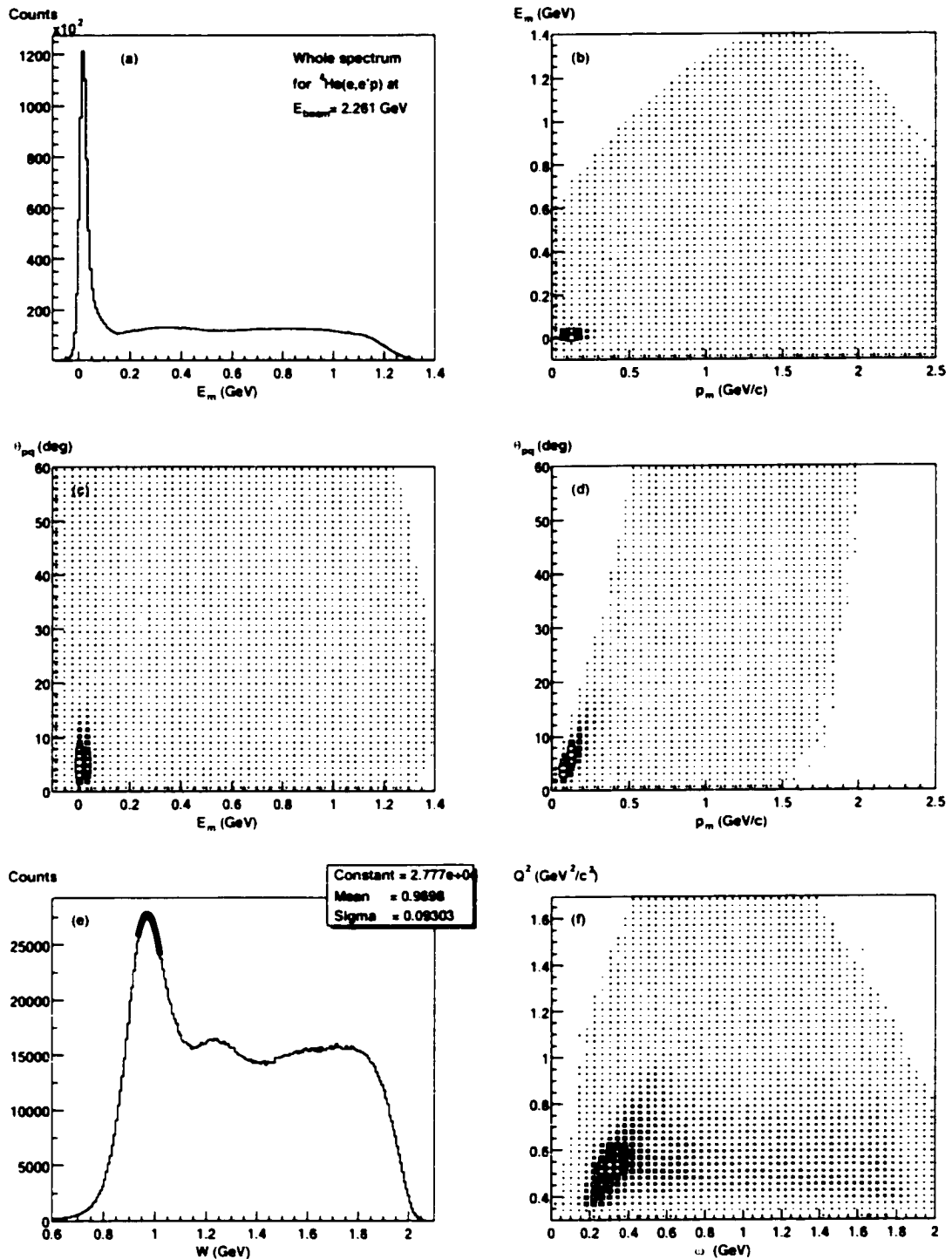
Figure 4-21: Accessible spectra for {}^4\text{He}(e, e'p) at 2.261 GeV beam energy: (a) missing energy E_m , (b) missing energy vs. missing momentum p_m , (c) polar angle \theta_{pq} versus missing energy E_m , (d) polar angle \theta_{pq} versus missing momentum p_m , (e) invariant mass W for the (e, e'p) reaction and (f) Q^2 versus \omega distribution.
