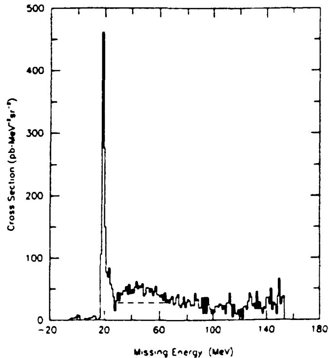
Figure 2-5: Missing energy spectra for ^{12}\text{C}(e, e'p) at quasielastic kinematics from R. Lourie et al. [8]. The area above the dashed line is attributed to the s -shell.
