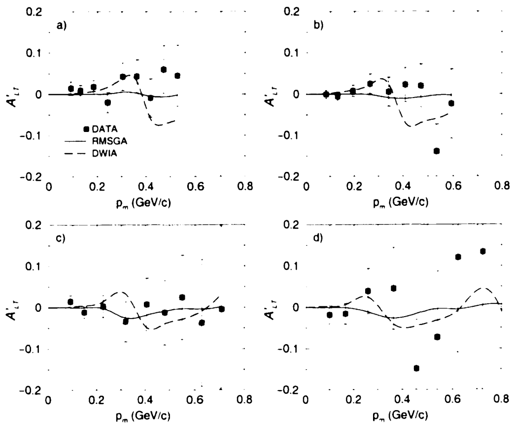
Figure 5-10: Dependence of A'_{LT} versus missing momentum p_m for {}^4\text{He}(e, e'p) at 4.462 GeV, in four Q^2 bins along the quasielastic ridge. The Q^2 bins are set as follows: a) 0.800 < Q^2 ( \text{GeV}^2/c^2 ) < 1.200 , b) 1.200 < Q^2 ( \text{GeV}^2/c^2 ) < 1.600 , c) 1.600 < Q^2 ( \text{GeV}^2/c^2 ) < 2.000 and d) 2.000 < Q^2 ( \text{GeV}^2/c^2 ) < 2.400 . The solid (dashed) curves correspond to RMSGA (DWIA) calculations used as described in section 5.2. The data used are listed in table 5.4. Errors shown are statistical.
