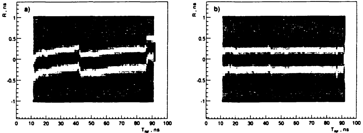
Figure 4-7: Two dimensional plot showing versus T_{RF} for (a) uncalibrated RF-signal and (b) calibrated RF-signal (figure courtesy of H. Egiyan [73]).
