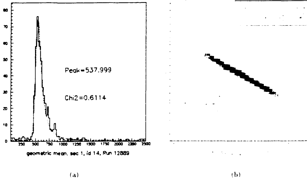
Figure 4-4: Monitoring histogram showing (a) the fit to the geometric mean of the energy loss for MIP-s in the counter and (b) correctly calibrated attenuation length and energy loss. (from [63]).
