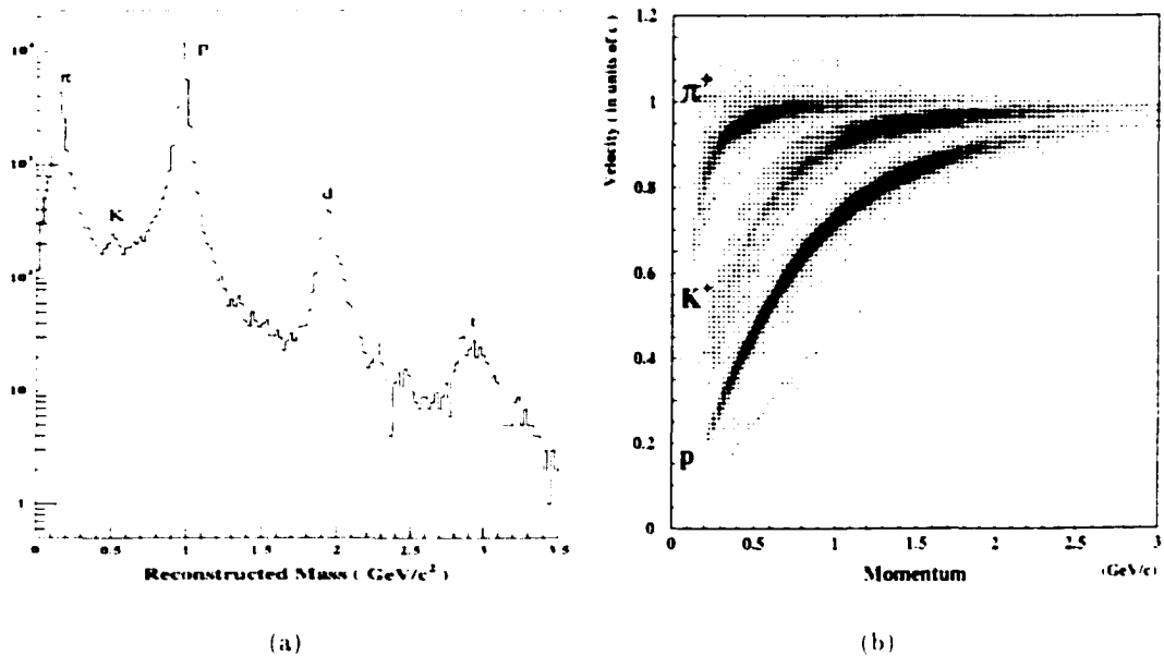
Figure 4-8: (a) Mass spectrum of hadrons from an empty target run. (b) Plot of \beta versus momentum. Here the kaon band was artificially enhanced. The pion and proton bands are reliably separated up to 2.5 GeV/c momenta (from [73]).
