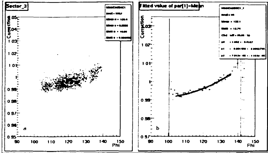
Figure A-5: Plots of the correction f_1 versus the angle \phi for \theta > 16^\circ : a 2D Histogram (left) is sliced and fitted (right). Only sector 3 is shown. For the other five plots, please see [104]
