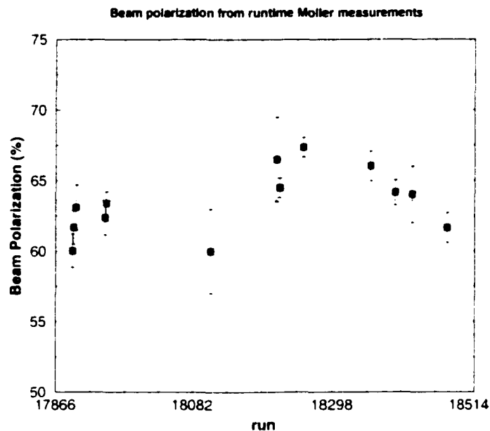
Figure 3-8: The electron beam polarization during the E2A run period as obtained from online analysis of the Moller measurements. The dotted line corresponds to the mean value.
