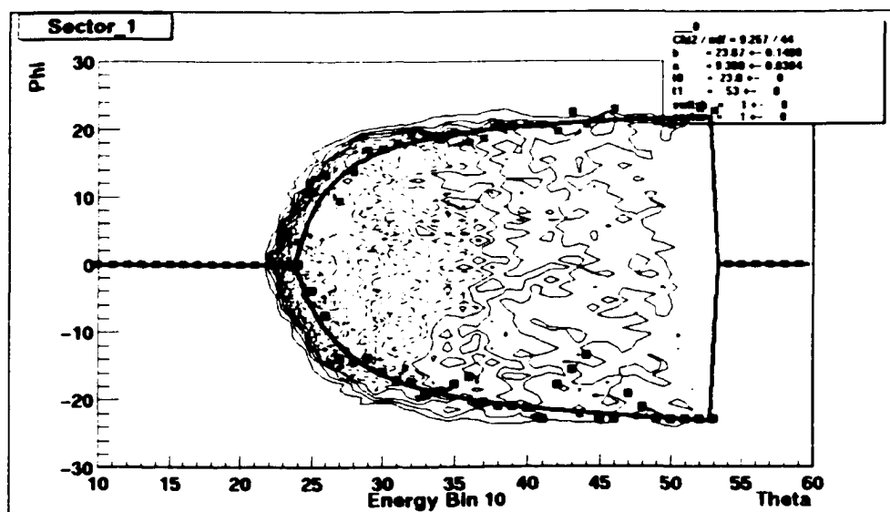
Figure B-9: Second generation fit. Energy bin 10 means 1.0 \text{ GeV} < p_{t1} < 1.1 \text{ GeV} . All other plots can be found in [102].
