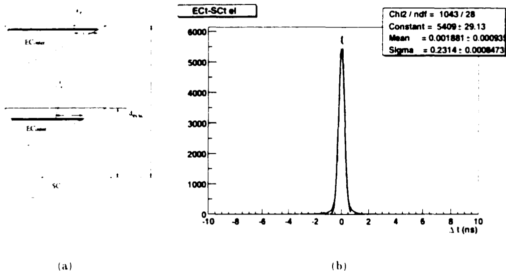
Figure 4-10: (a) EC time extrapolation from SC time. Only the scintillation bar with the largest ADC value in one view for each EC layer is shown. (b) Obtained EC time resolution for electrons in sector 1 (from [70]).
