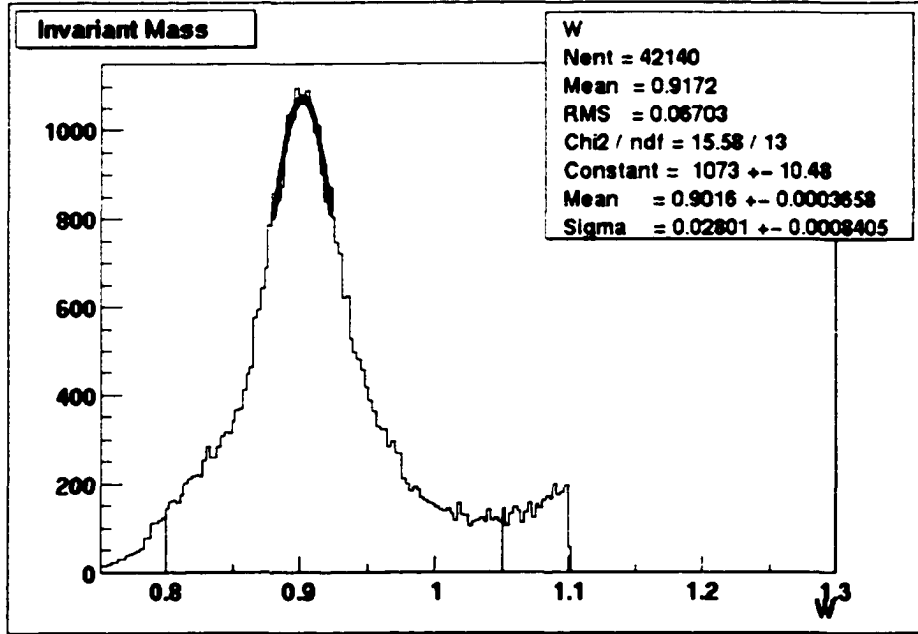
Figure A-2: The elastic peak in W before applying any corrections. All sectors together.
