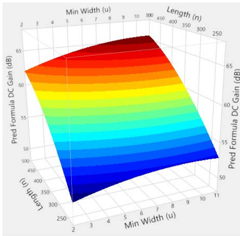
Fig. 3.3. Response surface analyzing minimum width, length, and prediction formula for DC gain of indirect feedback amplifier.
