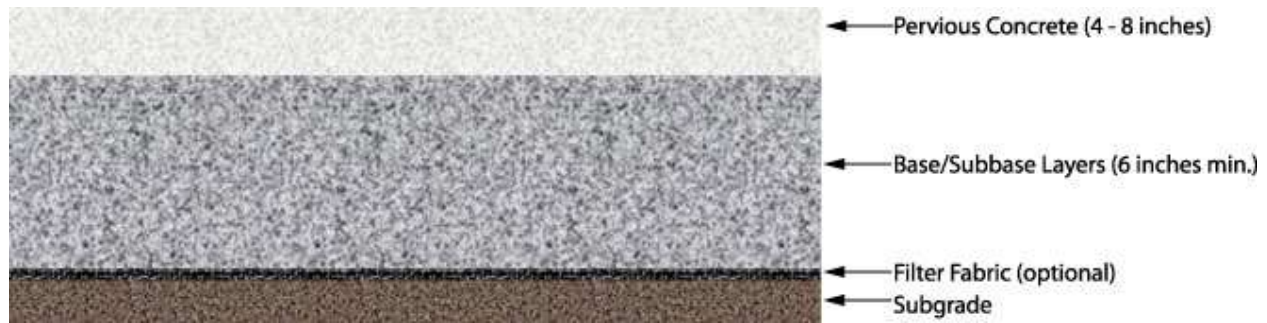
Figure 1. Pervious Concrete Pavement Structure Components (from FHWA TechBrief: Pervious Concrete, December 2012)
