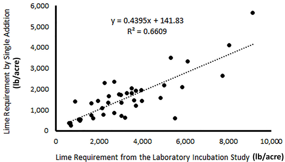
Fig. 2. Relationship between the amount of \text{CaCO}_3 required to raise the soil \text{pH}_{w1:2} to 6.0 as determined by a 90-day laboratory incubation study and the single addition of \text{Ca(OH)}_2 for 40 soils from across Arkansas.
