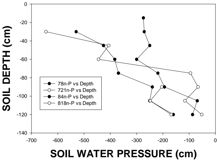
Fig. 21. Soil water pressure in the Sharkey profile at four dates during the growing season.
