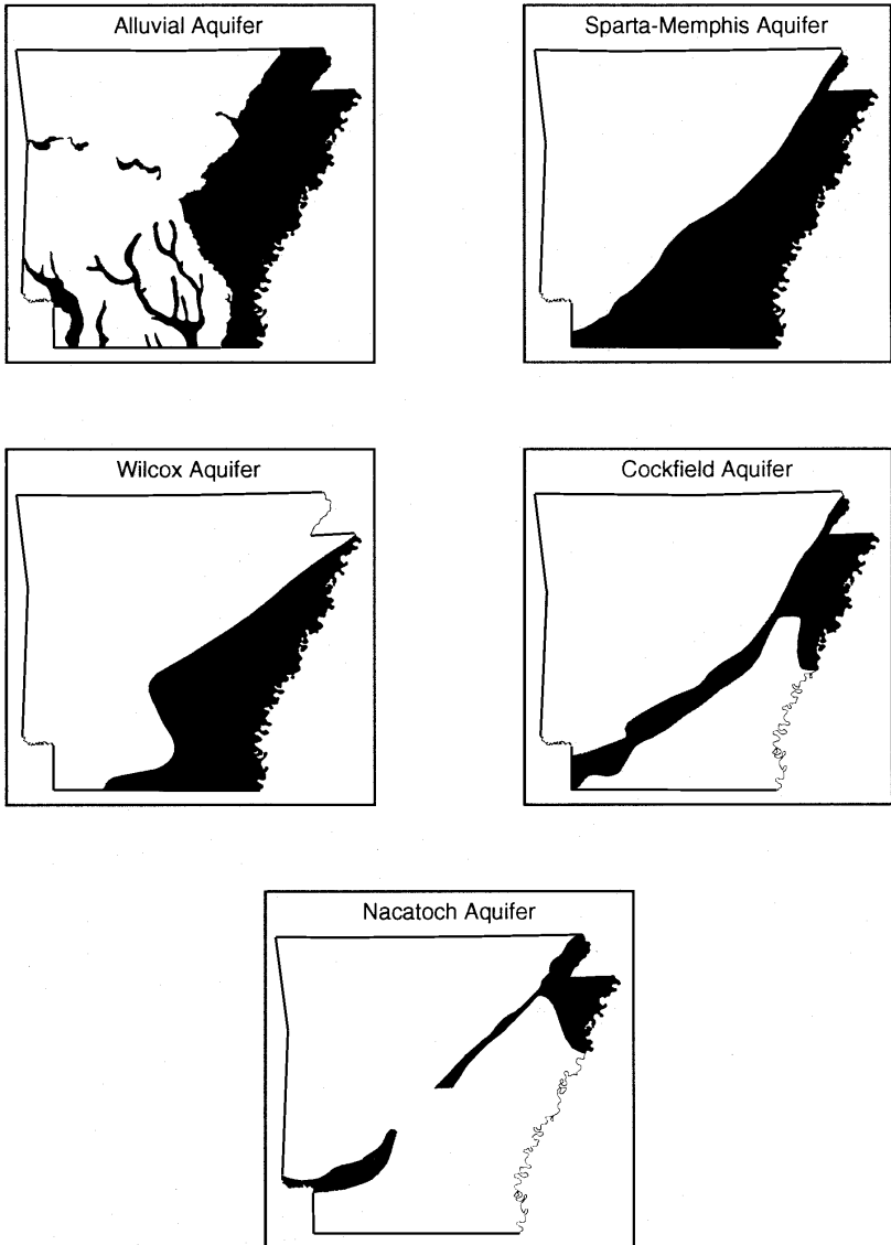
Fig. 6. Areal extent of selected aquifers in Arkansas.
