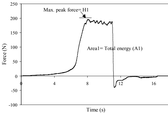
Fig. 4. Typical force-time extrusion curve (Test IV).
