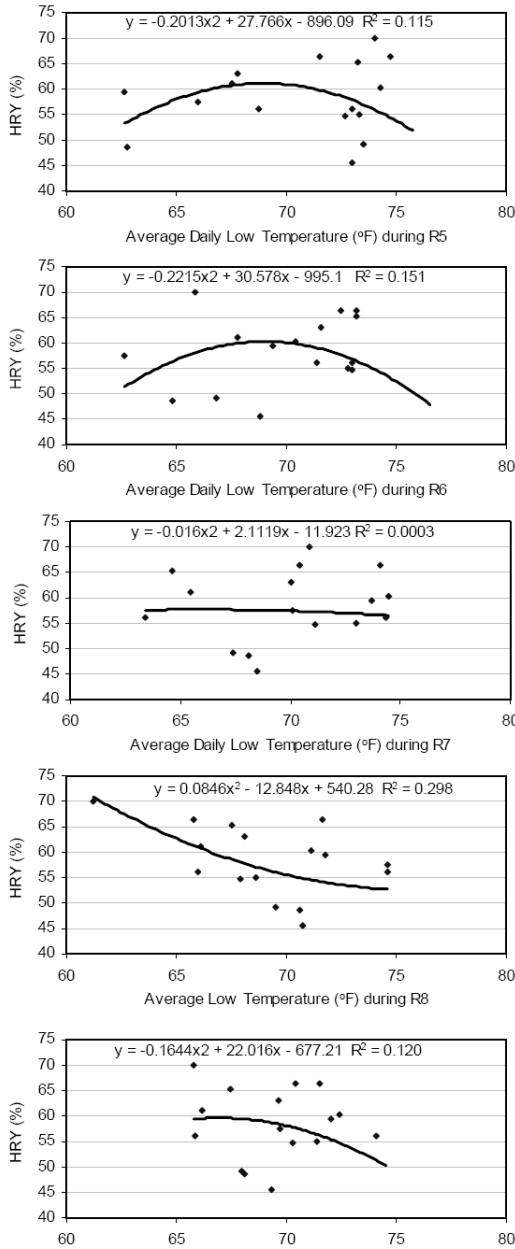
Fig. 3. Historical head rice yield (HRY) of Lemont rice from Stuttgart, Ark., 1983-1999, related to the average low (or nighttime) temperatures at the indicated stages of rice development,
