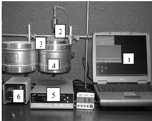
Fig. 1. Miniature/precision rice cooker. 1. Computer with temperature controller software. 2. Thermocouple. 3. Glass bowl. 4. Heating mantle. 5. Temperature controller. 6. Temperature controller set at 60°C.
