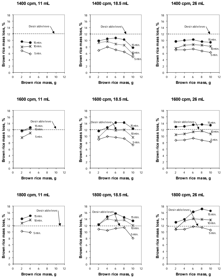
Fig. 2. Francis brown rice mass loss percentage after milling using the Genogrinder 2000 at various oscillation speeds, milling durations, and tube sizes for different amounts of brown rice at 12% MC. Note that for the 11 mL tube, only 2 and 4 g brown rice samples were run due to space limitation. Each data point is the average of two replications.
