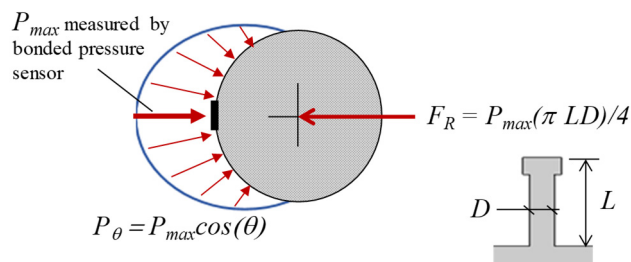
Figure 3. Pressure distribution on a cylinder embedded within a solid (negligible tolerance) [6, 7]
