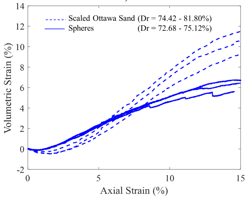
Figure 16: Triaxial shear behavior of scaled Ottawa sand and spheres with medium (10.16 cm diameter): a) principal stress difference b) volumetric strain.
