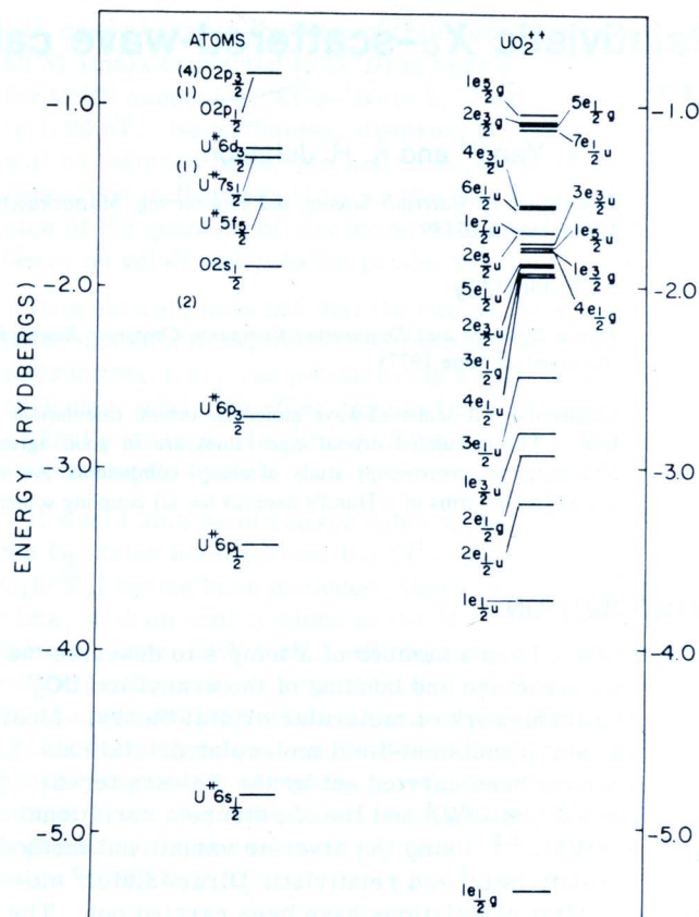
FIG. 1. Relativistic X\alpha -SW orbital energies for \text{UO}_2^{++} , \text{U}^{++} , and O.
