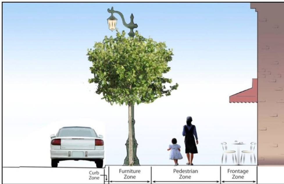
Figure 34. Sidewalk Zones
