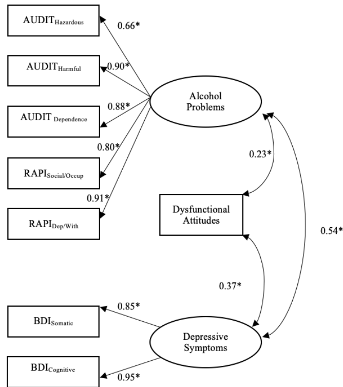
Figure 4. The final measurement model for the community sample, time 1 data used.
