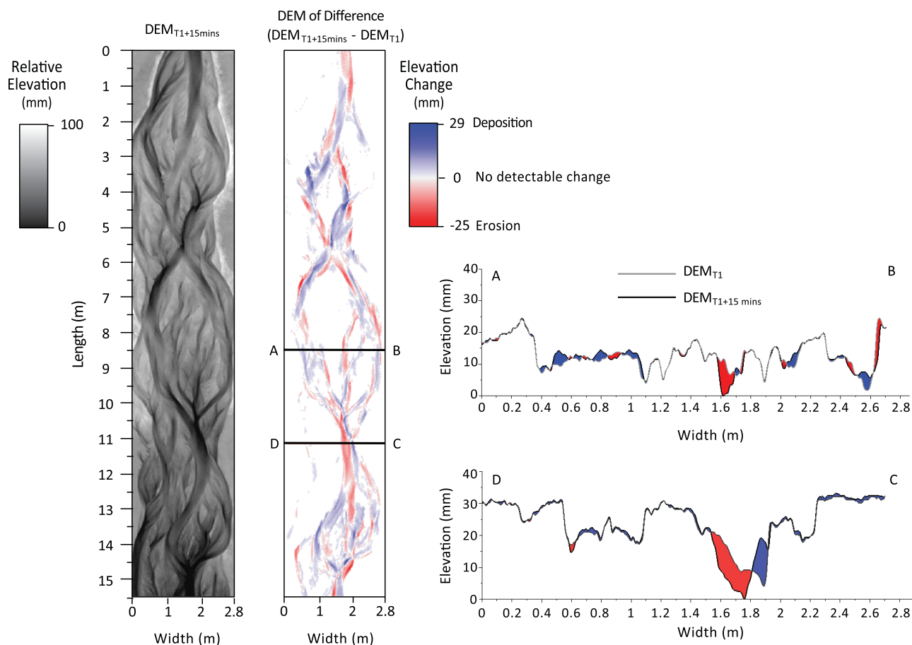
Figure 1. (left) Digital elevation models from a Froude-scaled physical model of a braiding channel were used to generate (middle) DEMs of difference (DoD) by comparing the elevation differences between DEMs over time. (right) The planform view of the DoDs demonstrate differences in the morphological active width spatially, while the cross sections illustrate some of the variability in the morphological active depth at a given time step.
