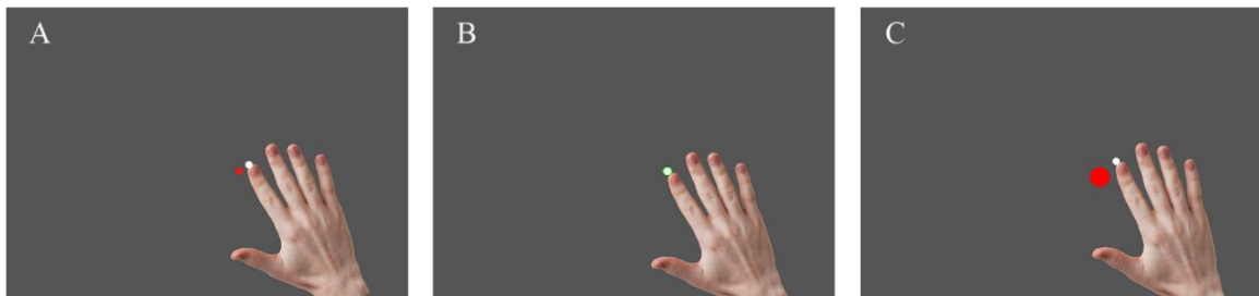
Figure 9. Perturbation-Calibration trial. A) Participant had to move his index finger tip's indicator (white circle) to the home location (red circle). B) Staying in the home location turned home location color into green. C) After a random period, an extension perturbation displaced the index finger tip's indicator from home location and the home location was turned into a larger red circle.
