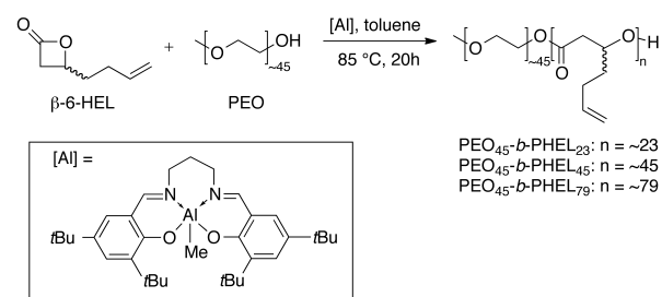
Scheme 1. Synthesis of PEO- b -PHEL block copolymers.
