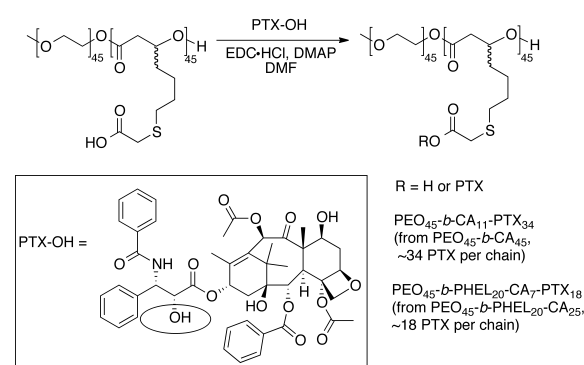
Scheme 3. Synthesis of the PTX conjugates PEO 45 -b-CA 11 -PTX 34 and PEO 45 -b-PHEL 20 -CA 7 -PTX 18 . The site of conjugation on PTX is circled.
