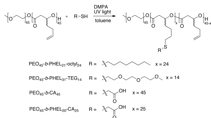
Scheme 2. Functionalization of PEO _{45} - b -PHEL _{45} with octyl chains, TEG, and carboxylic acids.
