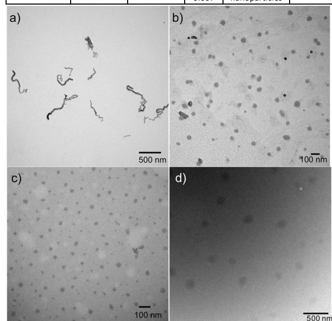
Fig. 3. TEM images of assemblies formed from: a) PEO 45 - b -PHEL 21 -octyl 24 ; b) PEO 45 - b -PHEL 31 -TEG 14 ; c) PEO 45 - b -PHEL 20 -CA 25 ; d) PEO 45 - b -PHEL 40 -RHD 5 using the THF/water solvent exchange method.
