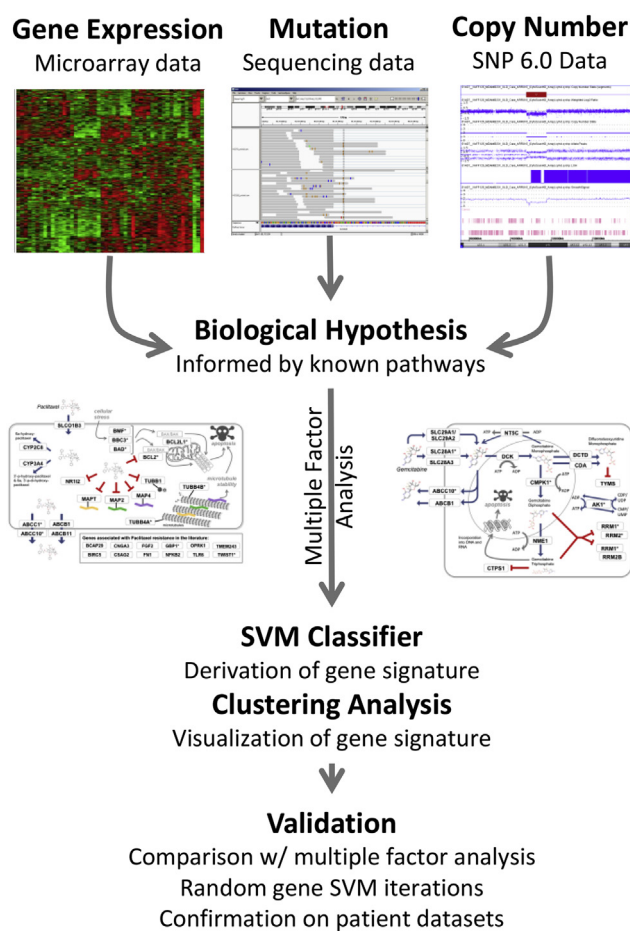
Figure 1 – Workflow to derive gene signatures. Gene sets were derived for paclitaxel and gemcitabine based on known drug pathways, metabolism, and genes previously implicated in resistance. A multiple factor analysis was completed for each gene to determine which data types (gene expression, copy number, and mutation data) were correlated with the growth inhibitory values for paclitaxel and gemcitabine. Gene expression values were used to derive the paclitaxel SVM classifier, and both gene expression and copy number were used for the gemcitabine SVM. Cell lines were then clustered on optimized gene sets to visualize stratification of tumor subtype and sensitivity. The SVM classifiers were validated using random gene iterations to determine the significance of the classification accuracy, and patient data sets to ensure robustness of the models derived.
