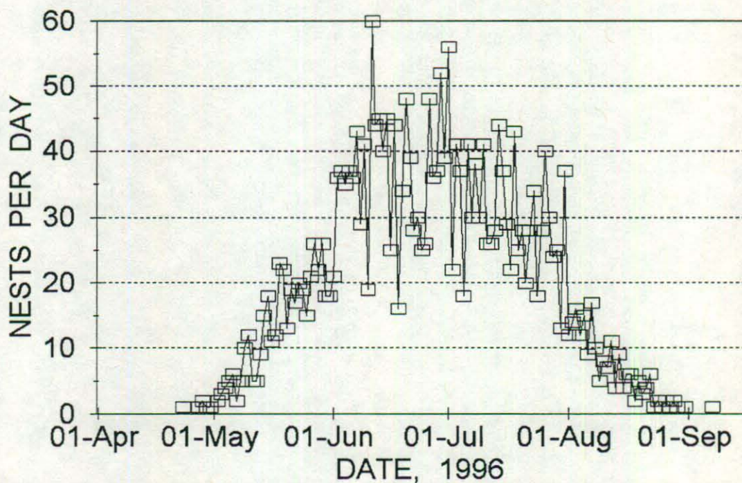
Figure 3: The seasonal pattern of daily loggerhead nesting in Broward County, 1996.
