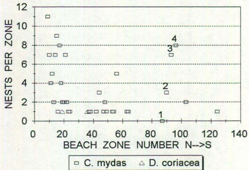
Figure 7: Locations of loggerhead, green and leatherback nests in Broward County, 1996. Numbers 1-4 indicate the four beach zones of John Lloyd Park.
