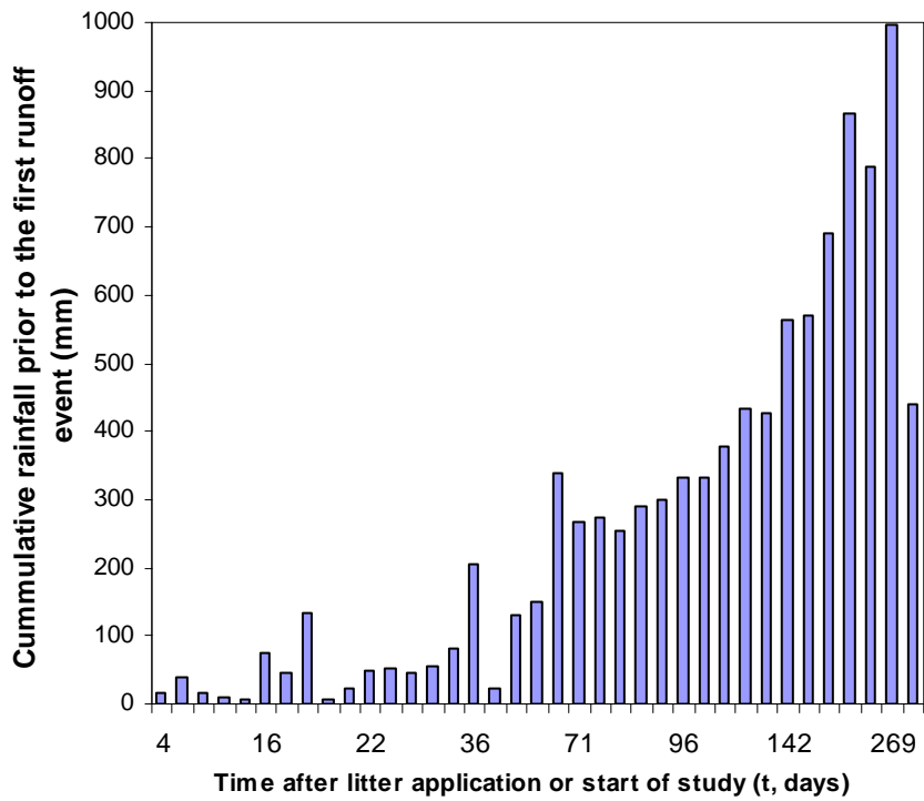
Figure 4-8. Cumulative precipitation prior to runoff event vs. days after litter application for the summarized projects.
